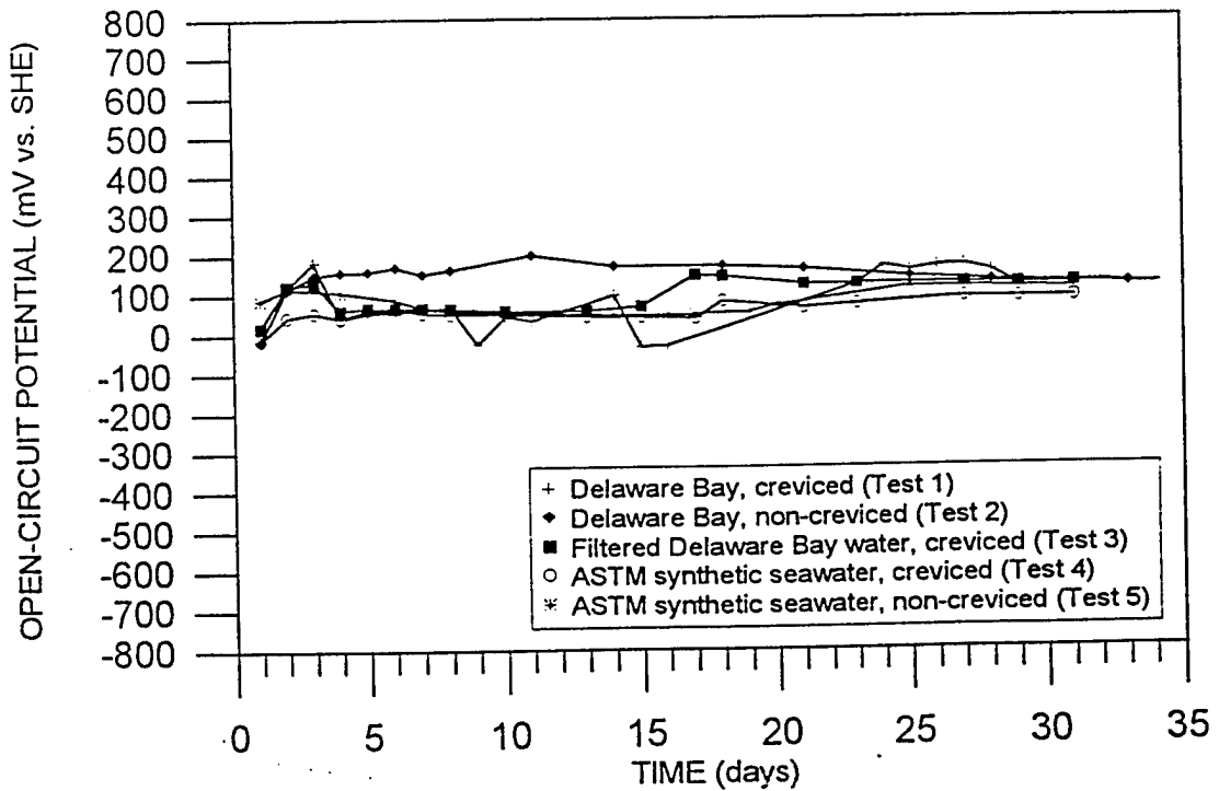
Figure 10. Open-circuit potential vs. time for weldment #1-b (304L/308L, brushed).
