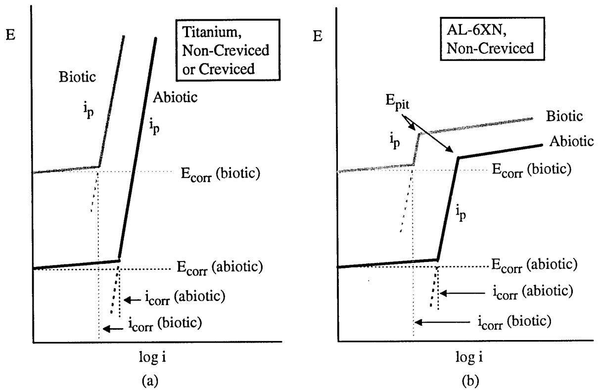
Figure 42. Schematic, proposed anodic polarization behaviors in abiotic and biotic environments for (a) non-creviced and creviced Ti weldments, and (b) non-creviced AL-6XN weldments.
