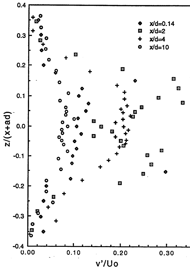
Figure 46a. v'/U_0 versus z^* in the deep mode for S = 0.265 at various axial distances
