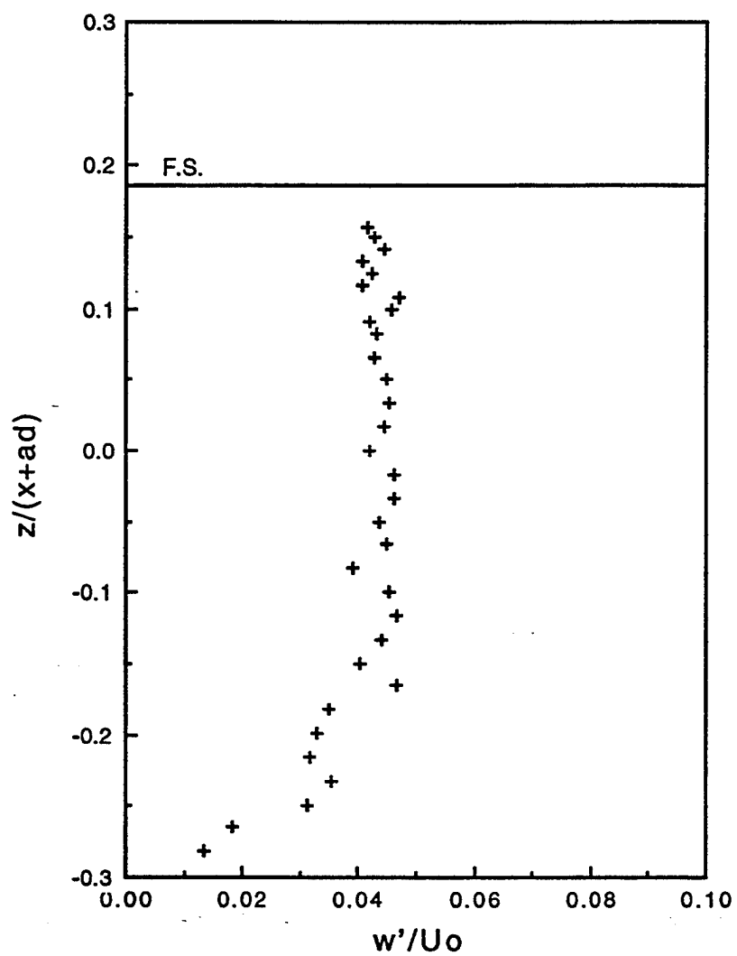
Figure 86. w'/U_o versus z^* in the shallow mode for S = 0.522 at x/d = 16
