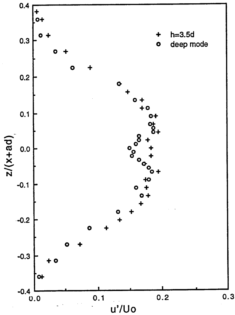
Figure 22. u'/U_o versus z^* in the deep and shallow modes for S = 0.265 at x/d = 4
