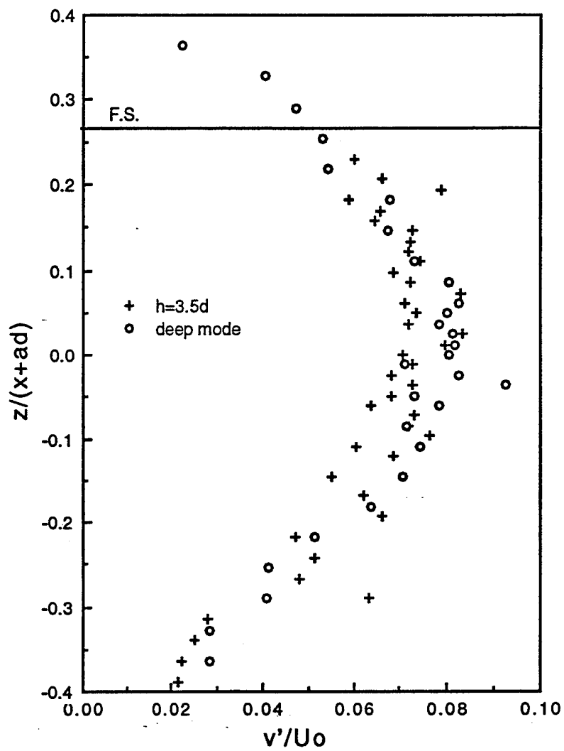
Figure 75. v'/U_0 versus z^* in the deep and shallow modes for S = 0.522 at x/d = 10
