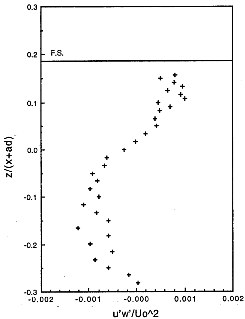
Figure 89. u'w'/U_o^2 versus z^* in the shallow mode for S = 0.522 at x/d = 16
