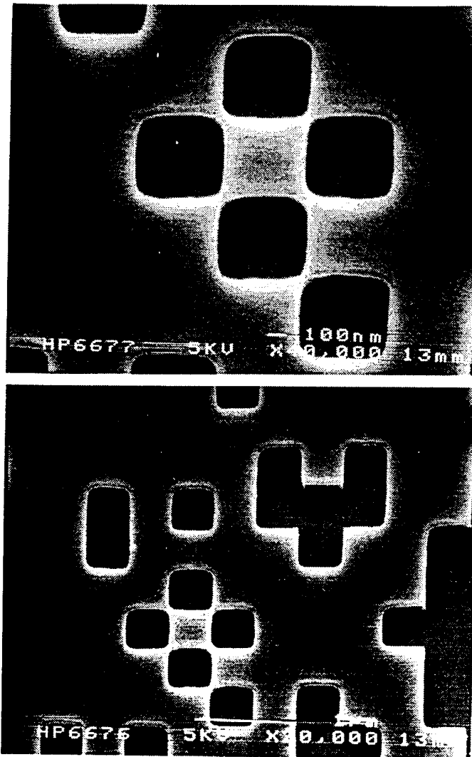
cd Figure 15: SEM micrographs of halftoned masks made at HP ULSI Research Laboratories, Palo Alto, CA.
