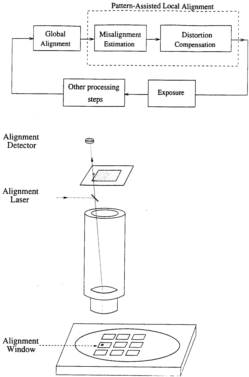
Figure 10: Schematic of pattern-assisted alignment scheme
