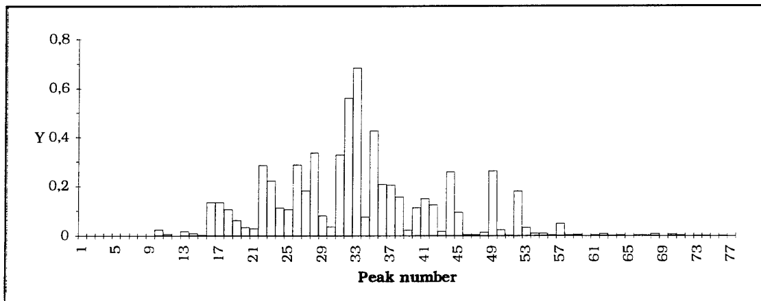
Fig.9 Arochlor 1248 degradation patterns of strains ENV360 and ENV391 with and without addition of glucose lipid MM1
