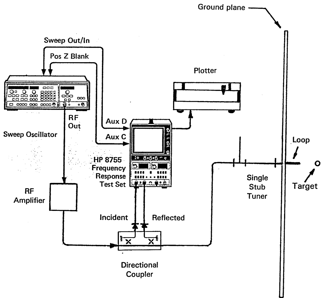
Figure 26. Measurement configuration for single stub tuned loop with high power input.
