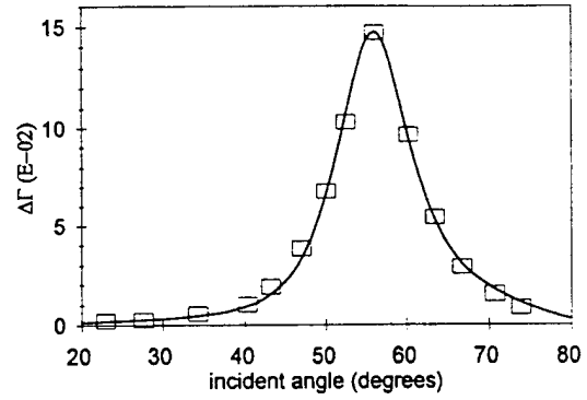
FIG. 6. Incident angle dependence of the field-induced phase retardation under voltage of -8.0 V for the PLZT thin-film sample measured in Fig. 5. The discrete points are experimental data. The solid line is the theoretical curve from least-squares fitting Eq. (13) to the experimental data.
