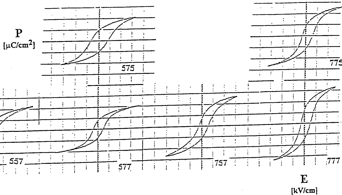
Figure 7. Ac hysteresis loops of PLZT 9/65/35 thin films with various firing schedules. Vertical scale = 15 \mu\text{C}/\text{cm}^2 per div. Horizontal scale = 50 \text{kV}/\text{cm} per div.
