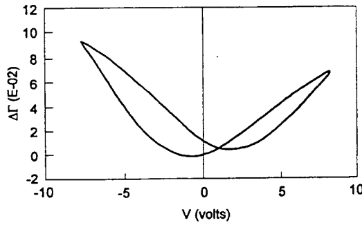
FIG. 5. Field-induced phase retardation vs electric-field loop for a 8/65/35 PLZT thin film sputter deposited on a Pt-coated silicon substrate.
