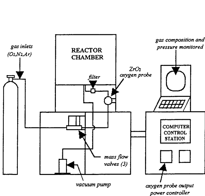
ATMOSPHERE CONTROL SYSTEM
