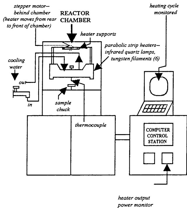
RAPID THERMAL PROCESSING UNIT
