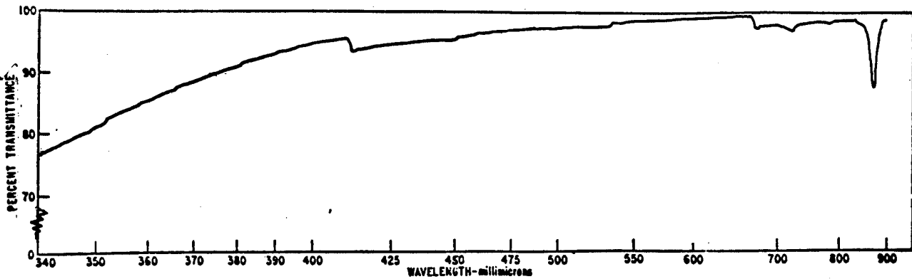
RTV 602 Transmission Data - Cured Section (4)
