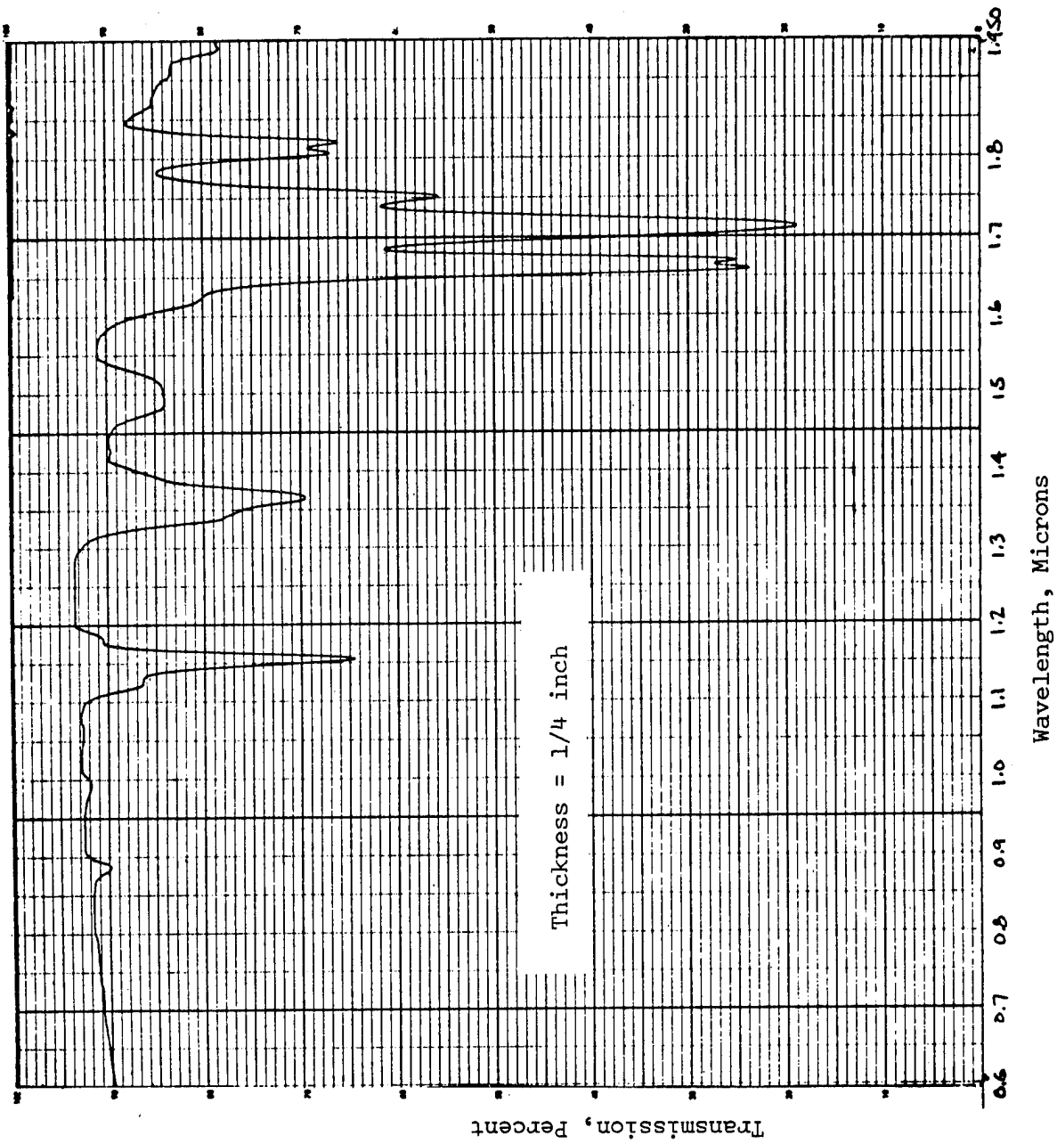
Optical Transmission Curve - Heat Aged XR-63-489 Adhesive Only (2)
