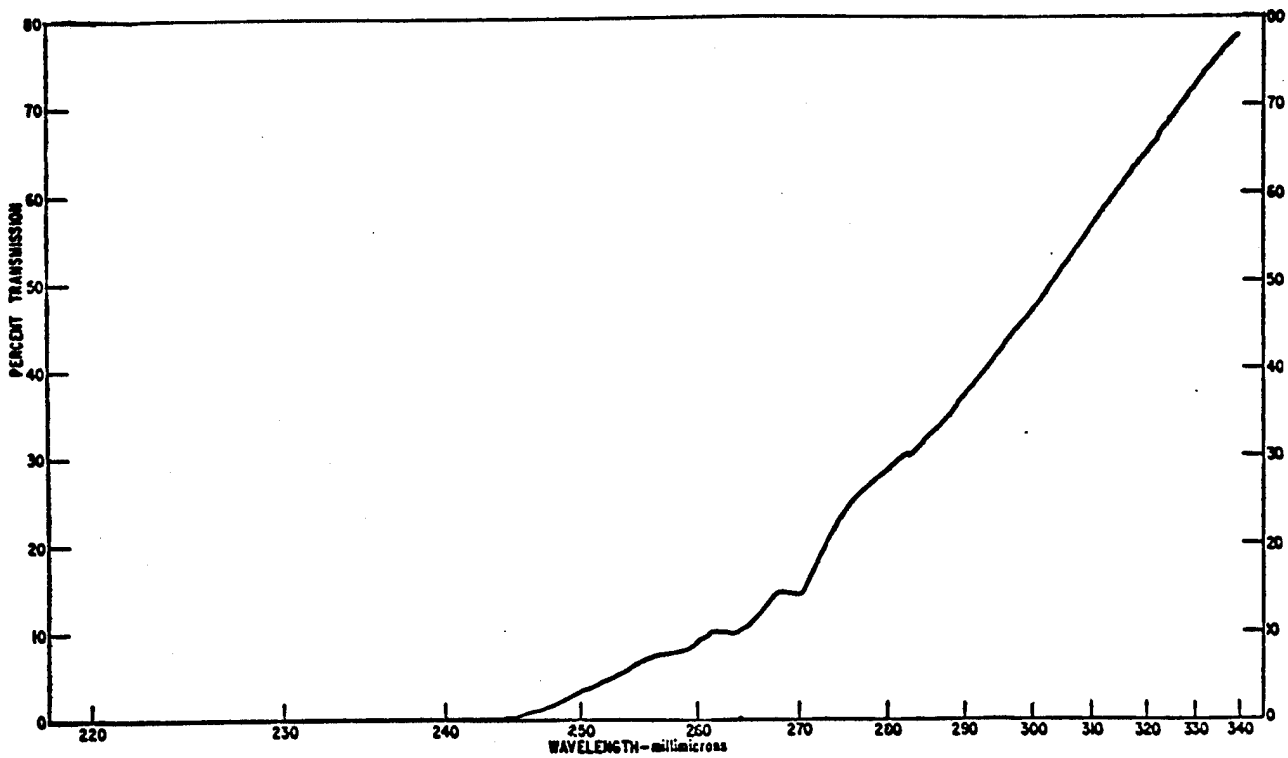
Effects of UV Exposure on RTV 602 (3)
