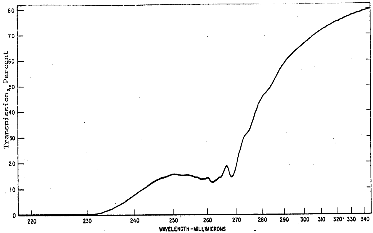
Transmission of GE RTV-615 Cured Section (2)
