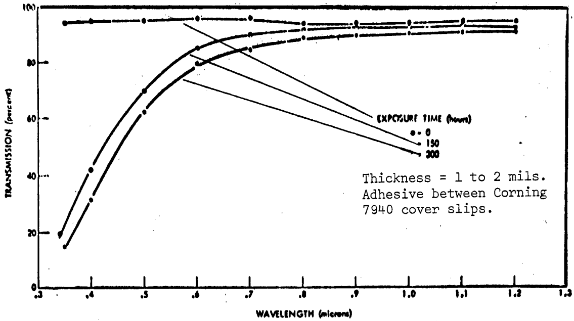
Effects of UV Exposure on RTV 602 (3)
