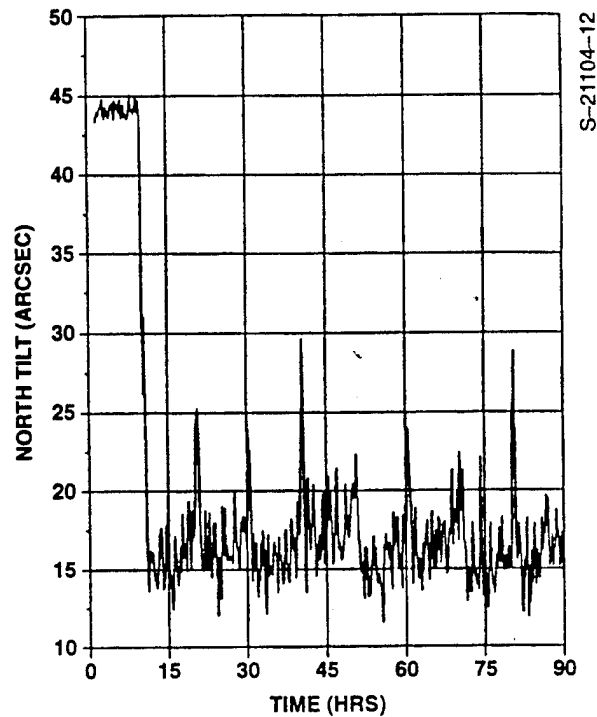
Figure 12. North Tilt for Scenario 2 (turns every 10 hours)
