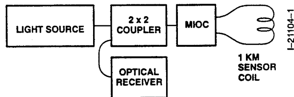
Figure 1. Gyrocompass IFOG Demonstration Unit Optical Configuration Design
