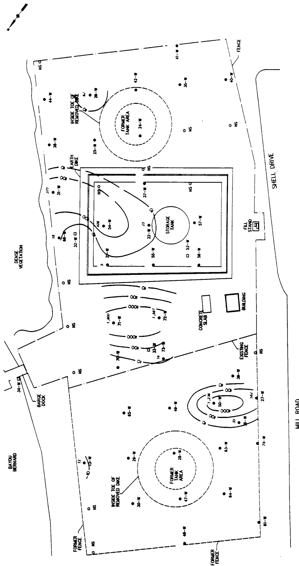
FIGURE 5 Ethylbenzene in the Water (ppb)
