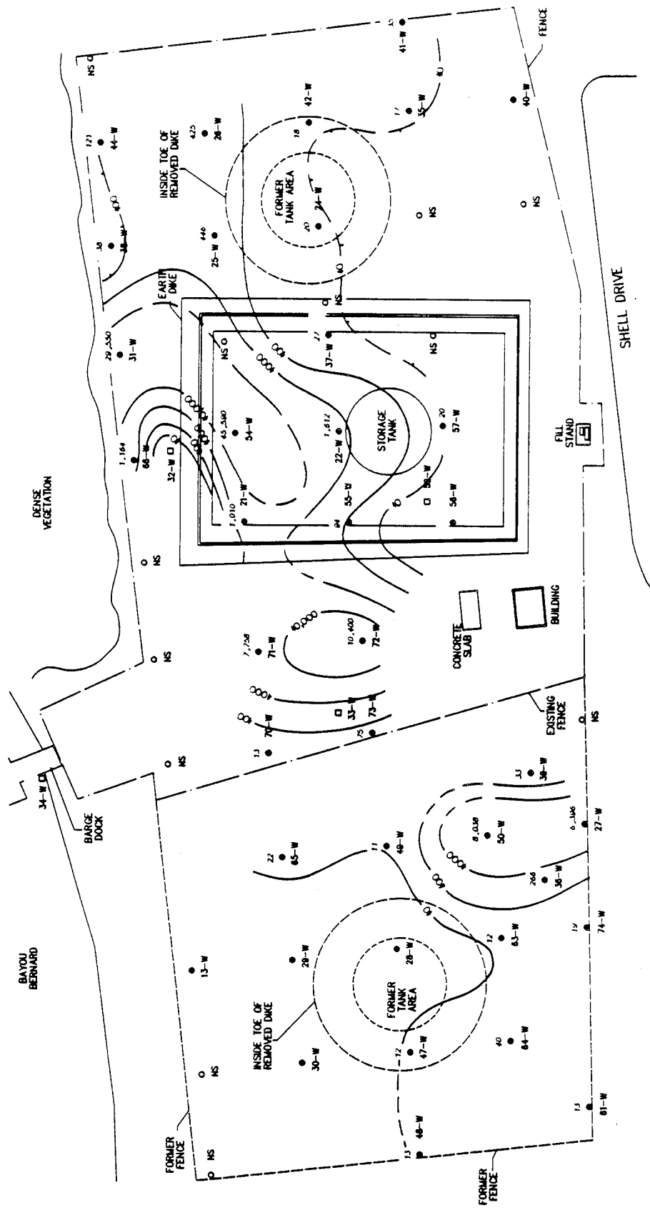
FIGURE 4. Toluene in the Water (ppb.)
