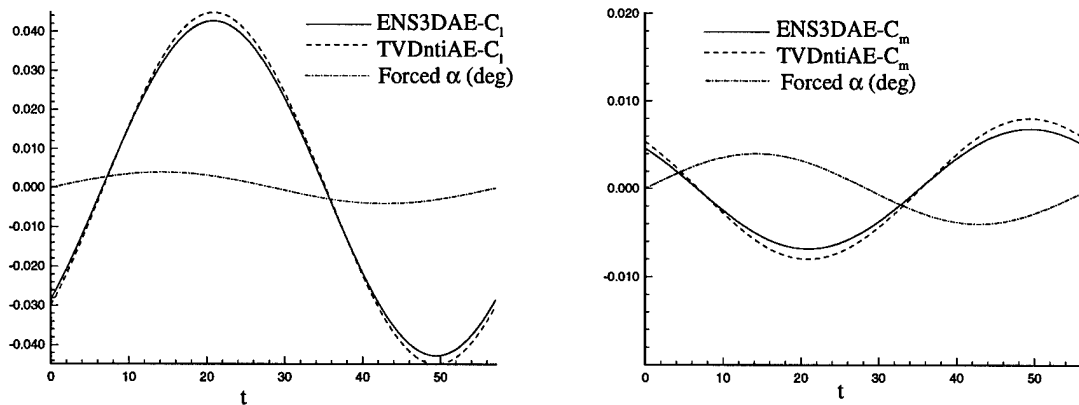
Figure 5.5 NACA 64A006 Forced Pitch Comparison: M_\infty = 0.87
