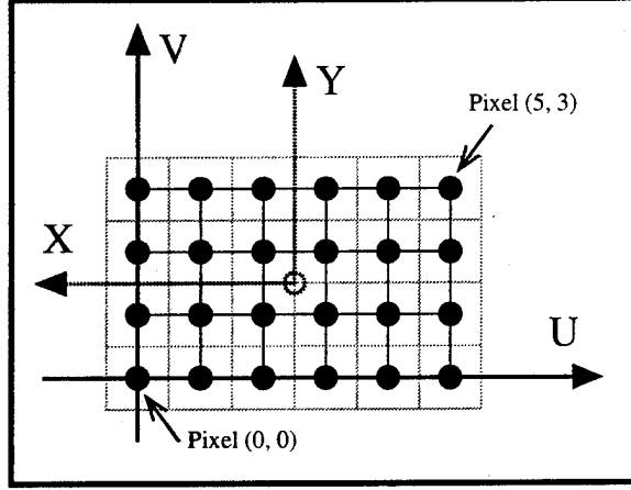
Figure 2: Illustrating pixel coordinate conventions.
