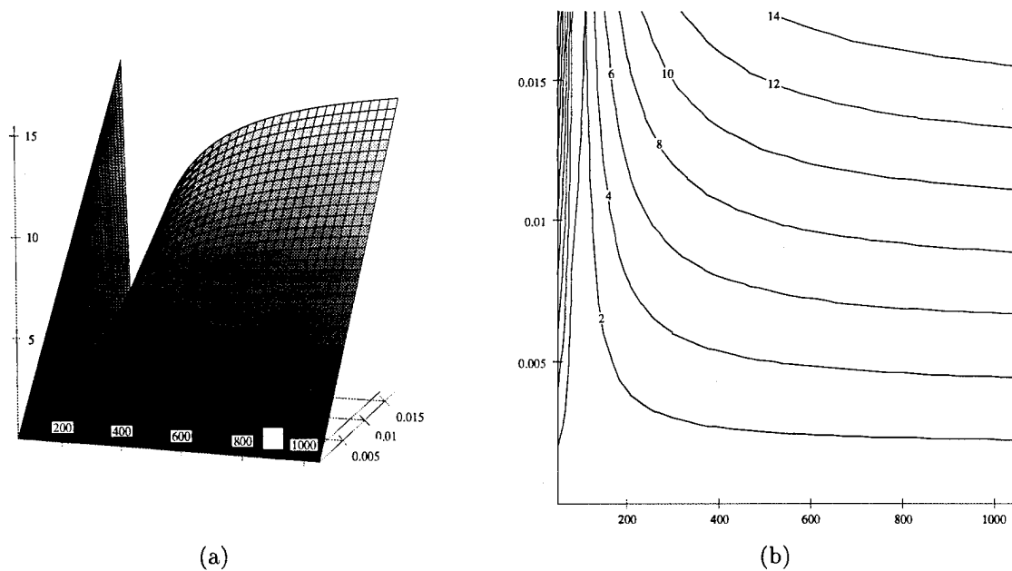
Figure 7: Pixel Differences \Delta over large variations in Depth for a center pixel as a function of Z and \phi_y . a) surface plot with \Delta vertical, Z facing and \phi_y back into page. b) contour plot of same data with \phi_y vertical and Z horizontal.
