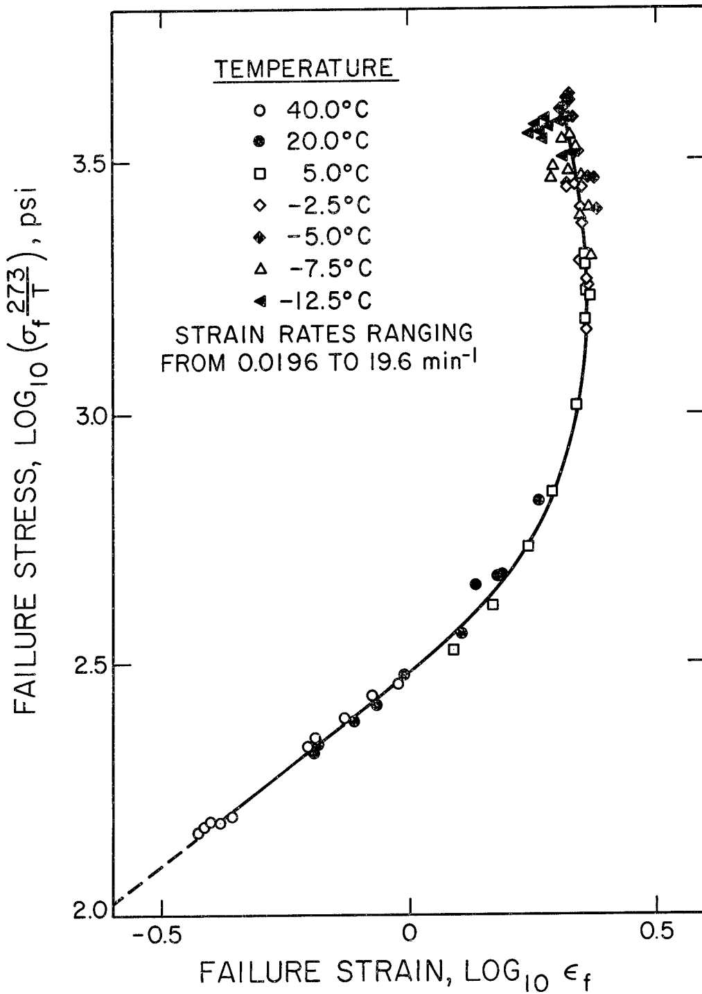
Fig.21 FAILURE ENVELOPE FOR UNSWOLLEN SOLITHANE 50/50
