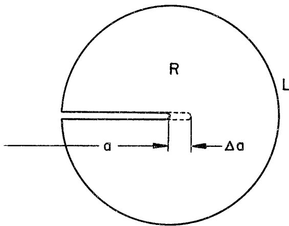
FIG. 2 CONTROL VOLUME
