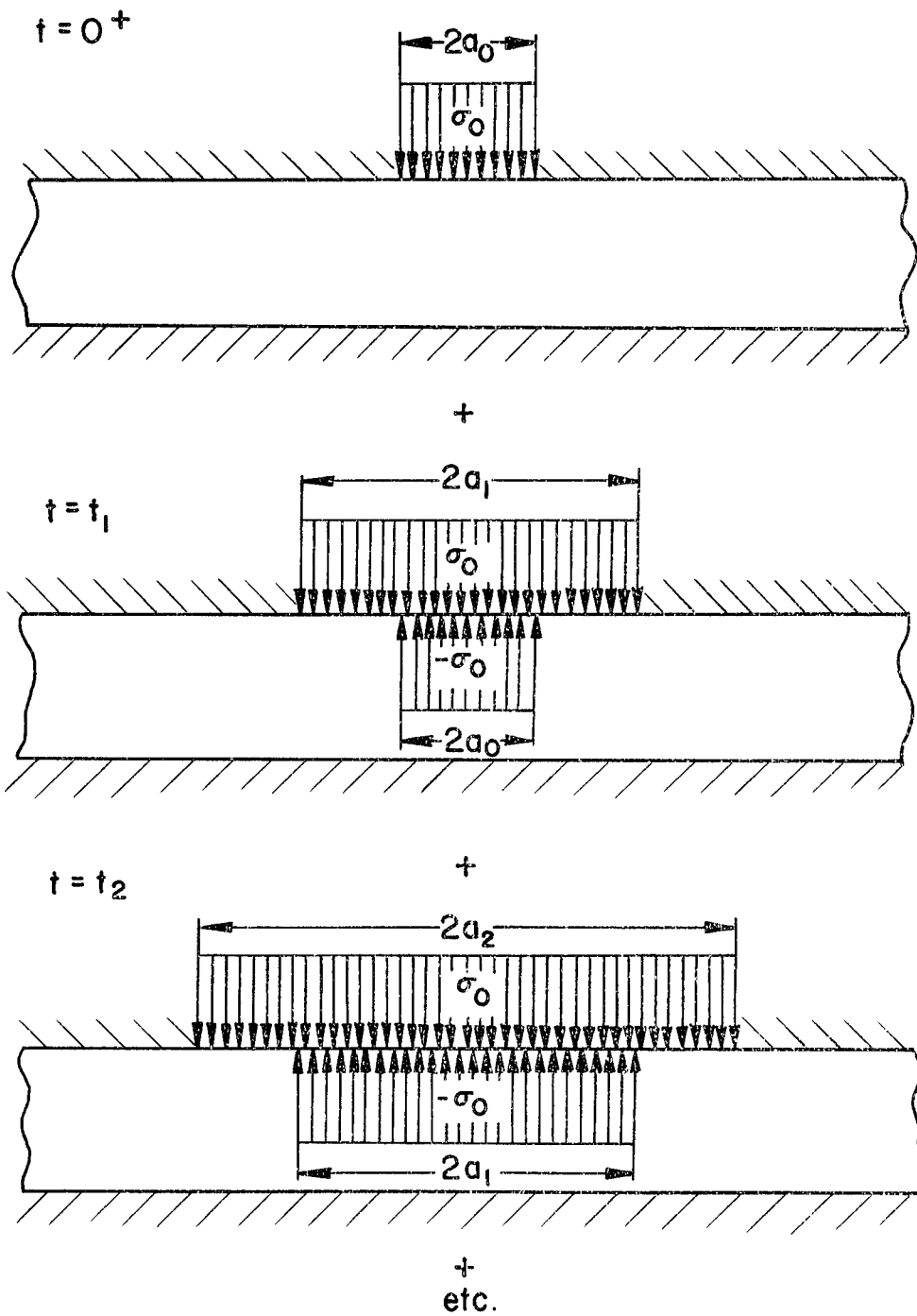
FIG.12 SUPERPOSITION SCHEME
