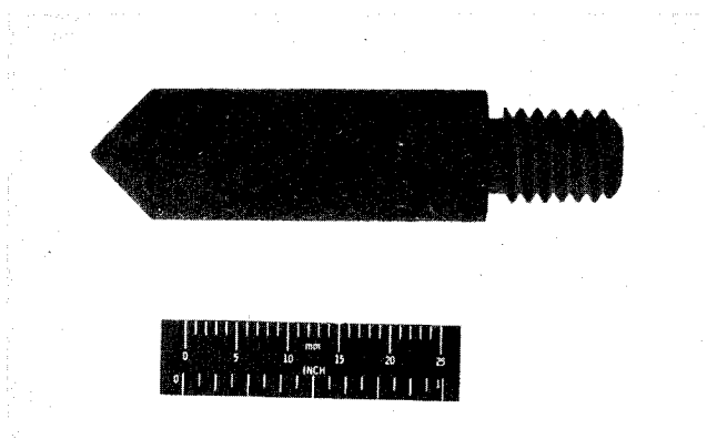
(b) Typical cone-cylinder model for test runs in the ceramic-heated tunnel at a Mach number of 2.
