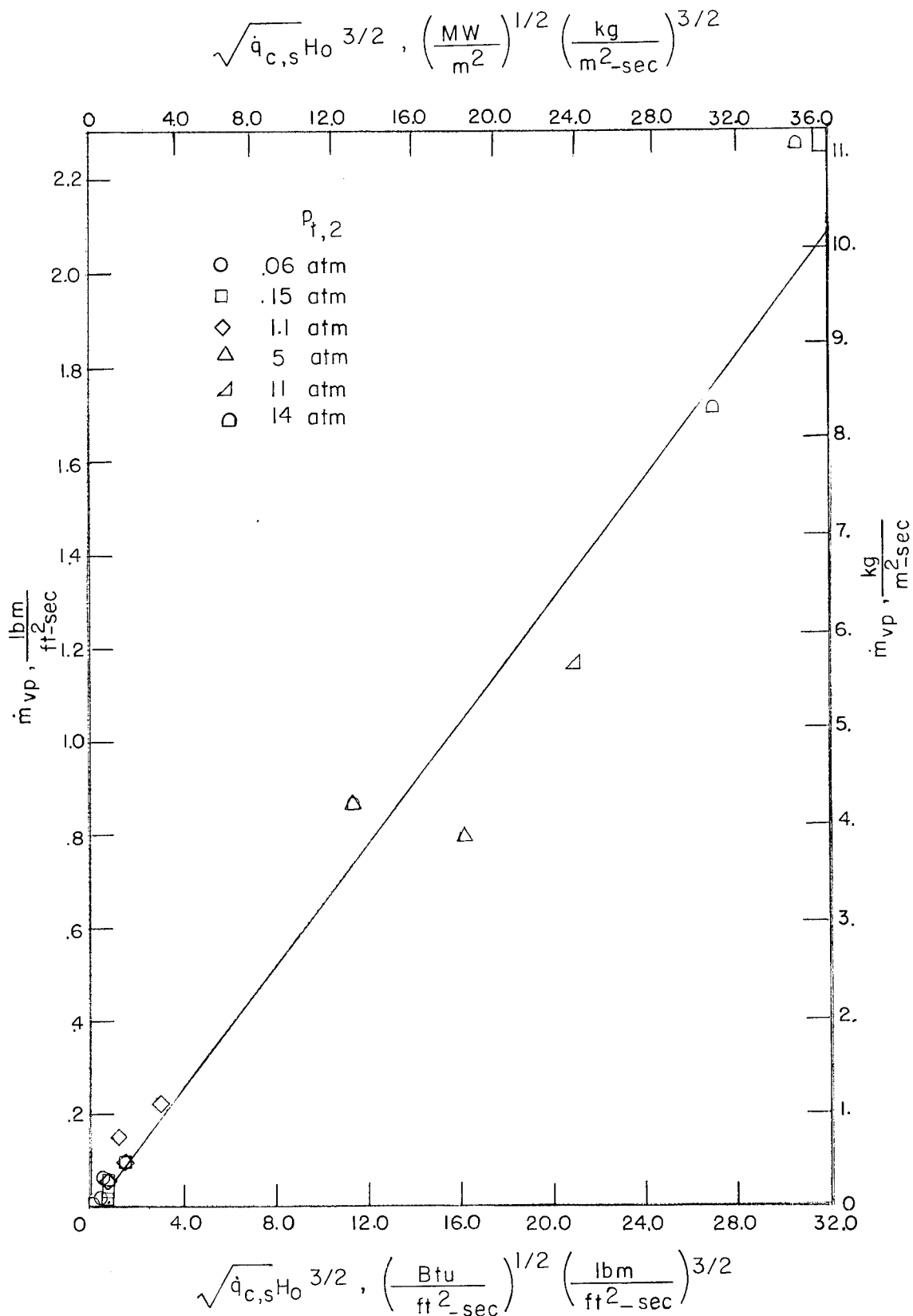
Figure 13.- Mass-loss rate as a function of oxygen-shear product for test runs in air.
