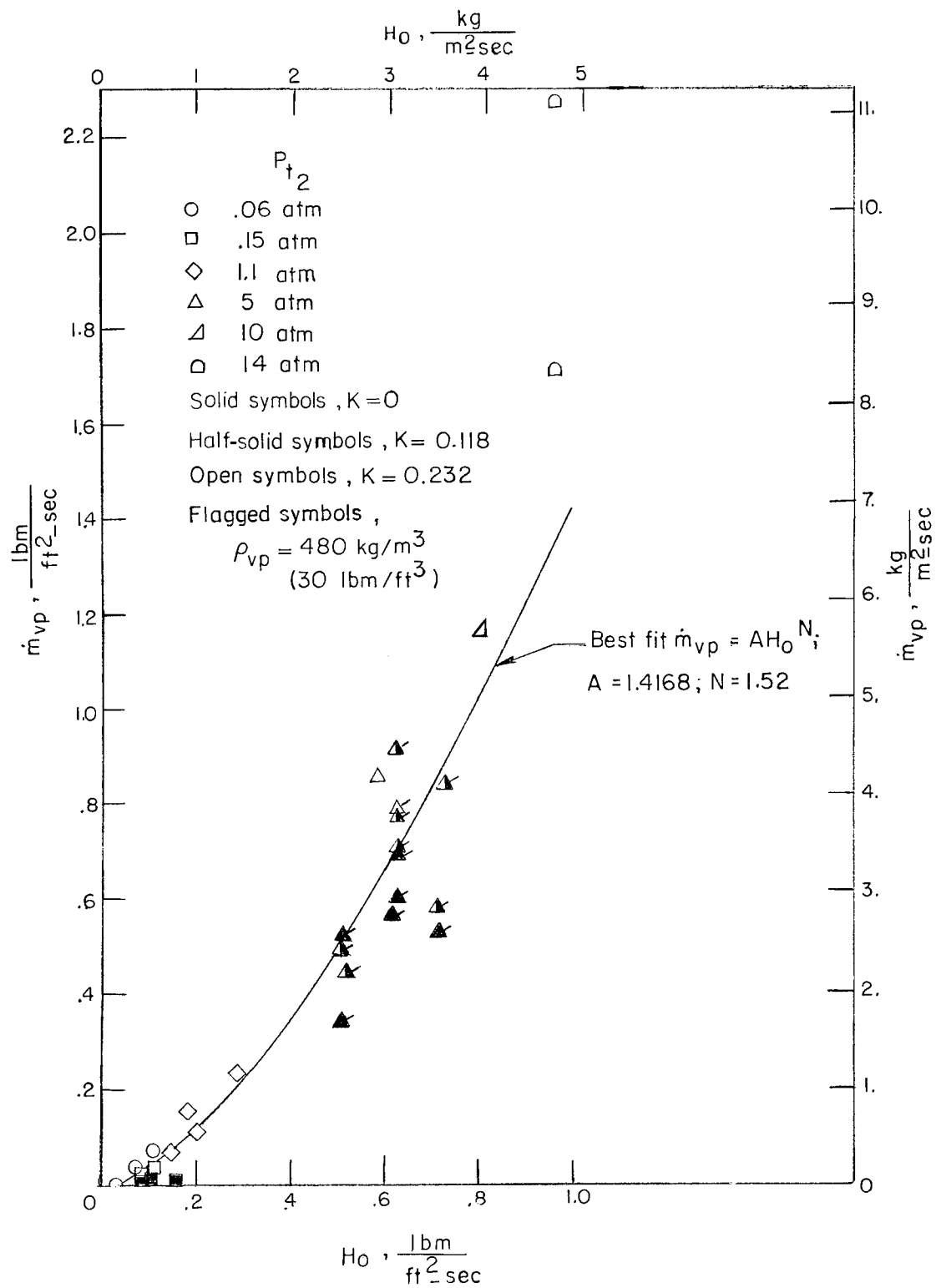
Figure 11.- Mass-loss rate as a function of heat-transfer coefficient for all test runs.
