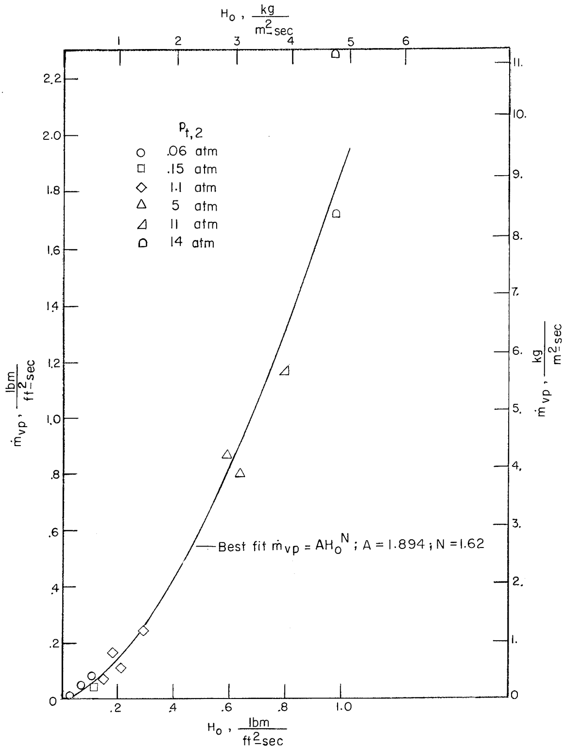
Figure 12.- Mass-loss rate as a function of heat-transfer coefficient for test runs in air.
