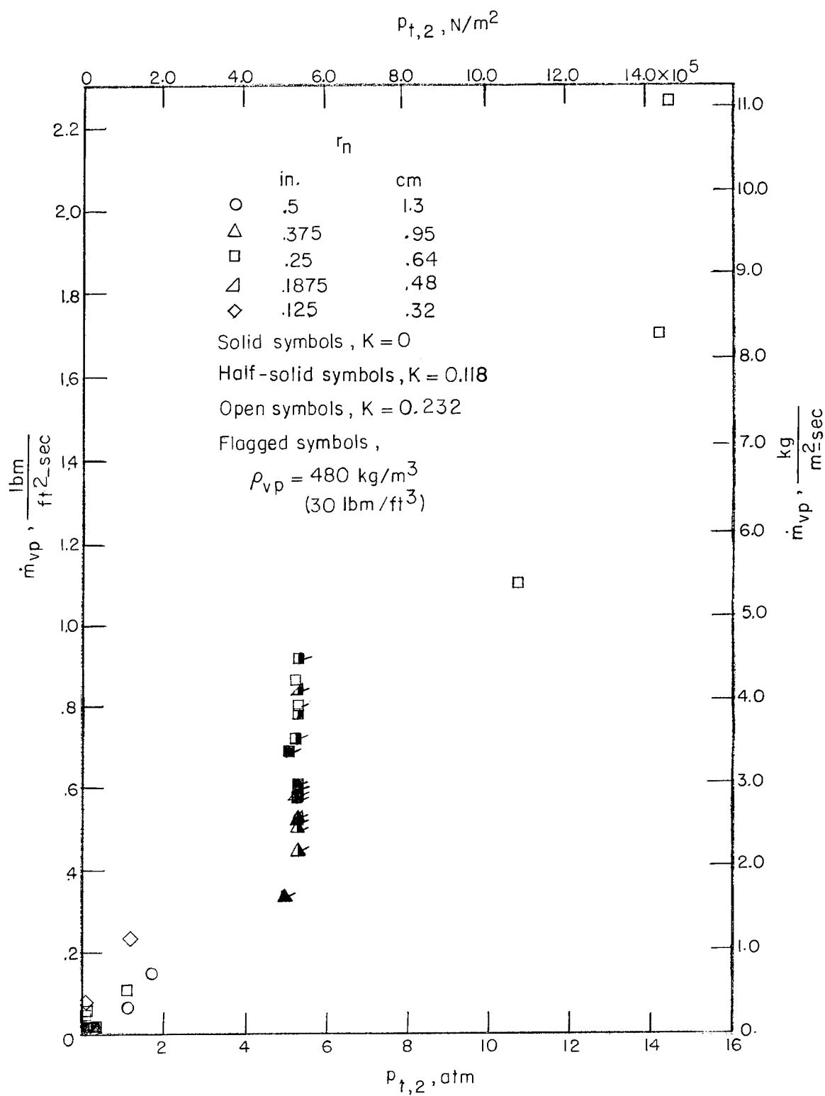
Figure 10.- Mass-loss rate as a function of stagnation pressure for all test runs.
