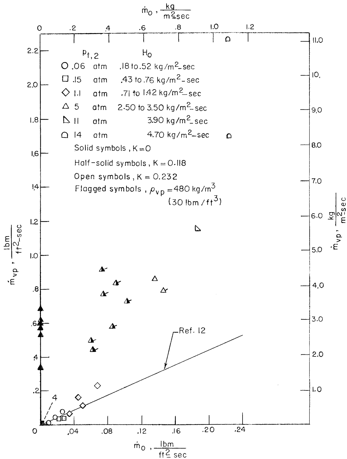
Figure 9.- Mass-loss rate as a function of diffusion-controlled oxygen flux for all test runs.
