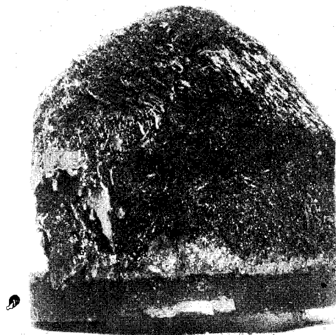
(c) Run 30; K = 0.232 ; p_{t,2} \approx 5 atm; run time 2 sec; H_0 = 3.10 kg/m 2 -sec.
