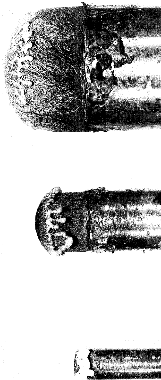
(a) Run 3; H_0 = 0.520 \text{ kg/m}^2\text{-sec} ; run time 30 sec; r_n = 0.3 \text{ cm} .
