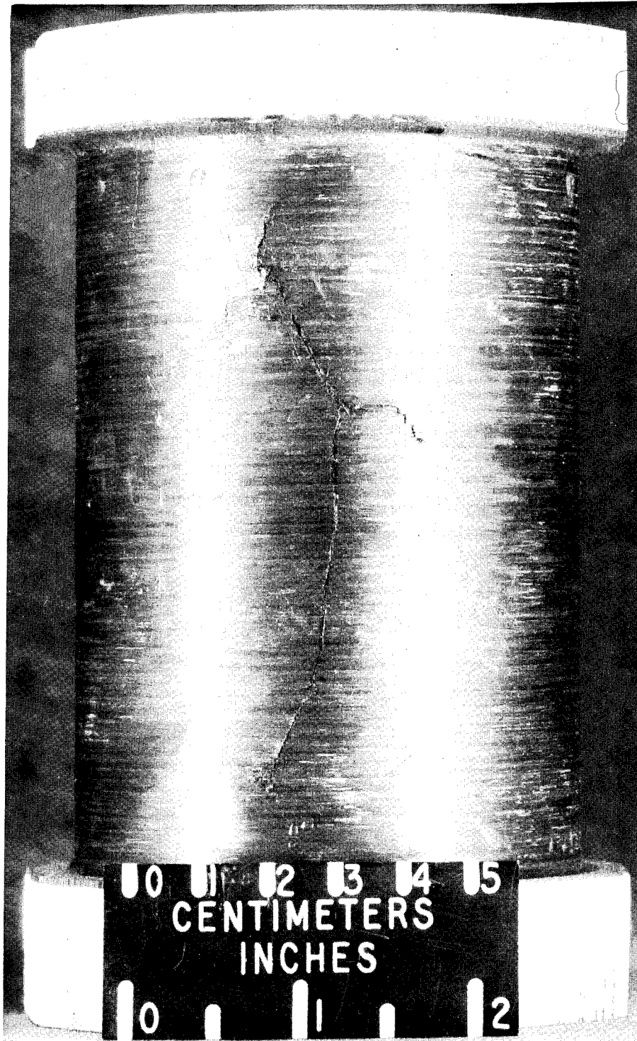
Figure 26.- Isotropic boron-epoxy cylinder failed by external pressurization.
