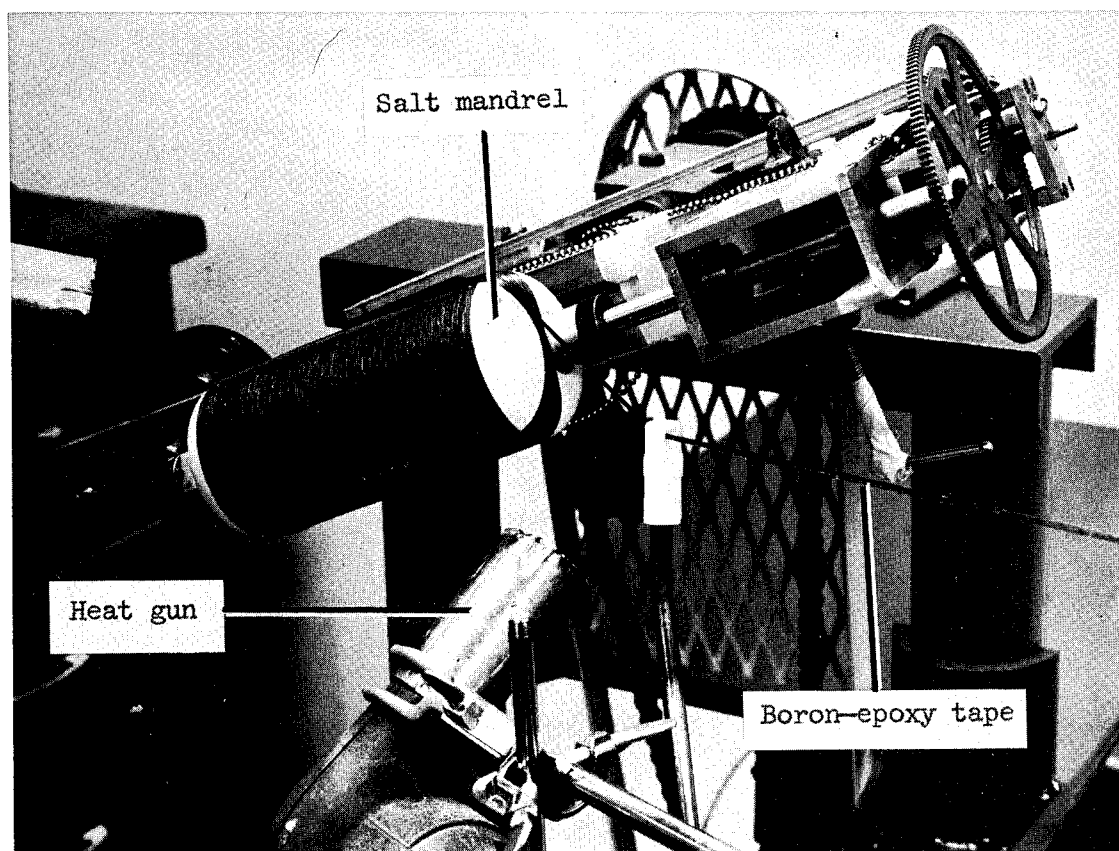
Figure 3.- Longitudinal winding of boron-epoxy tape onto a salt mandrel.
