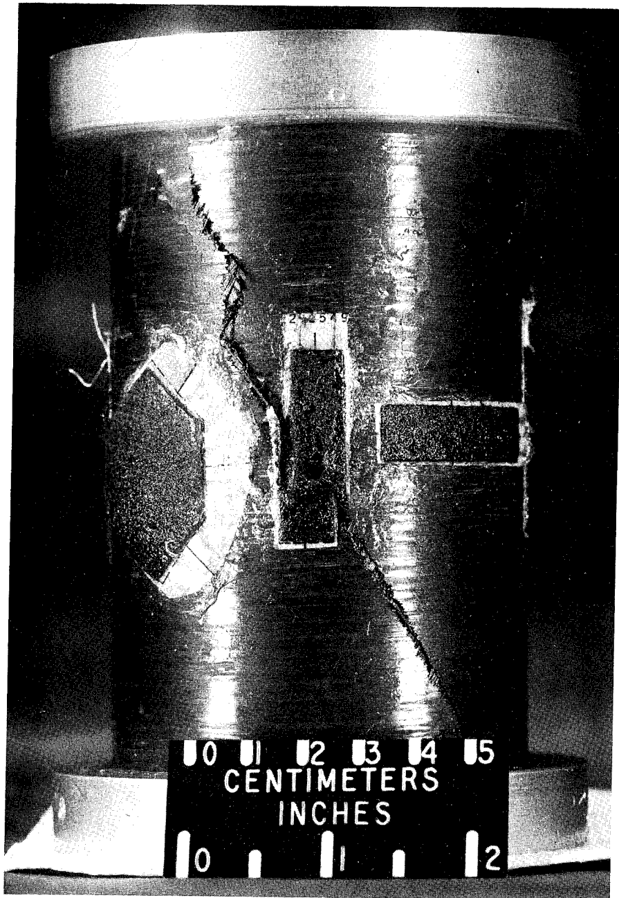
Figure 22.- Isotropic boron-epoxy cylinder failed by internal pressurization. L-66-10070
