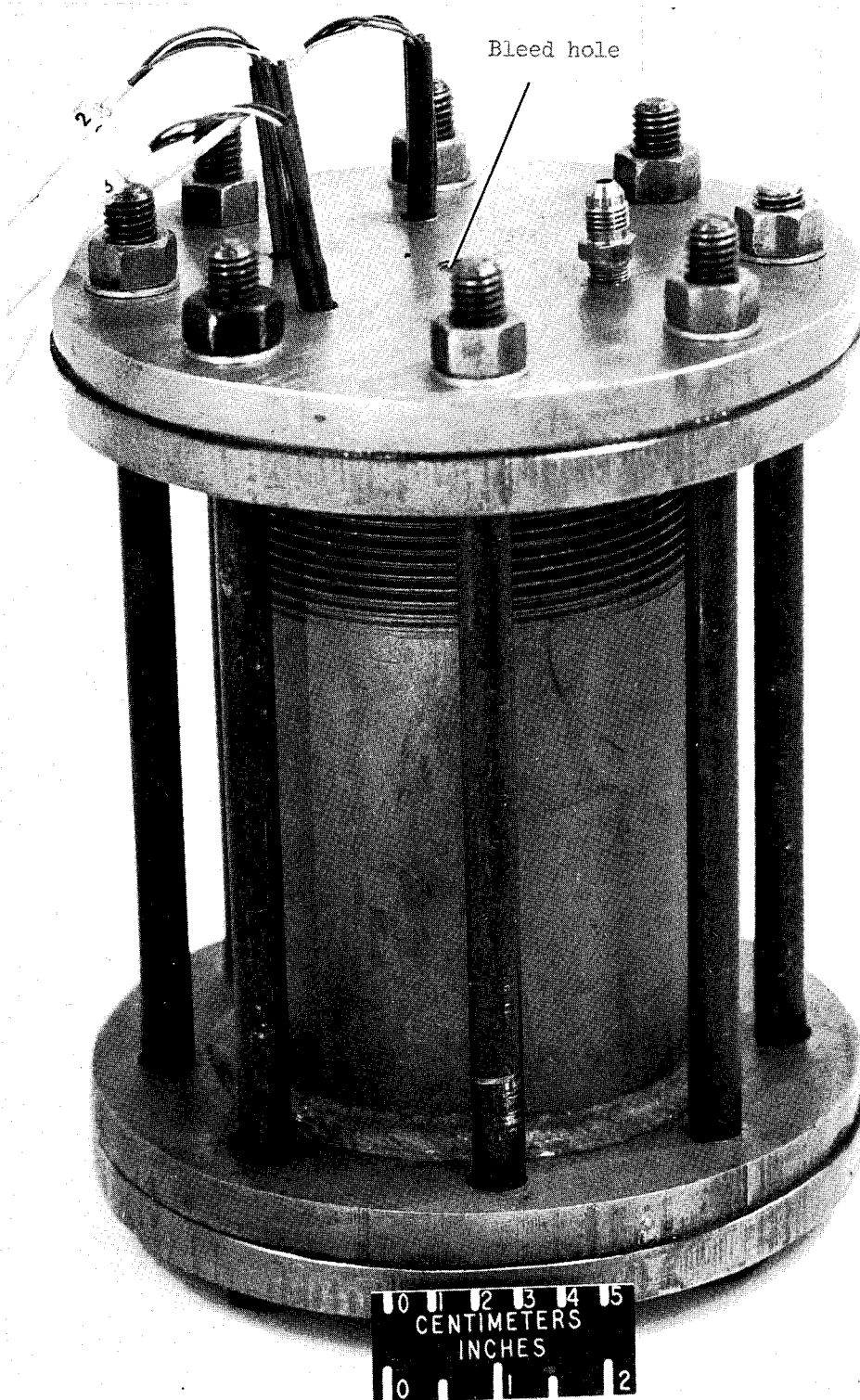
Figure 16.- Closed chamber with cylinder specimen inside ready for external pressure testing.
