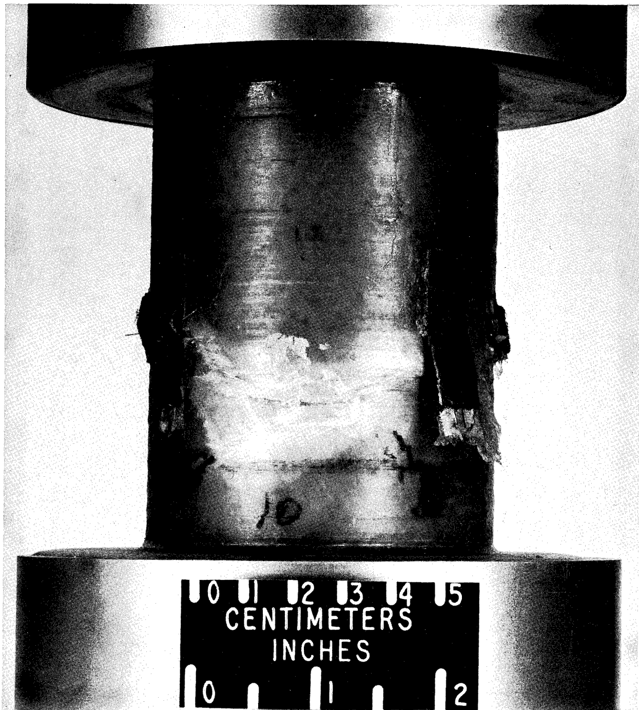
Figure 32.- Isotropic glass-epoxy cylinder failed by axial compression.
