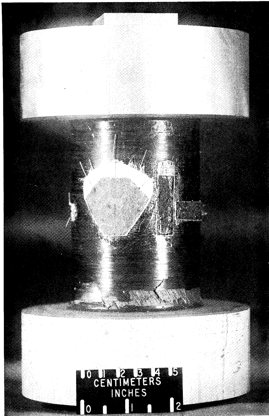
Figure 30.- Isotropic boron-epoxy cylinder failed by axial compression.
