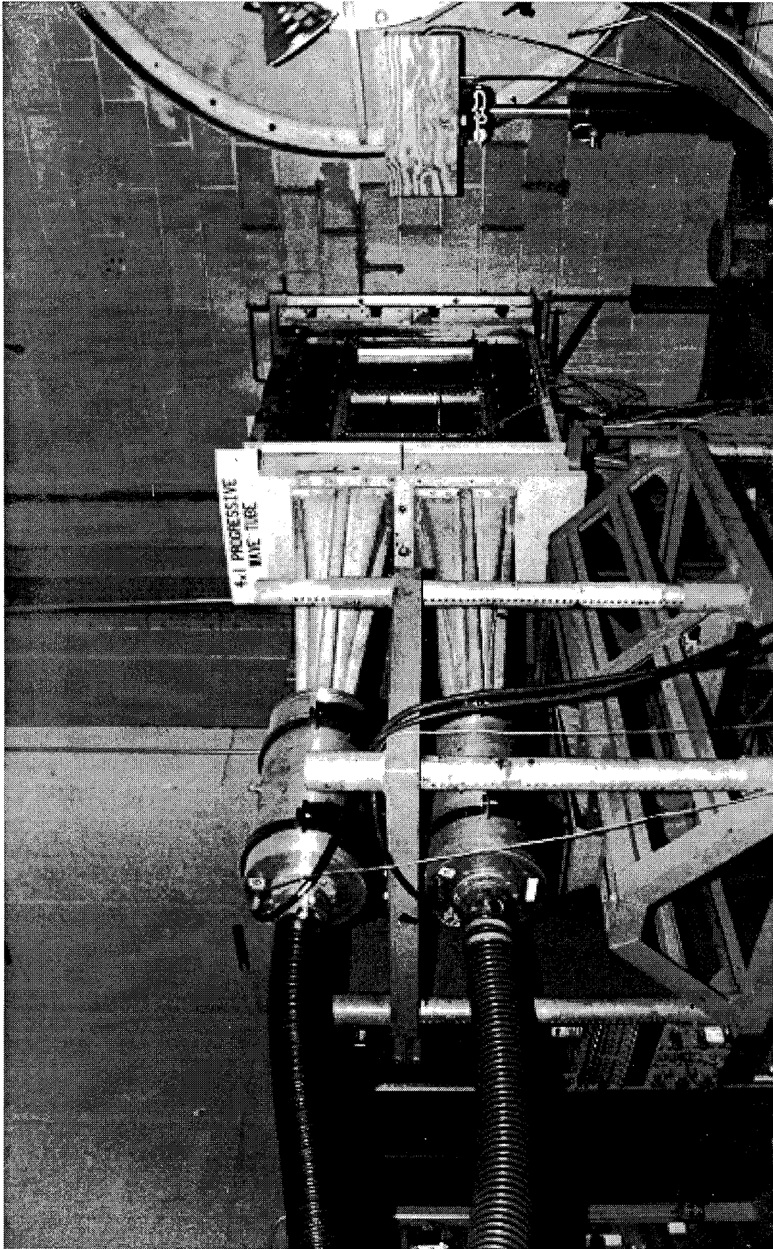
Fig 3.70 Photograph of C-C-C CFRP plate installation in APWT.
