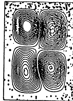
Fig 3.68 Mode shape, video holography method, a=59 Hz, b=77 Hz, c=107 Hz, d=139 Hz, e=160 Hz and f=187 Hz, C-C-C-C CFRP APWT plate.
