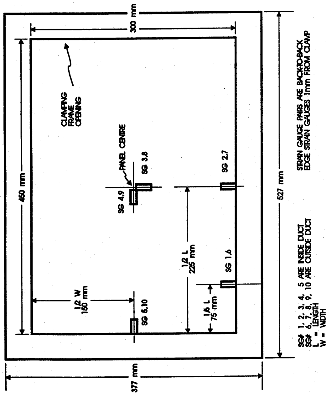
Fig 3.53 C-C-C-C aluminium APWT plate size and strain gauge location.
