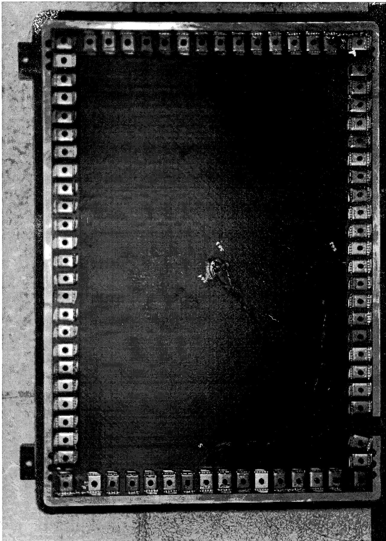
Fig 3.66 Photograph of C-C-C-C CFRP APWT plate clamping arrangement.
