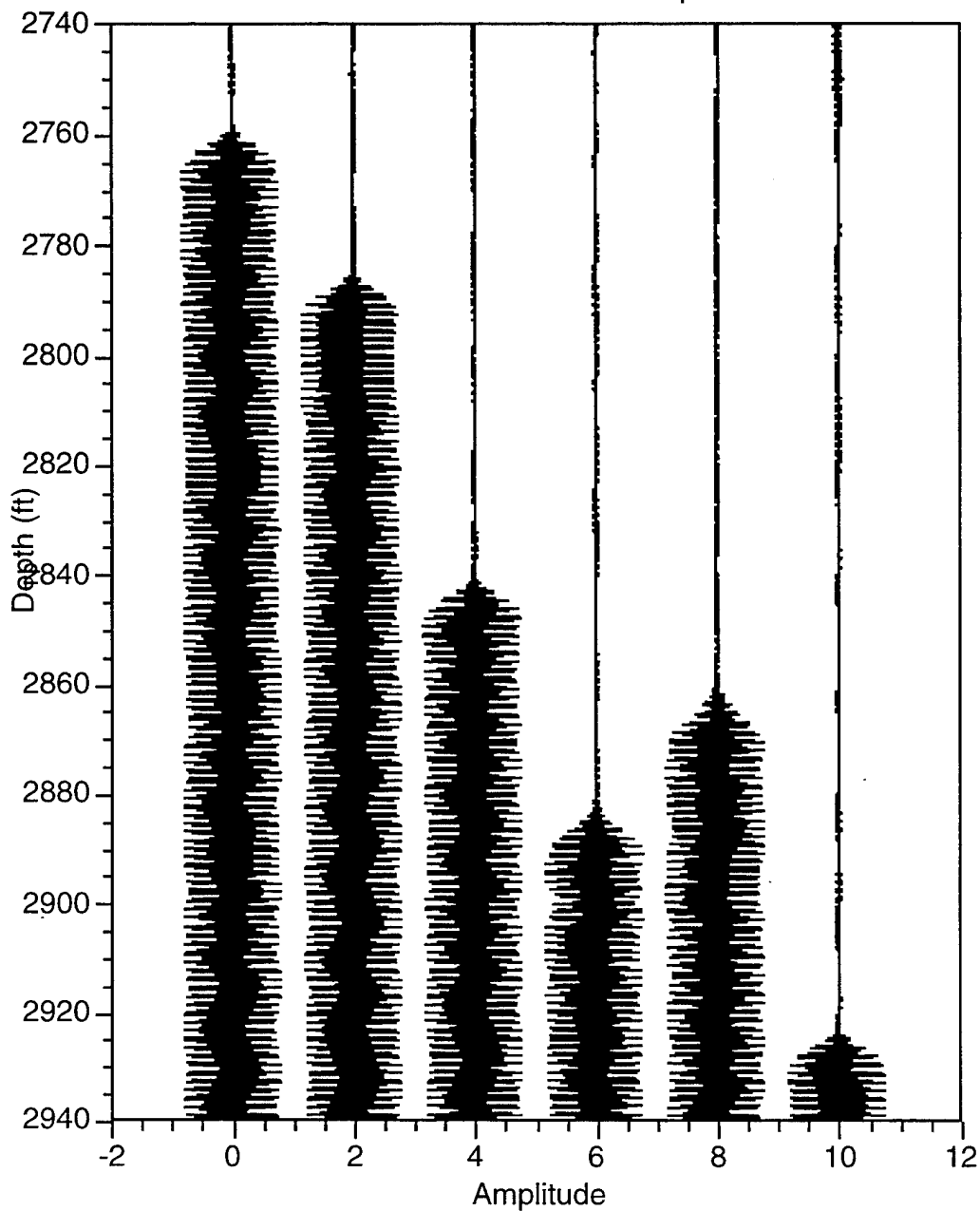
Figure 14. An Example of Six Pings without any Decimation.
