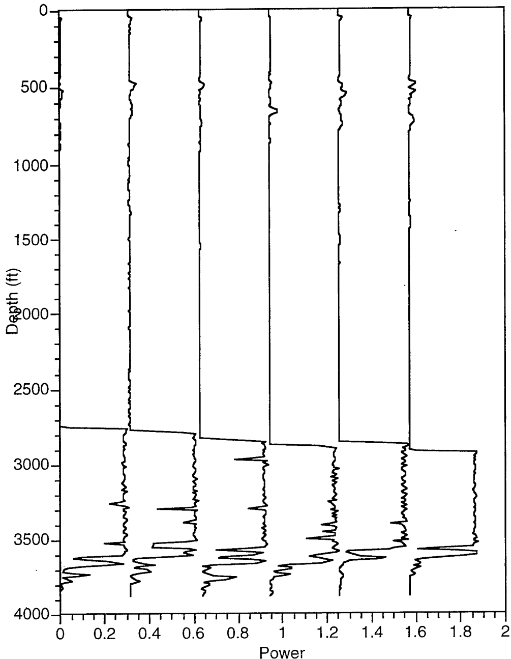
Figure 13. An Example of Decimated Data from Six Acoustic Pings.
