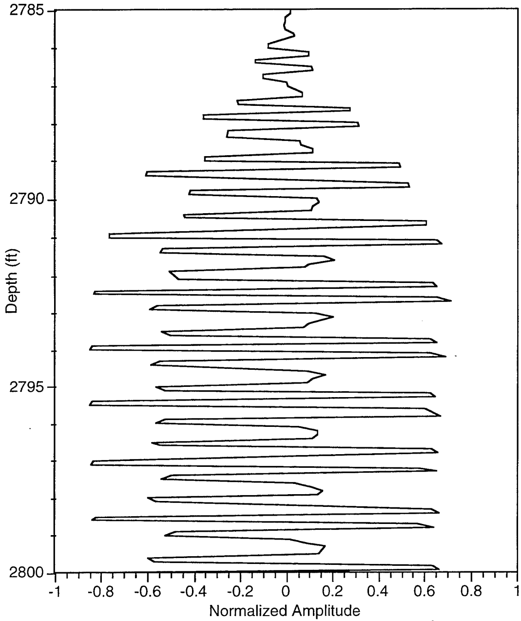
Figure 17. Time Expanded First Part of Pulse in Figure 16.
