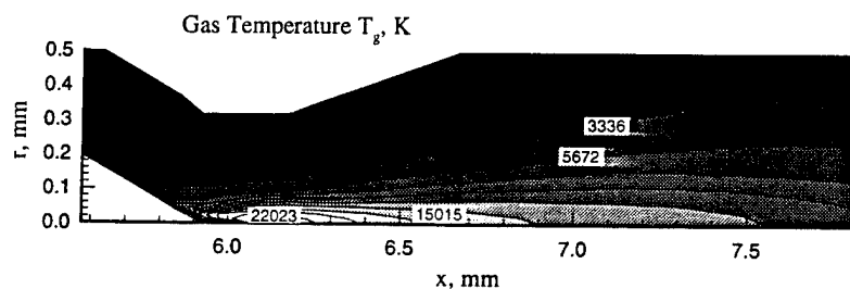
Figure 8: Heavy species temperature for hydrazine; chemical equilibrium (CE) simulation. The maximum is T_g \approx 22,000 K at the constricter centerline. The exit plane is located at x = 18.5 mm.
