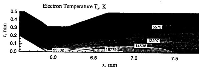
Figure 9: Electron temperature for hydrazine; chemical equilibrium (CE) simulation. The maximum is T_e \approx 23,500 K at the constricter centerline. The exit plane is located at x = 18.5 mm.
