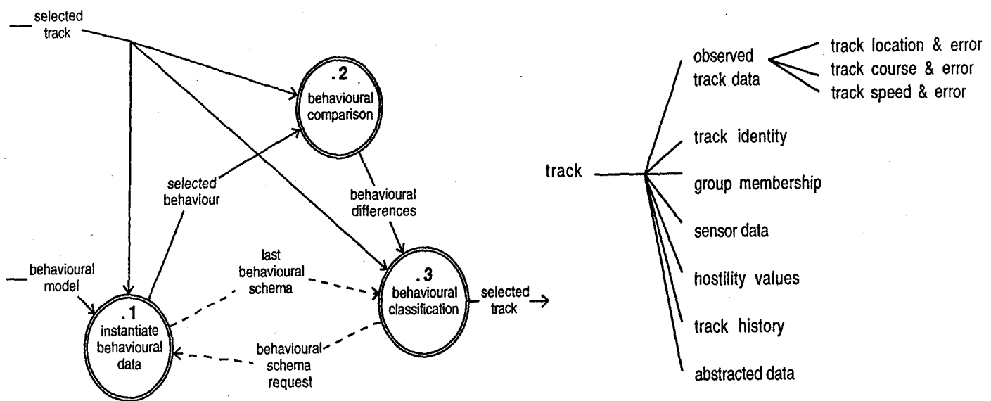
Figure 3 - Track analysis data flow decomposition
