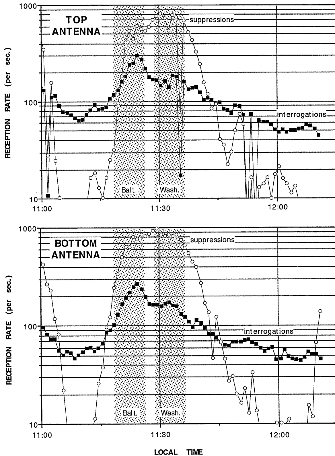
Figure 11. Total interrogations and suppressions received by the AMF (Washington).
