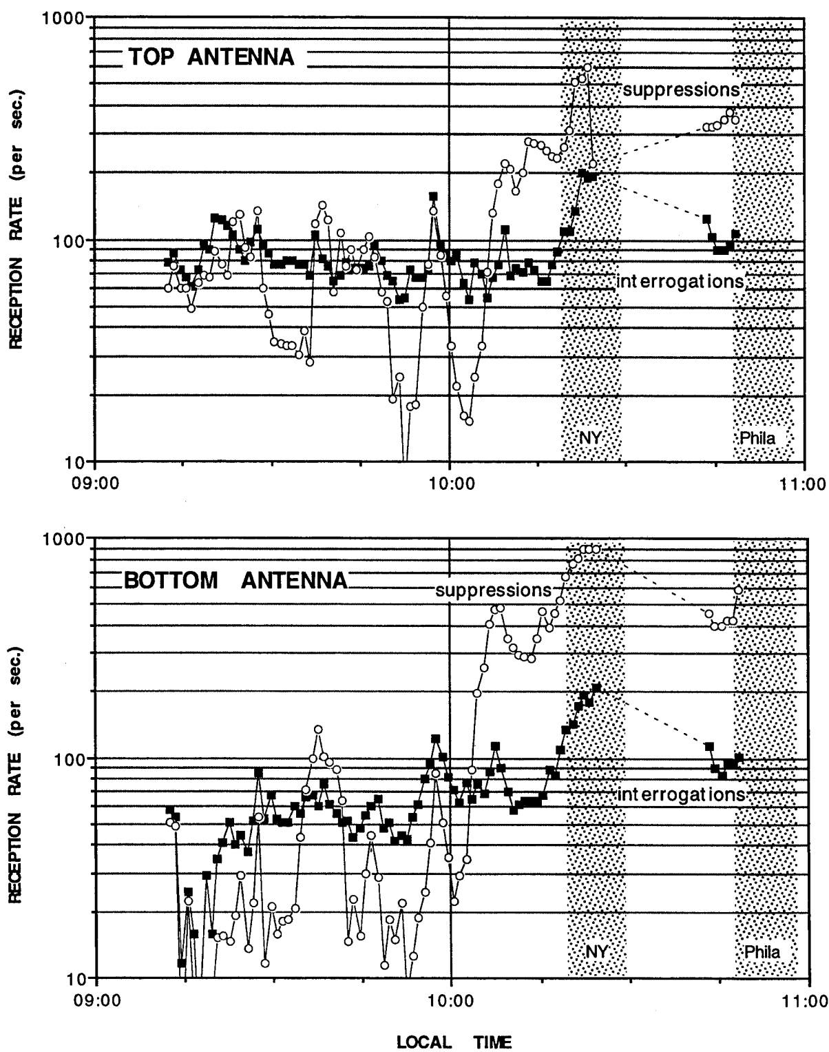
Figure 4. Total interrogations and suppressions received by the AMF.
