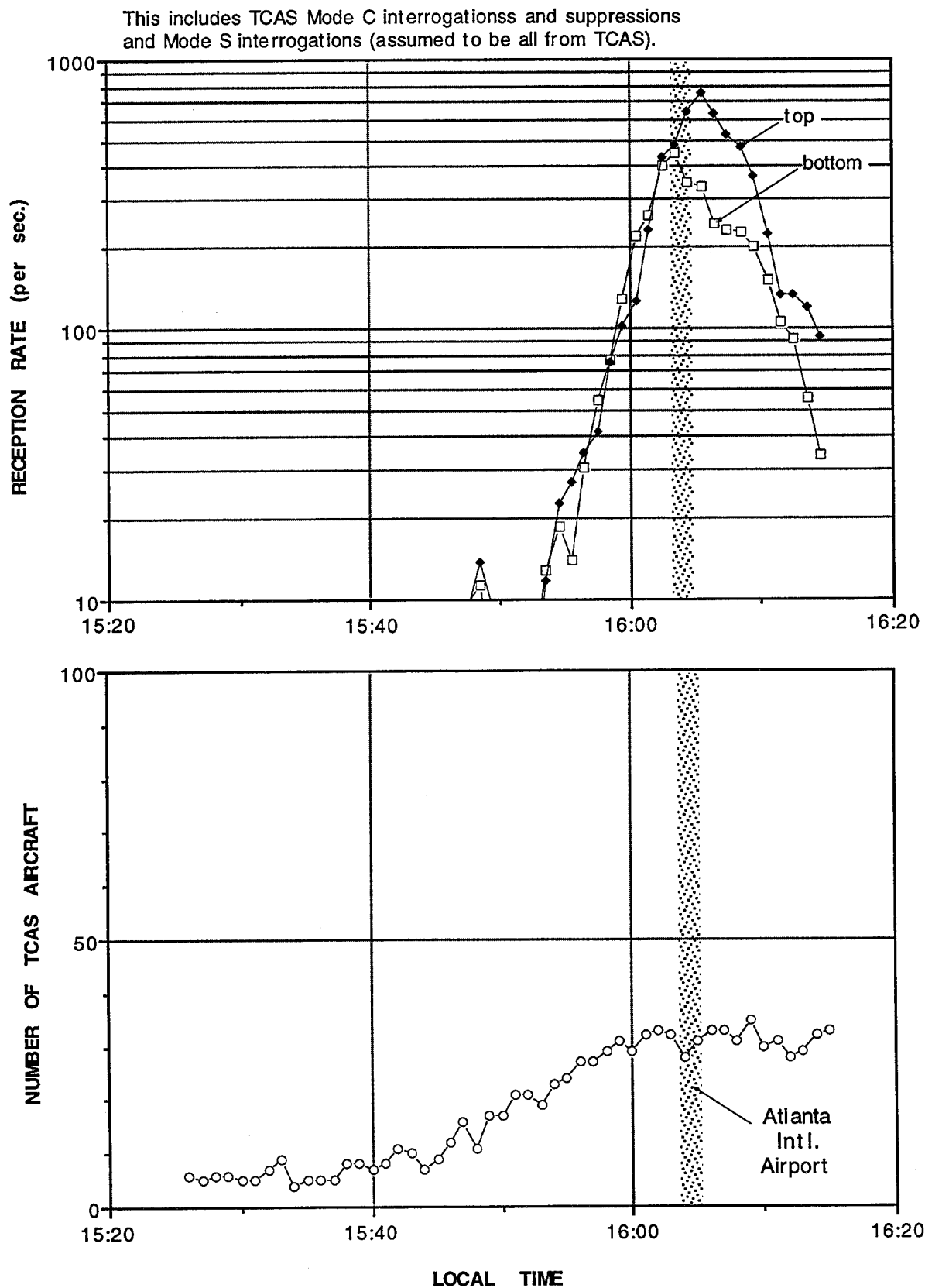
Figure 17. Total TCAS interrogations and suppressions received by the AMF (Atlanta).
