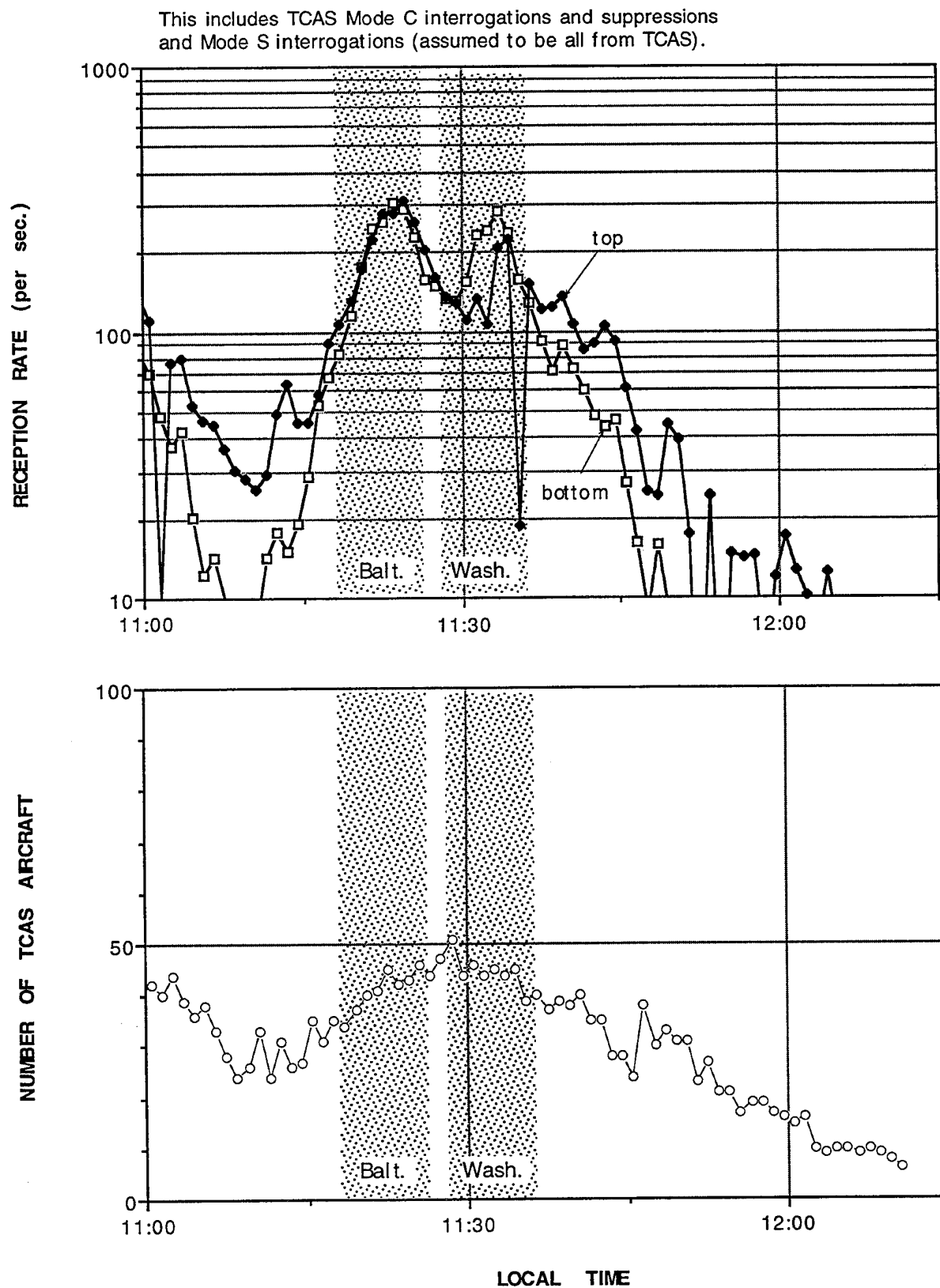
Figure 13. Total TCAS interrogations and suppressions received by the AMF, Washington.
