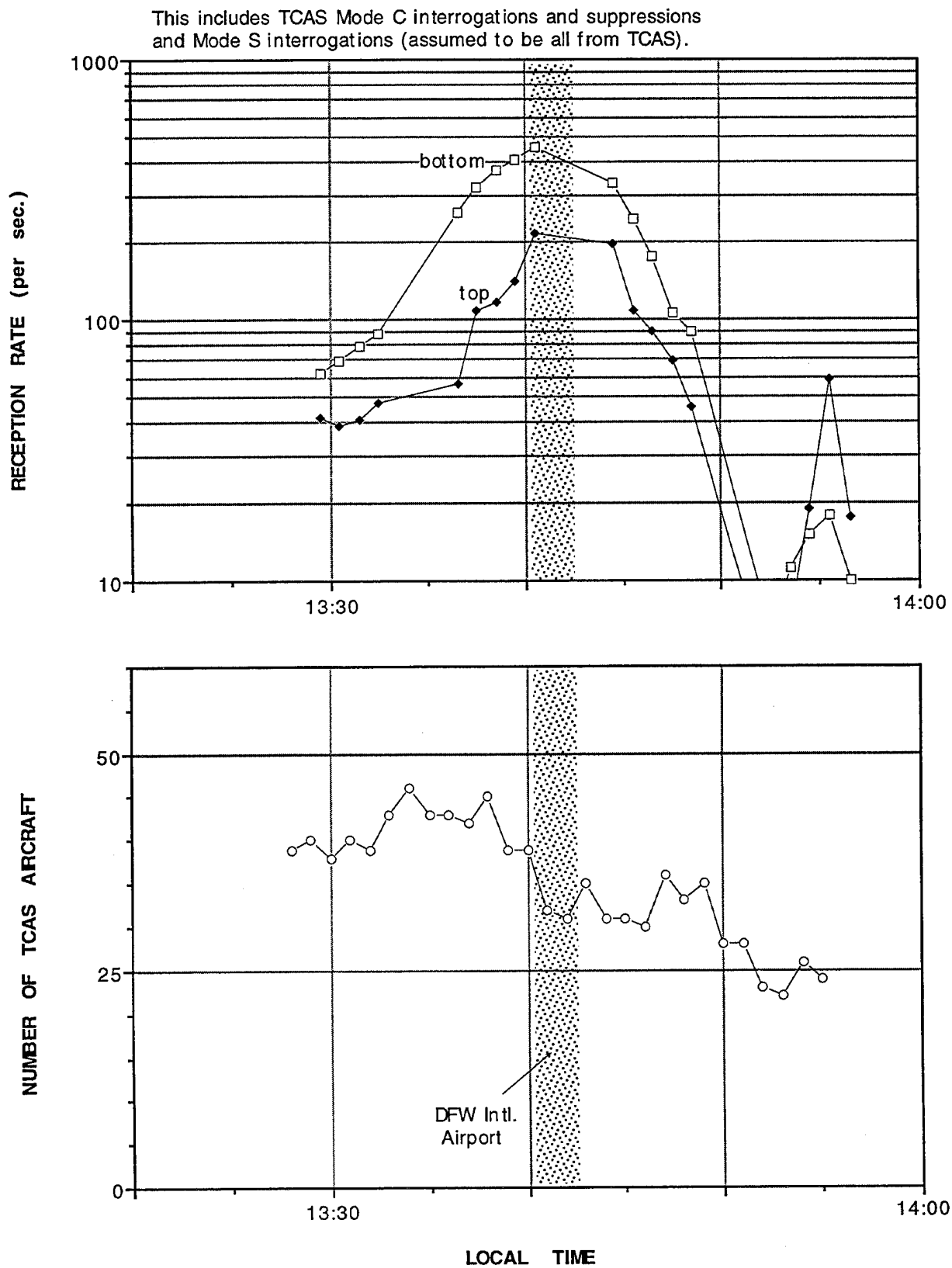
Figure 21. Total TCAS interrogations and suppressions received by the AMF (Dallas).
