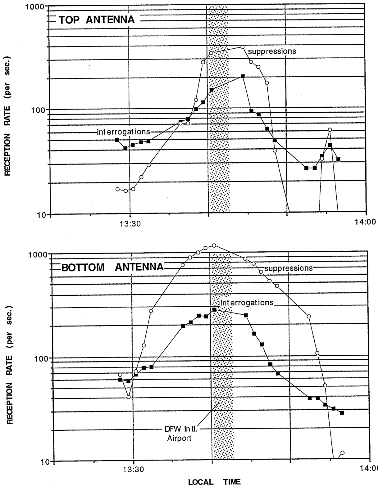
Figure 19. Total interrogations and suppressions received by the AMF (Dallas).
