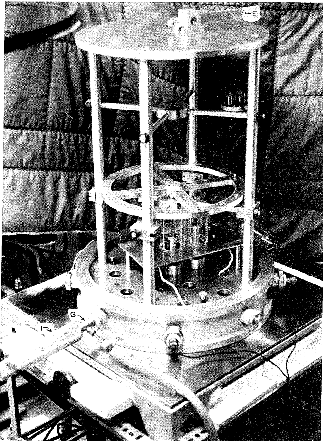
Figure 2. The Torsion Pendulum, Top-Front View.
