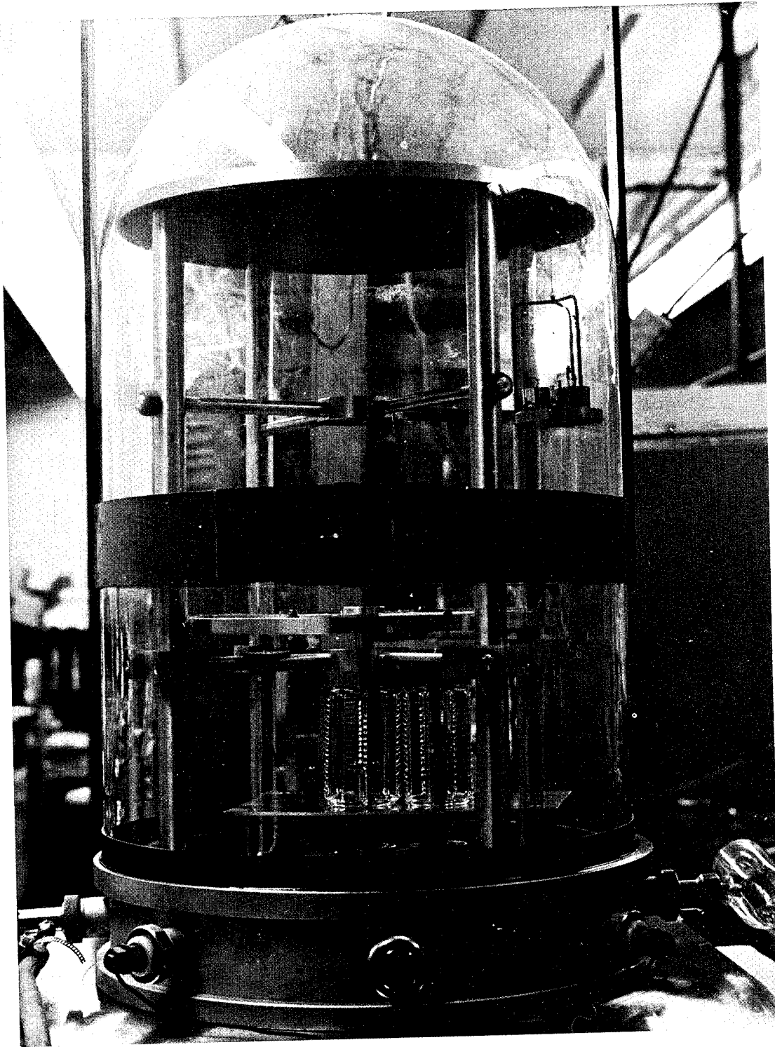
Figure 3. The Torsion Pendulum with the Bell Jar in Place.
