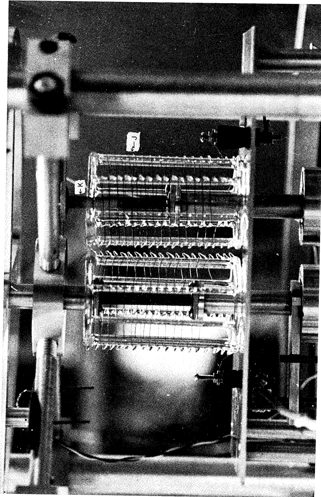
Figure 6. Detail of the Torsion Pendulum Heating Coils.
