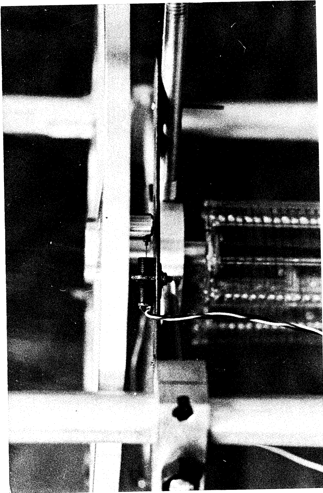
Figure 5. Detail of the Torsion Pendulum Showing the LVDT.
