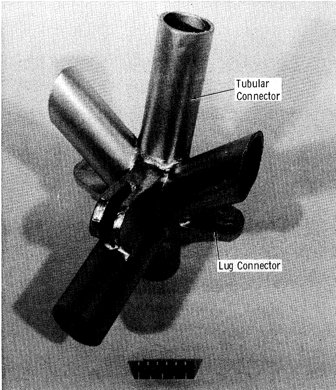
Figure 2.- Model of three-dimensional joint cluster.
