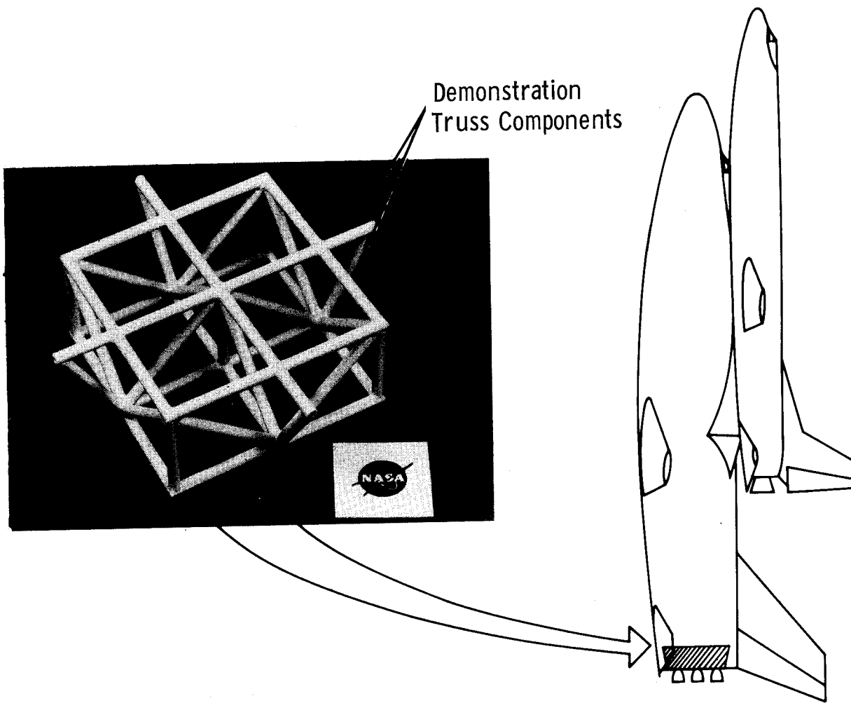
Figure 1.- Space shuttle booster thrust structure.
