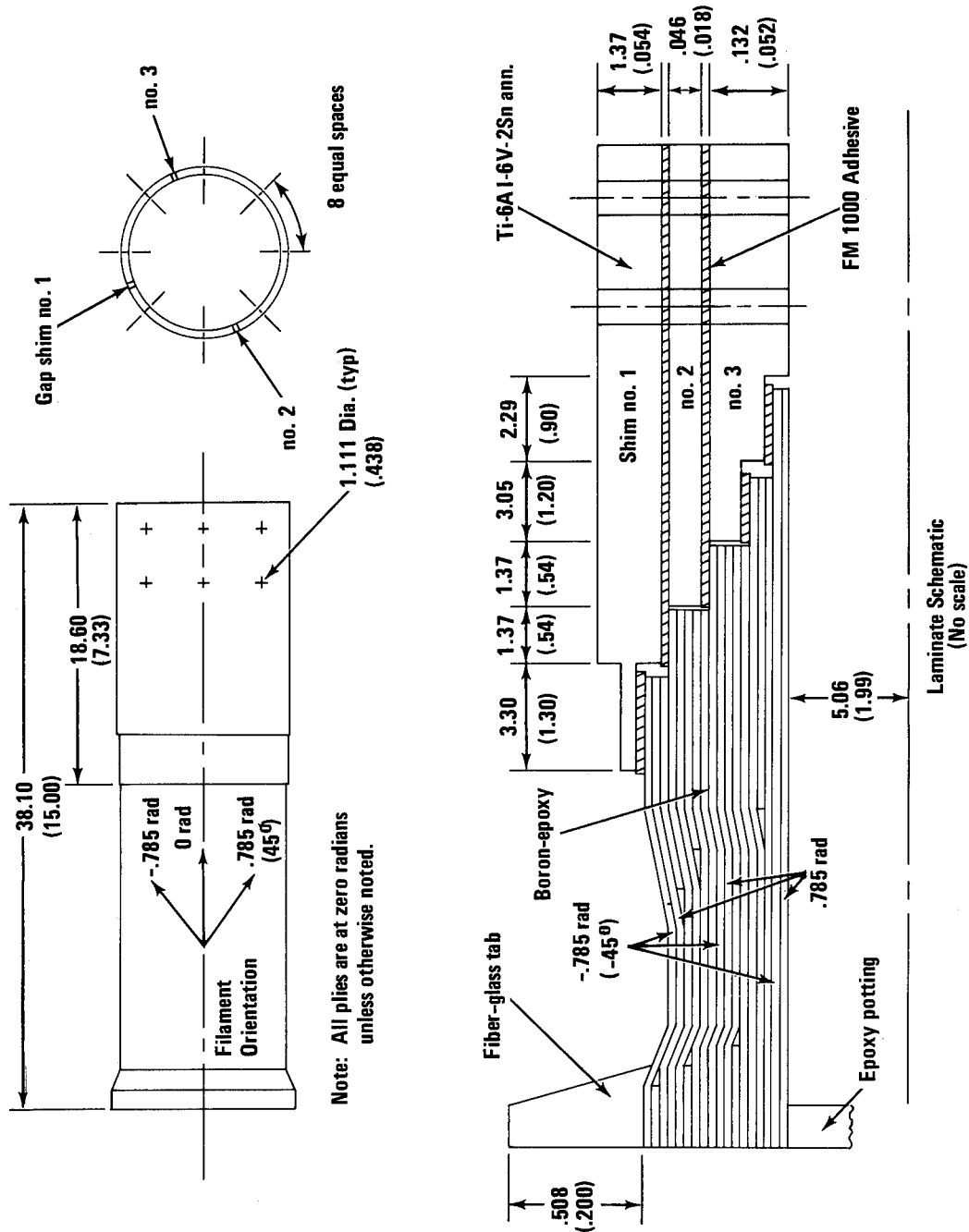
Figure 8.- Compression subelement specimen, all composite. Dimensions are given in centimeters (inches).
