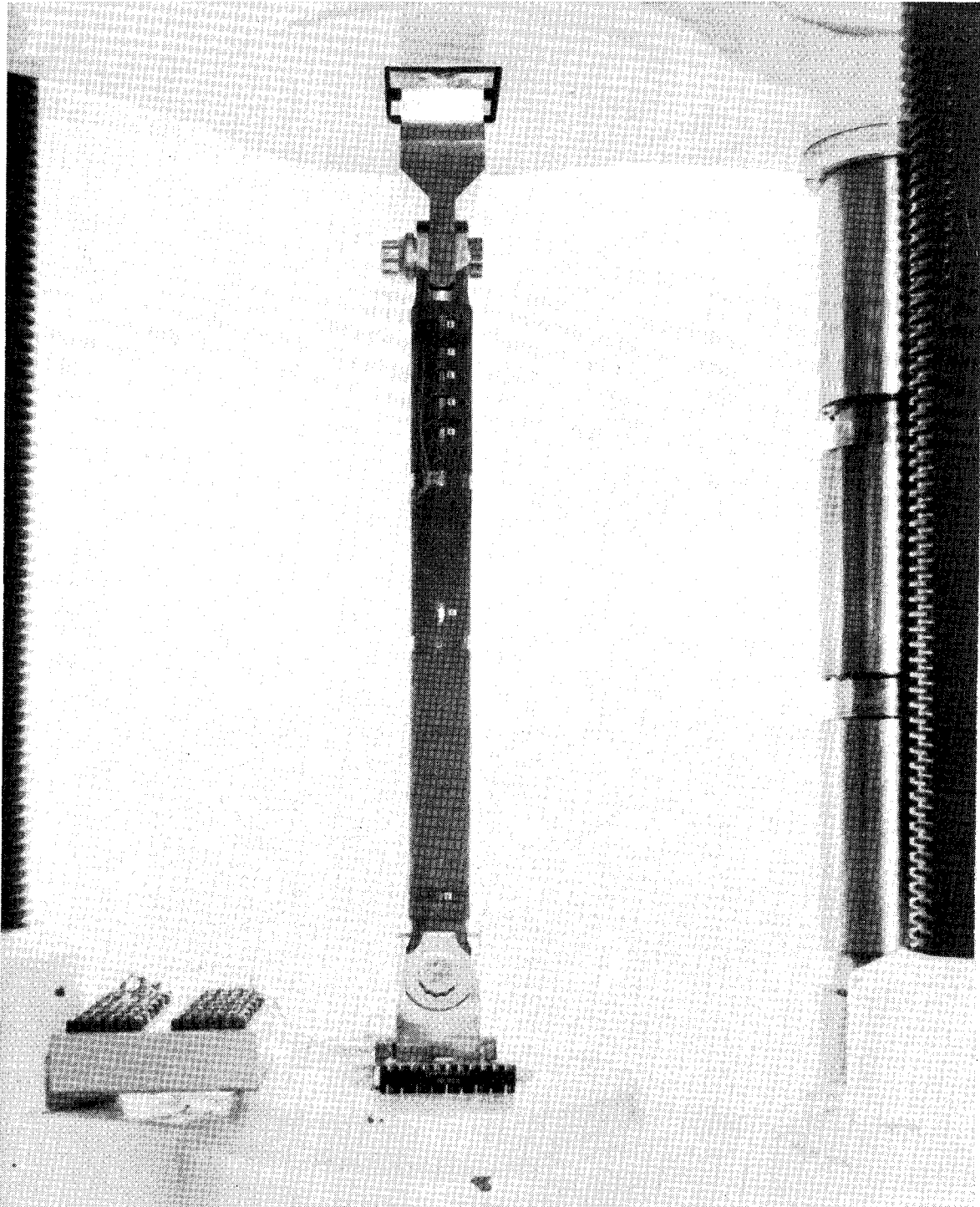
Figure 11.- Tension test setup.
