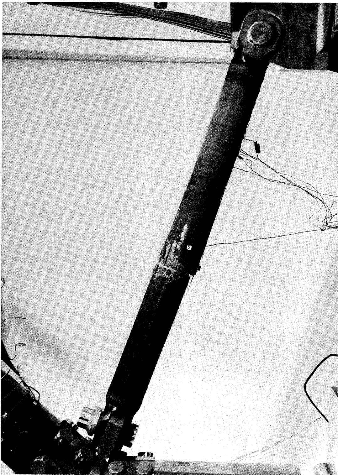
Figure 16.- Failure of demonstration truss.
