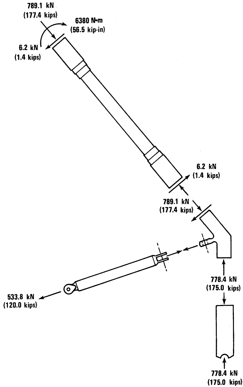
Figure 5.- Internal load distribution.
