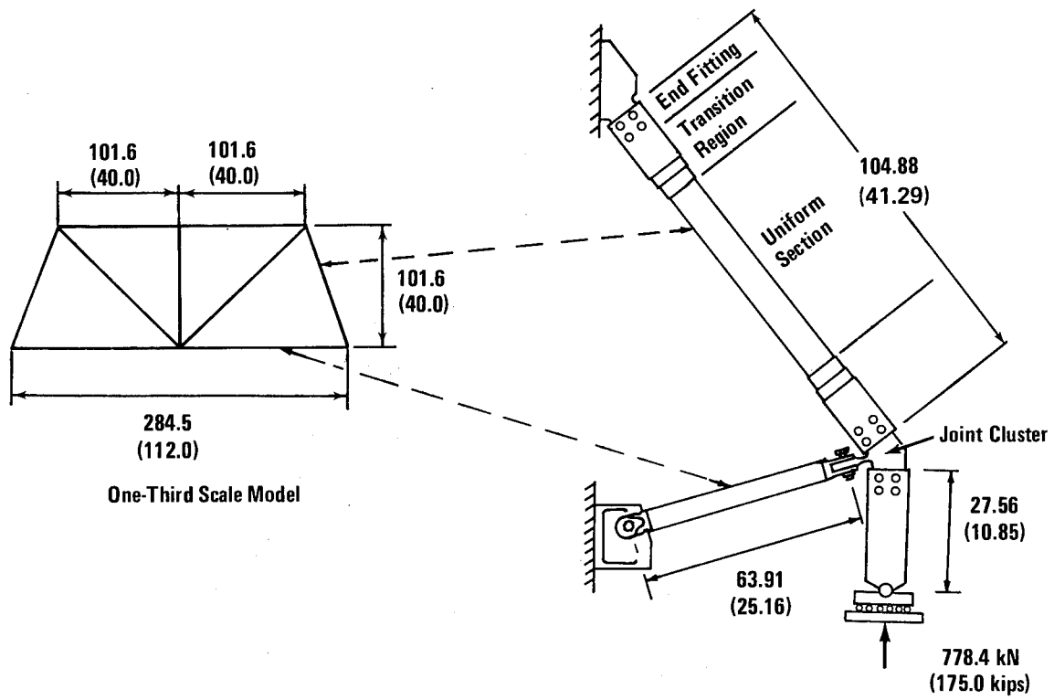
Figure 4.- Demonstration truss. Dimensions are given in centimeters (inches).
