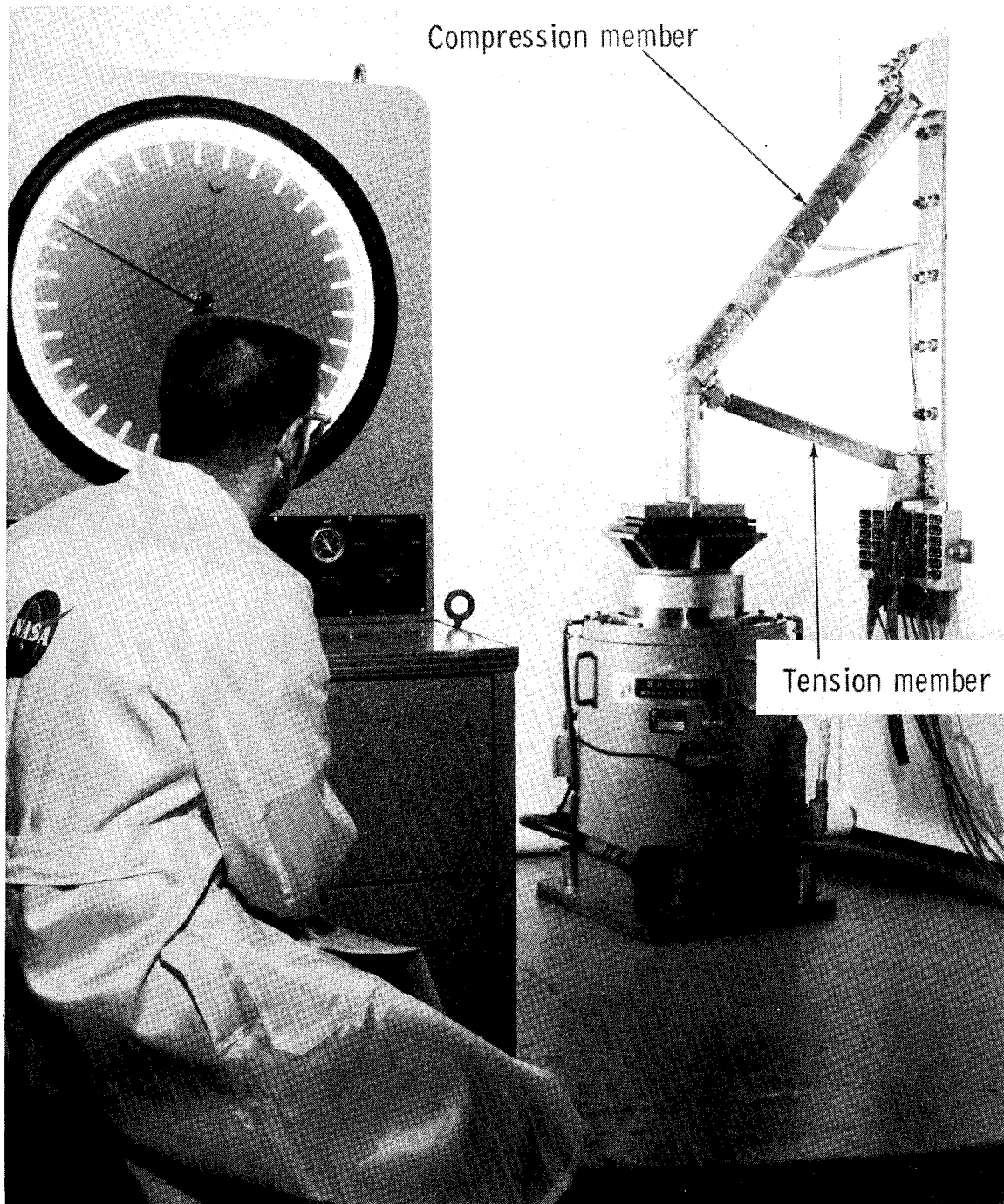
Figure 12.- Demonstration-truss test setup.
