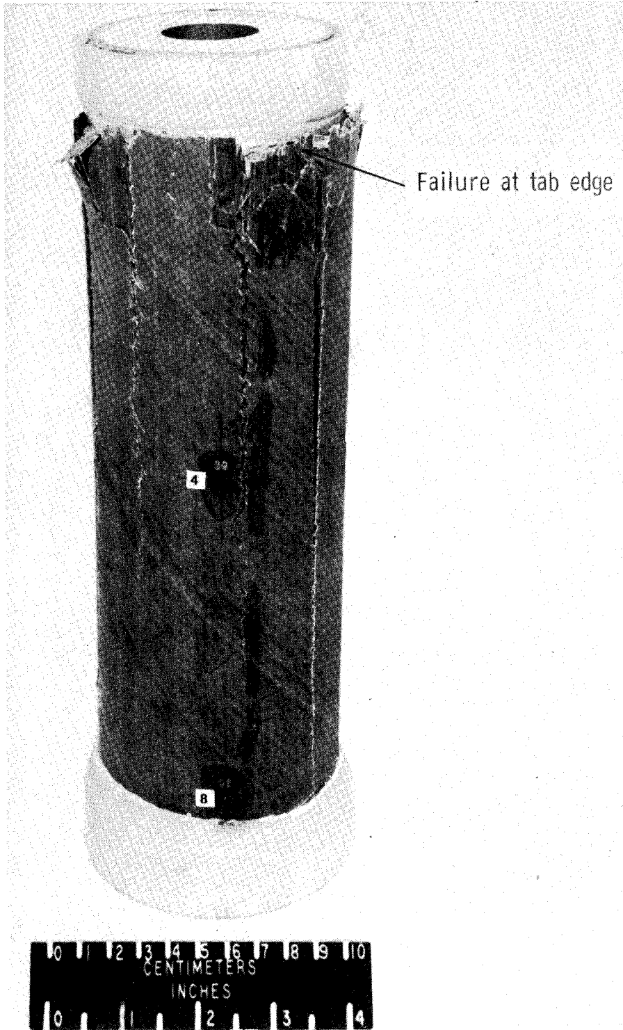
Figure 24.- Failure of local buckling specimen.
