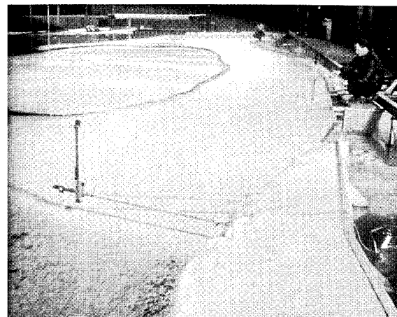
Figure 5. Physical model showing an ice jam formed of particulate material.
