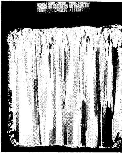
Figure 10. Urea-doped ice thin section showing the thin upper congelation layer and columnar lower layer.
