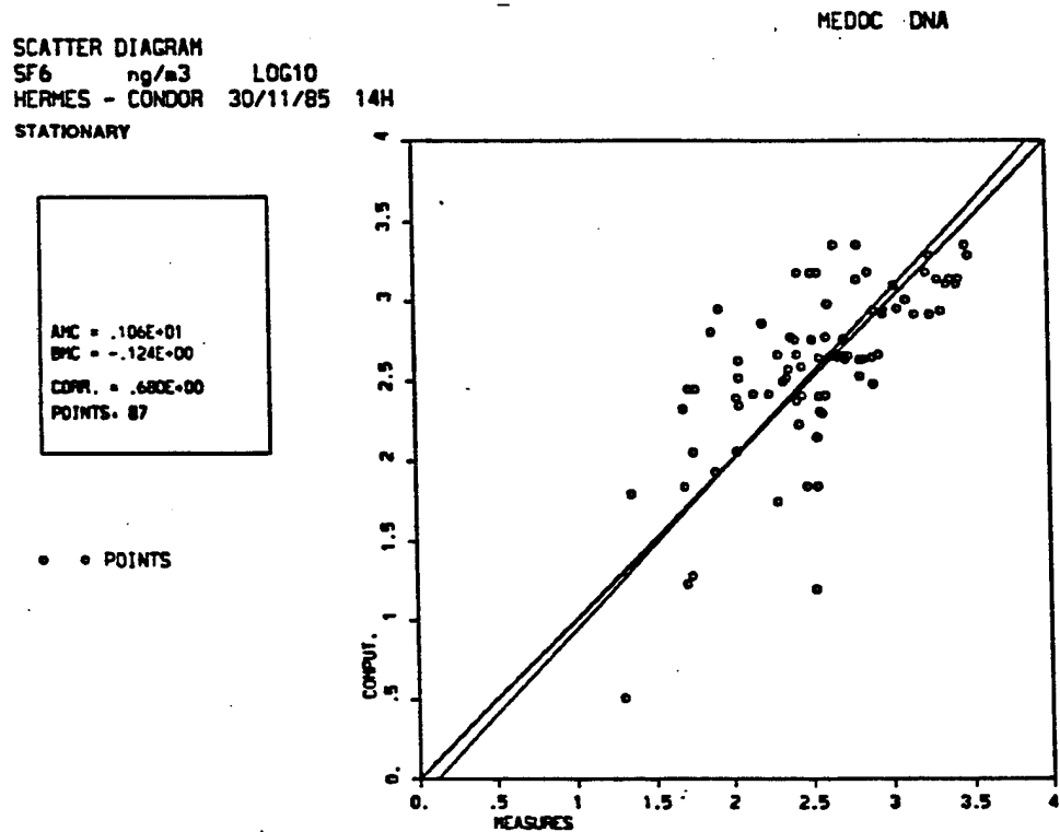
Figure 4-20. Scatter diagram for HERMES/CONDOR calculated concentrations for 30 November SIESTA Experiment.
