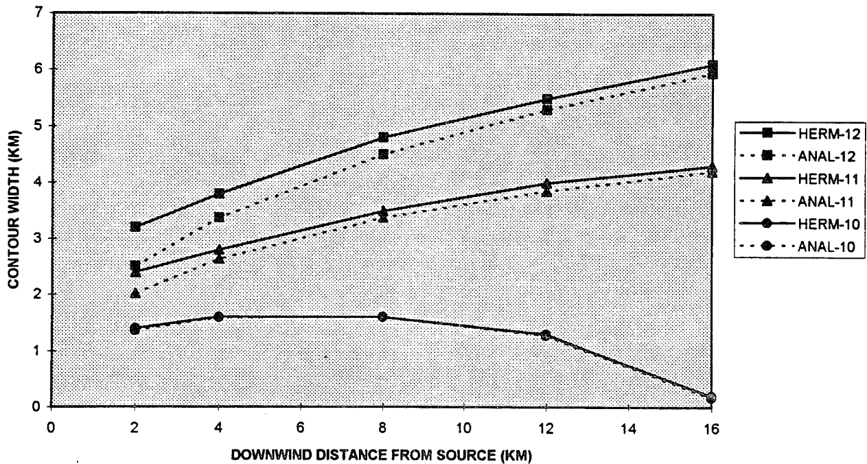
CONTOUR WIDTH VARIATIONS FOR UNSTABLE ATM. (WITH 400 M. HERMES GRID)
