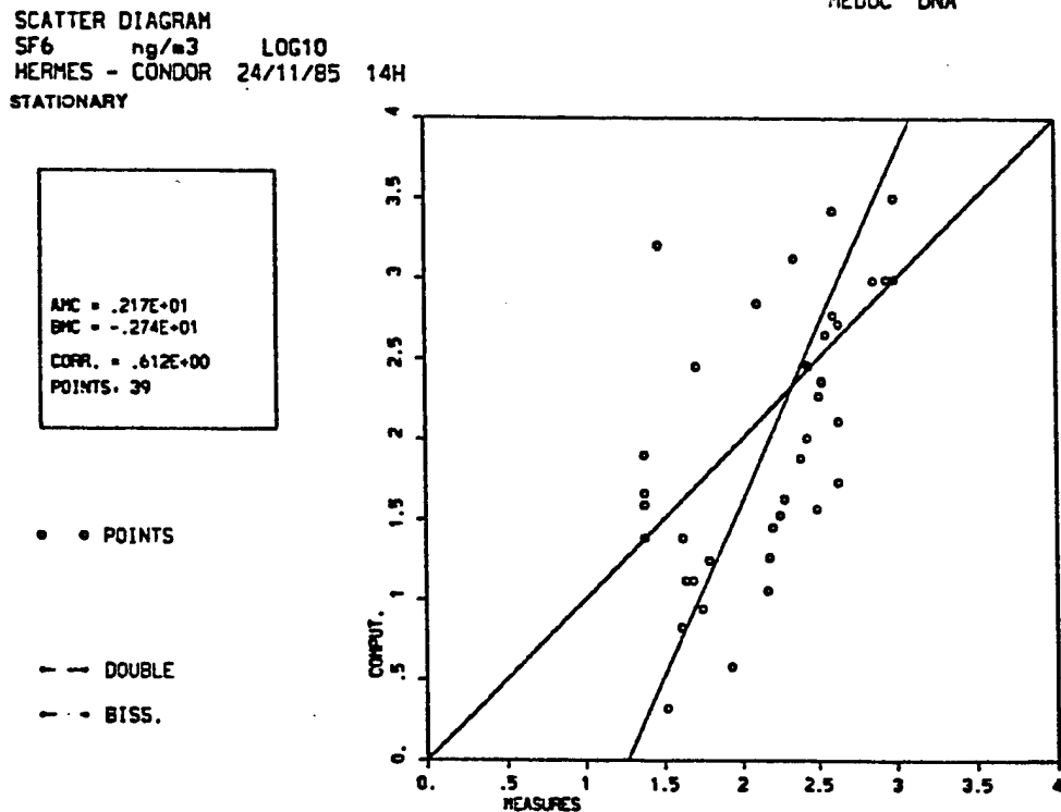
Figure 4-25. Scatter diagram for HERMES calculation with CONDOR winds on 24 November.
