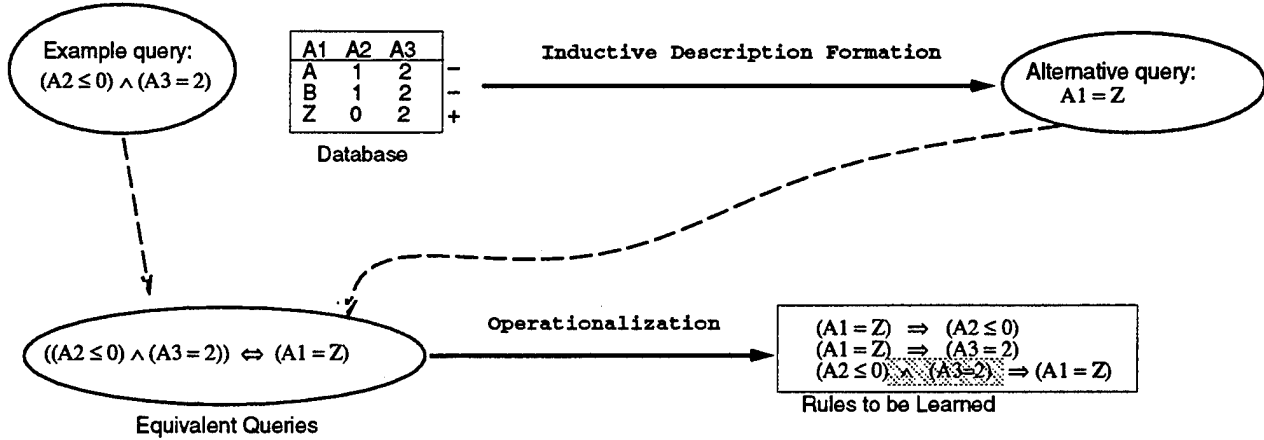
Figure 4: A simplified learning scenario
