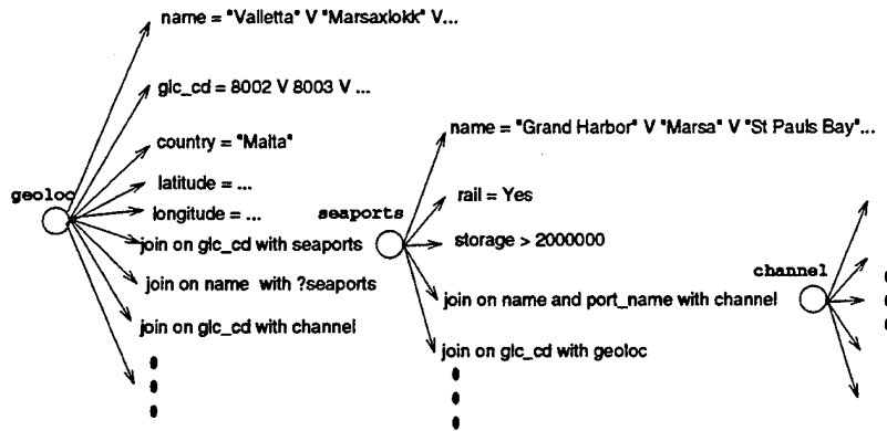
Figure 8: Candidate constraints to be selected
