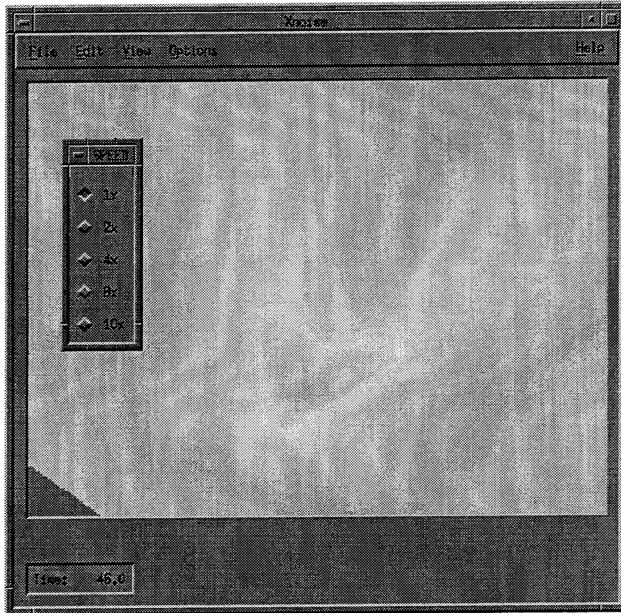
Figure 4.0-17 Speed Dialog
