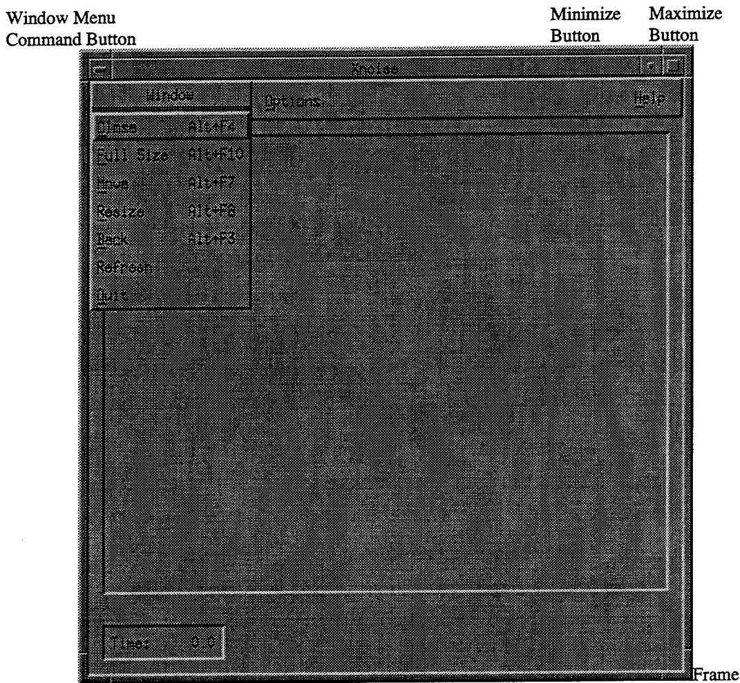
Figure 4.0-2 Window Attributes
