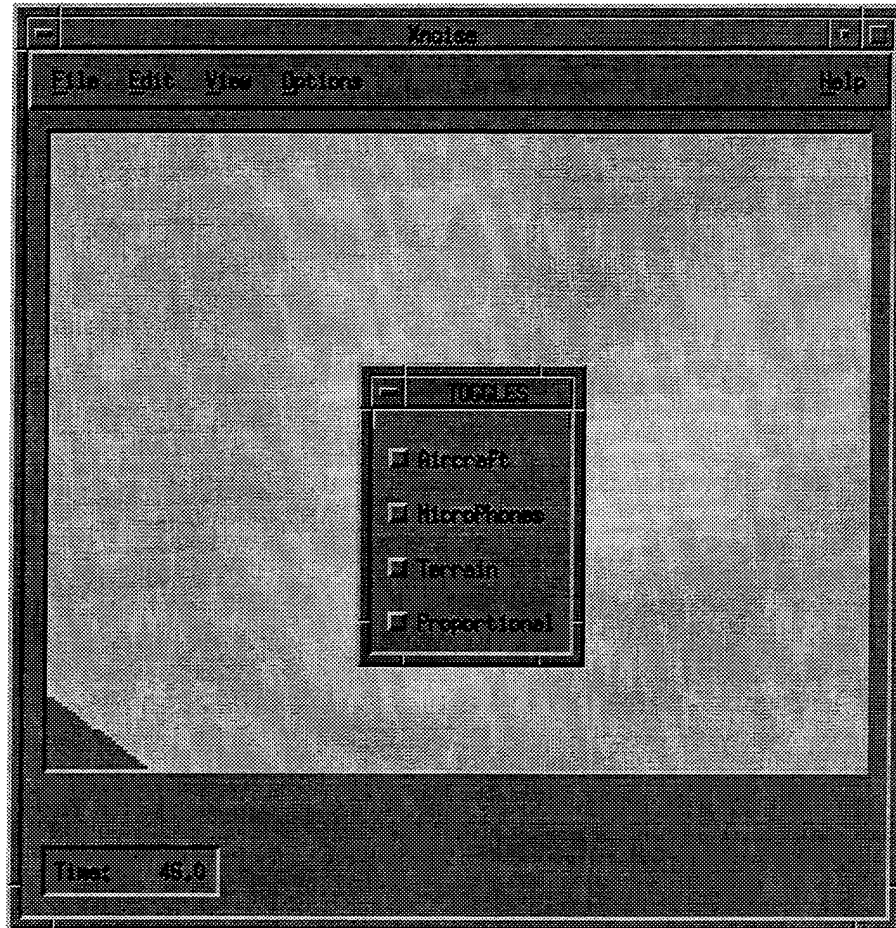
Figure 4.0-18 Toggles Dialog
