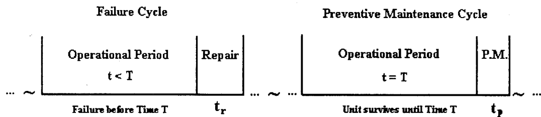
Figure 3.1 Age Replacement Preventive Maintenance Stochastic Process
