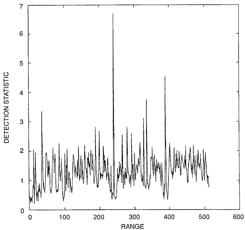
Figure 2. The output of a CFAR processor.
