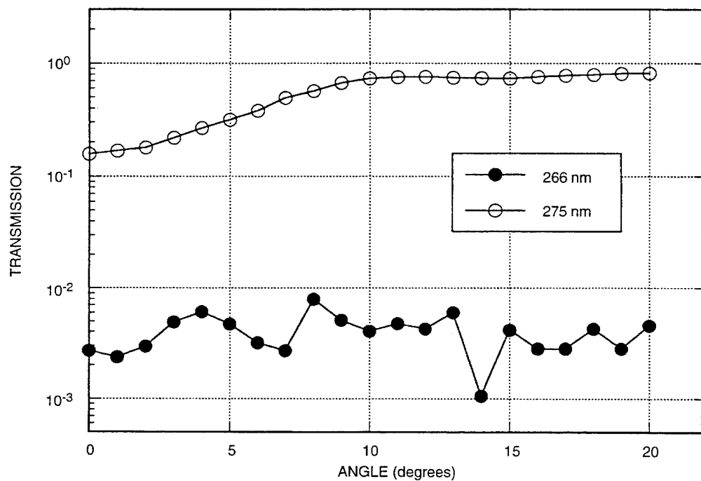
Figure 6. Normalized transmission through 275-nm passing filter for S and P polarization average.
