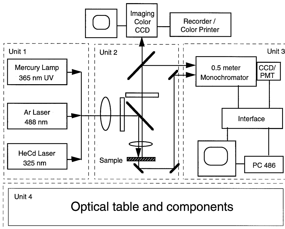
FIGURE 3.5.1 Block diagram of the optical characterization system.
