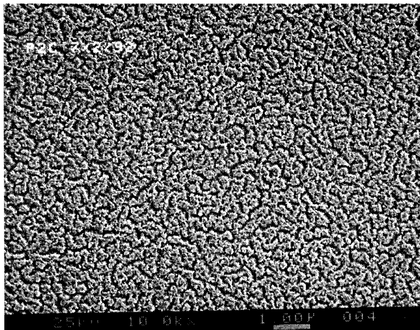
FIGURE 4.1.5(c) SEM micrograph (plan-view) of porous silicon regions of p -Si of 50 \Omega -cm stain-etched for t_j plus \sim 2 min.
