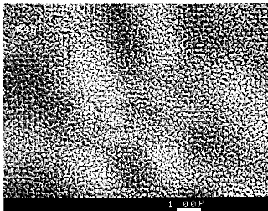
FIGURE 4.1.5(d) SEM micrograph (plan-view) of porous silicon regions of p -Si of 5 \Omega -cm stain-etched for t_j plus \sim 2 min.
