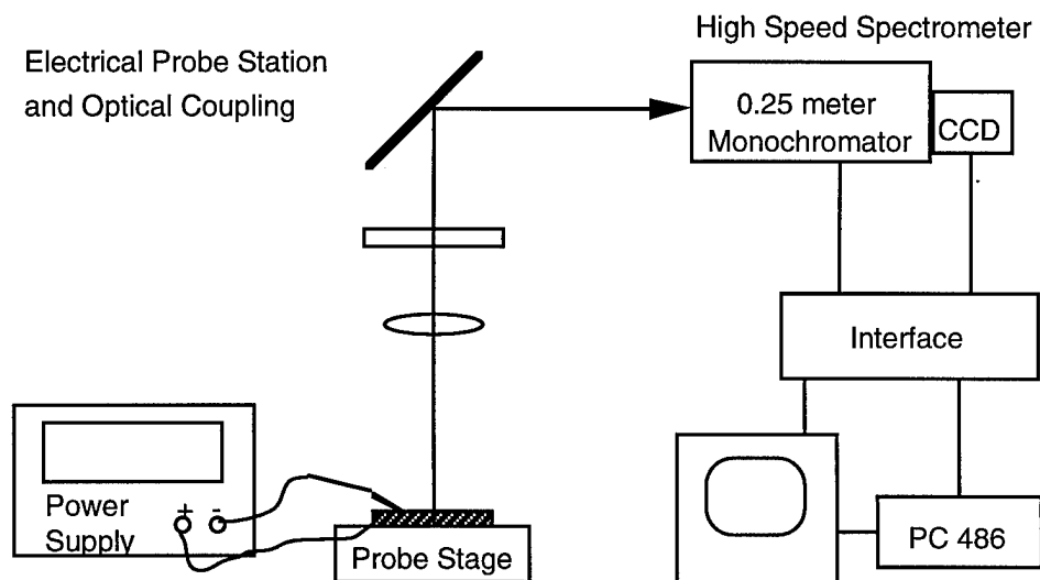
FIGURE 3.6.3 Block diagram of the electroluminescence characterization system.
