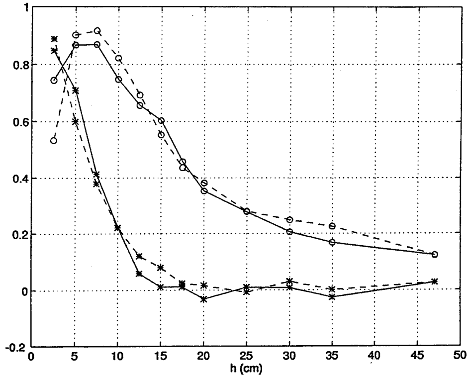
Figure 3: Comparison of skewness (o) and asymmetry (*) at different water depths. Solid lines is experimental data (Mase and Kirby, 1992). Dashed line is numerical result.
