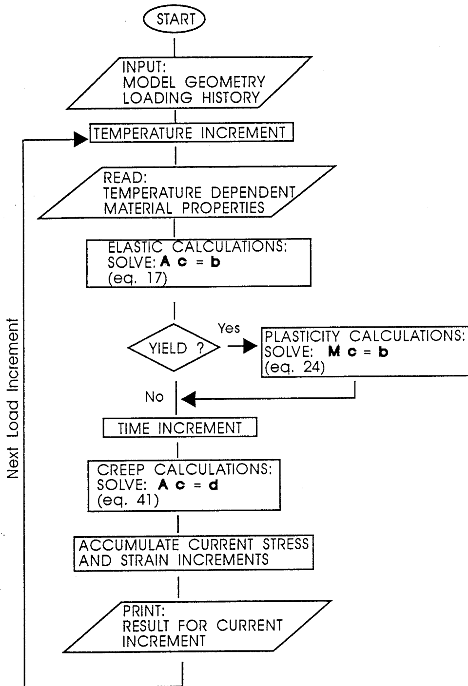
Fig. 3-4 Flow charts for elastic-plastic-creep algorithm.
