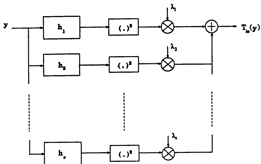
Figure 72 Block diagram of the processor for generating -th decision statistic.
