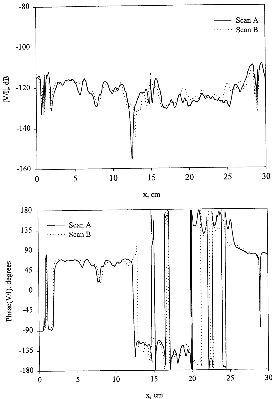
Figure 98 . Magnitude and phase of the response of the D-type probe as a function of position for scans A and B when the flaw is a 0.34 mm diameter hole and f = 1 kHz.
