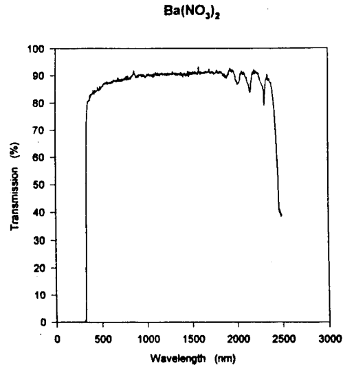
Figure 1: Transmission vs. wavelength for 3 mm pathlength Ba(NO_3)_2 crystal.
