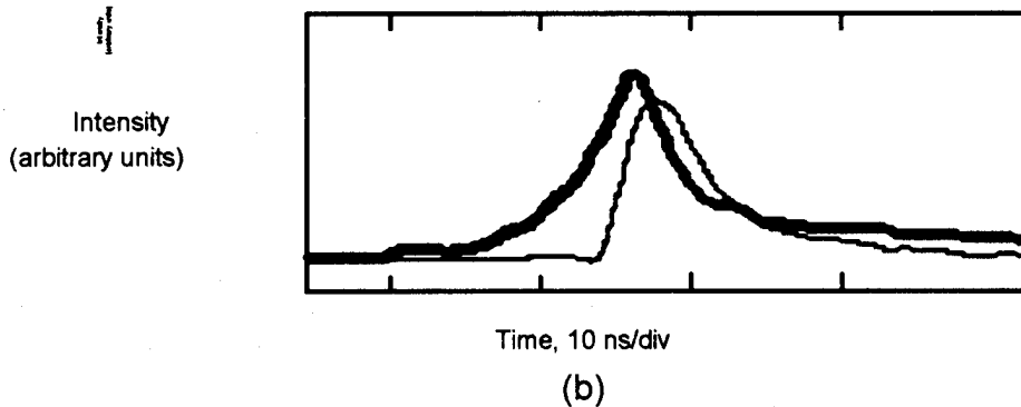
Figure 20: (a) Modeling of the pump depletion and Raman emission. The maximum 1.3 \mu\text{m} output of the Nd:YAG laser without the Raman conversion would correspond to 25 \text{ mJ/pulse} . The slower risetime curve is the 1.3 \mu\text{m} pump pulse and the delayed, rapidly rising pulse is the first Stokes output at 1.5 \mu\text{m} . The result shows the well defined Raman threshold, pump depletion and high Raman gain. (b) oscilloscope trace of the temporal profile of pump and Raman emission. Pump is dark solid line and Raman output is thin solid line.
