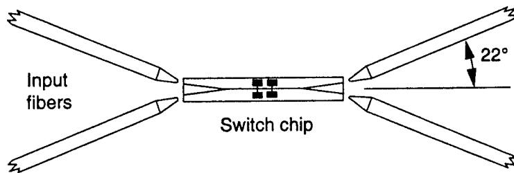
Figure 7. The 2x2 optical switch has on-chip input and output waveguides angled at \mathcal{T} to the facet to minimize reflections. Refraction produces entrance and exit angles of about 22^\circ .
