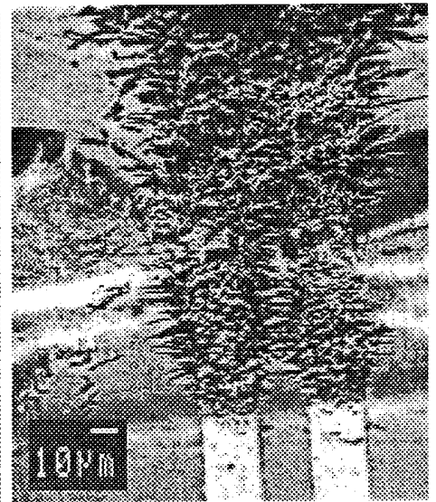
figure 2b SEM of Au CPS TL after overgrowth by LT GaAs and anneal at 600°C
