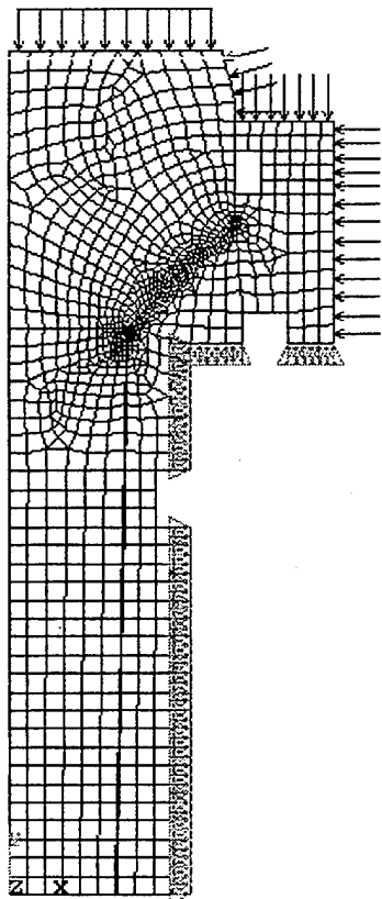
Figure 35. NRaD acrylic wide angle light pipe (w/o stem) maximum principal stress contours at 1000 psi (low-pressure face edge detail).
