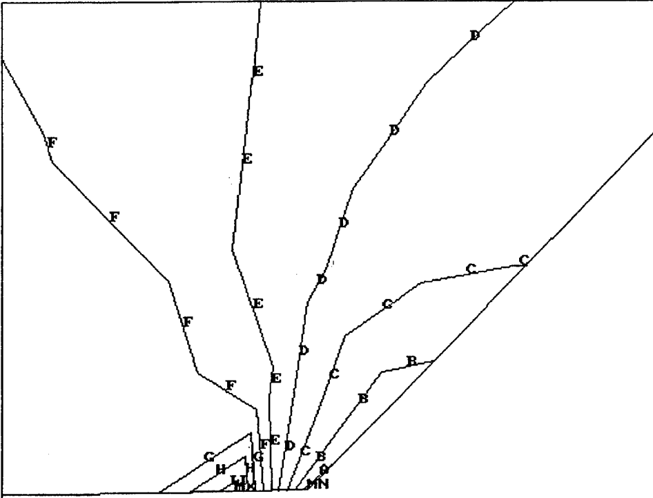
Figure 31. Acrylic conical frustum window ( t/D_i = 0.5 ) maximum principal stress contours at 1000 psi (low-pressure face edge detail).
