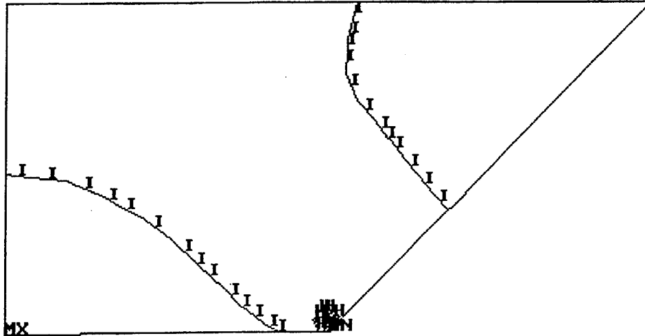
Figure 29. Acrylic conical frustum window ( t/D_i = 0.5 ) minimum principal stress contours at 1000 psi.
