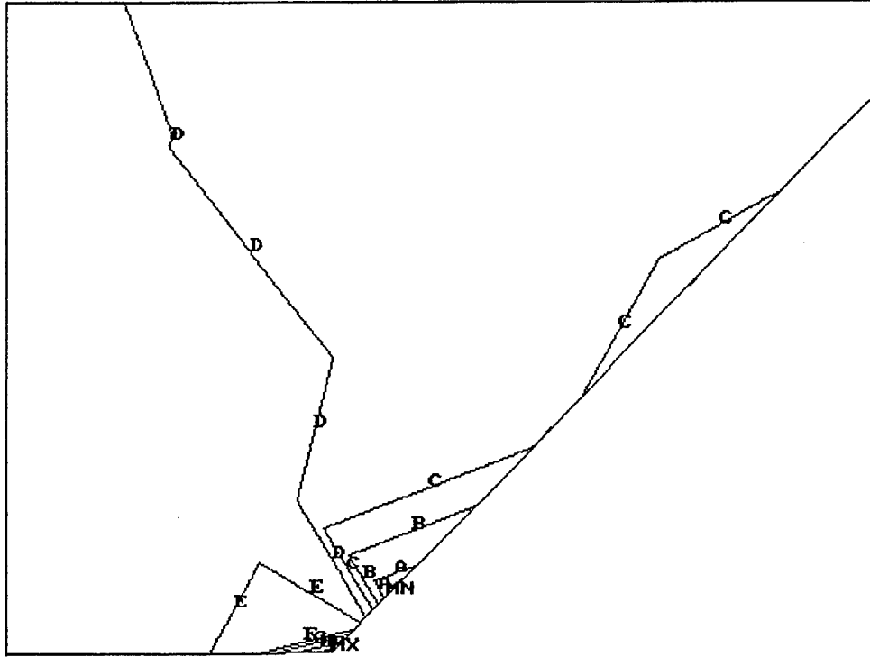
Figure 35. NRaD acrylic wide angle light pipe (w/o stem) maximum principal stress contours at 1000 psi (low-pressure face edge detail).
