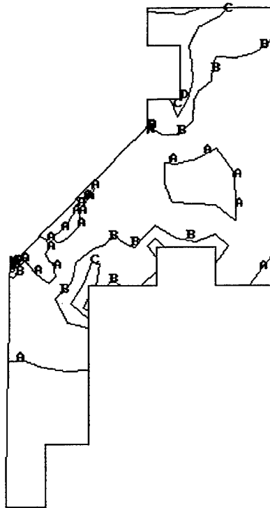
Figure 40. NRaD CRES adapter equivalent stress contours at 1000 psi.
