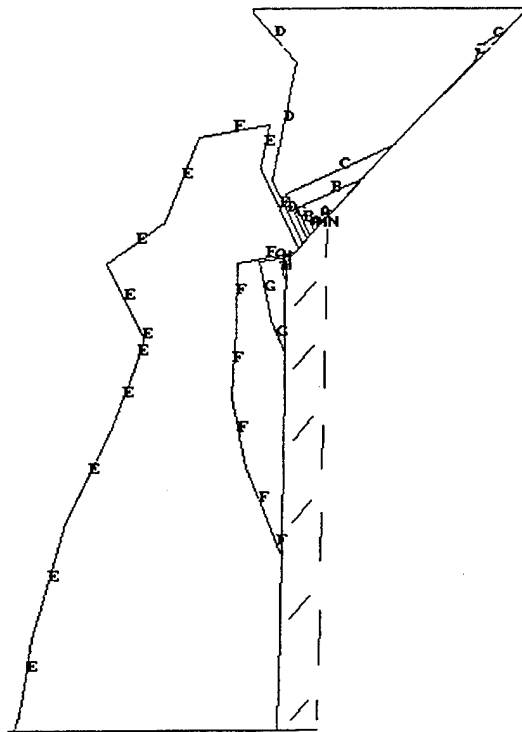
Figure 39. NRaD acrylic wide angle light pipe maximum principal stress contours at 1000 psi (stem/head junction detail).
