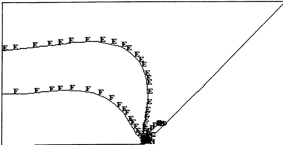
Figure 30. Acrylic conical frustum window ( t/D_i = 0.5 ) maximum principal stress contours at 1000 psi.
