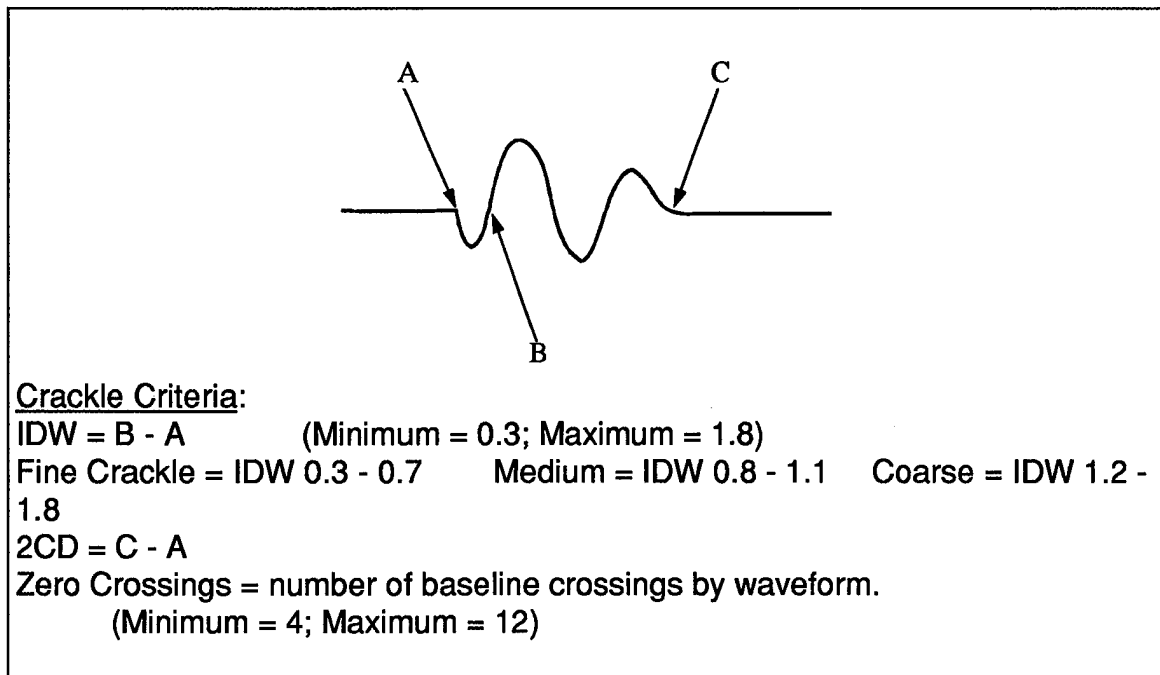
Figure 7. Typical crackle waveform and measurement
