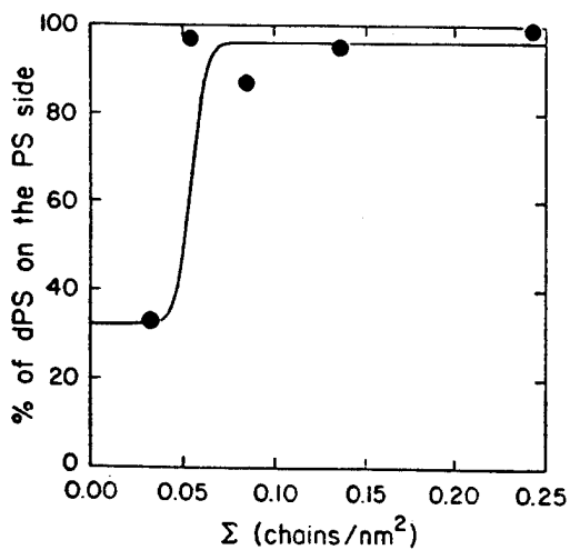
Figure 6: a.) Interfacial fracture energy of glass-PS interfaces modified by a 680-95 dPS-PVP block copolymer. b.) and c.) percentage of dPS on the PS and PVP on the glass sides of the fracture surface, respectively.
