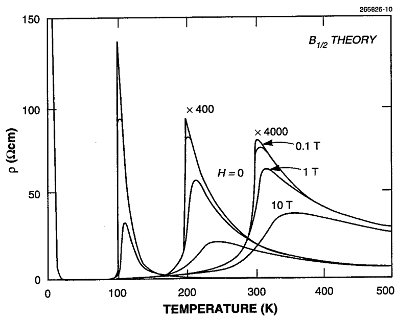
Figure 12. Predicted plots of \rho versus T by the B_{1/2} approximation for T_C values of 100, 200, and 300 K. Magnetic field strengths are H = 0, 0.1, 1 , and 10 T.
