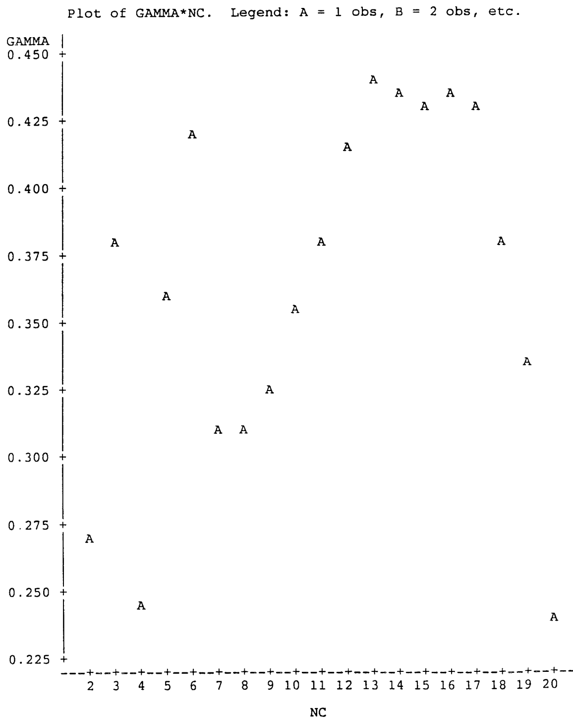
Figure 2. Gamma by Number of Clusters
