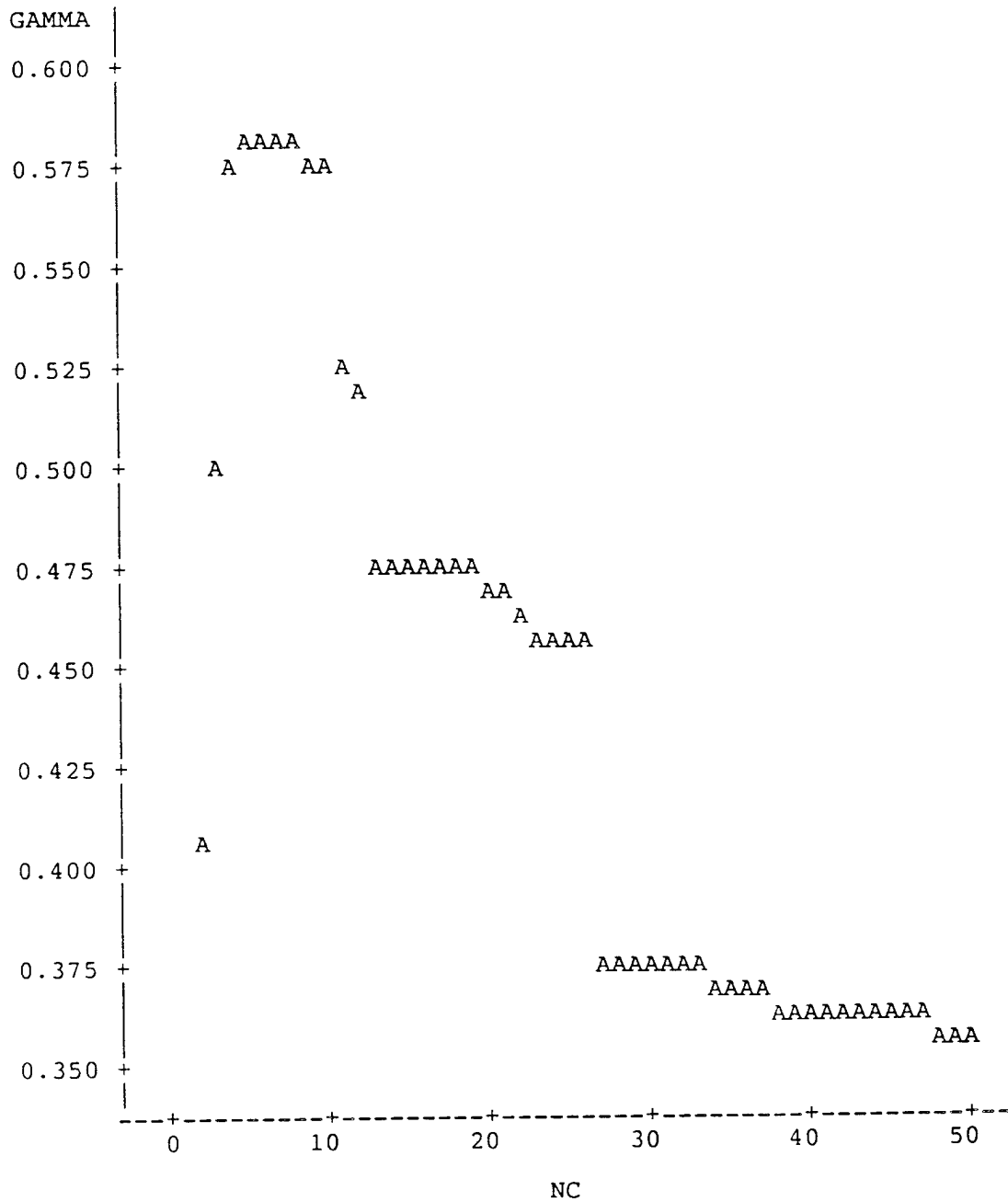
Figure 2. Gamma by Number of Clusters
