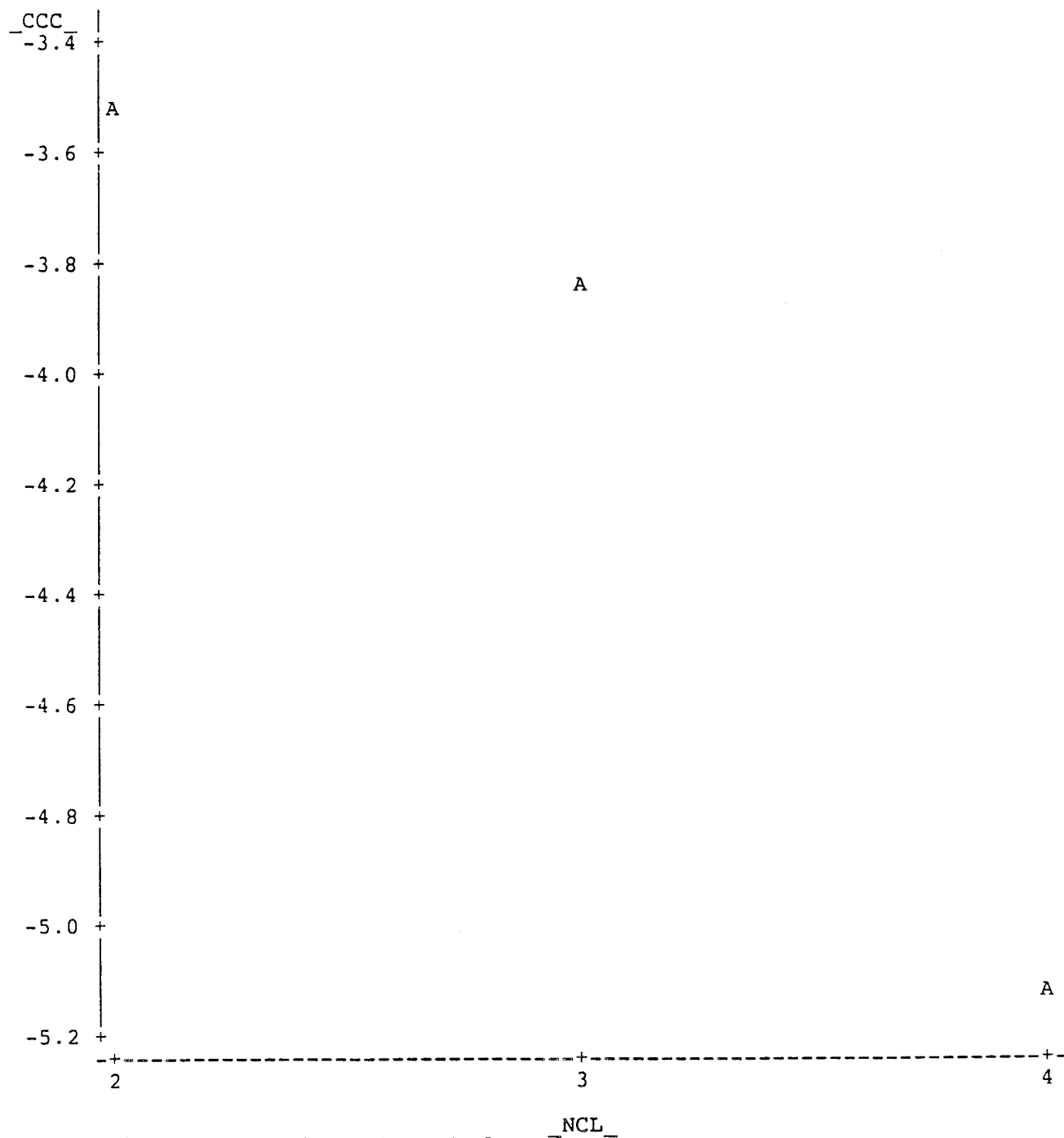
Figure 1. CCC by Number of Clusters
