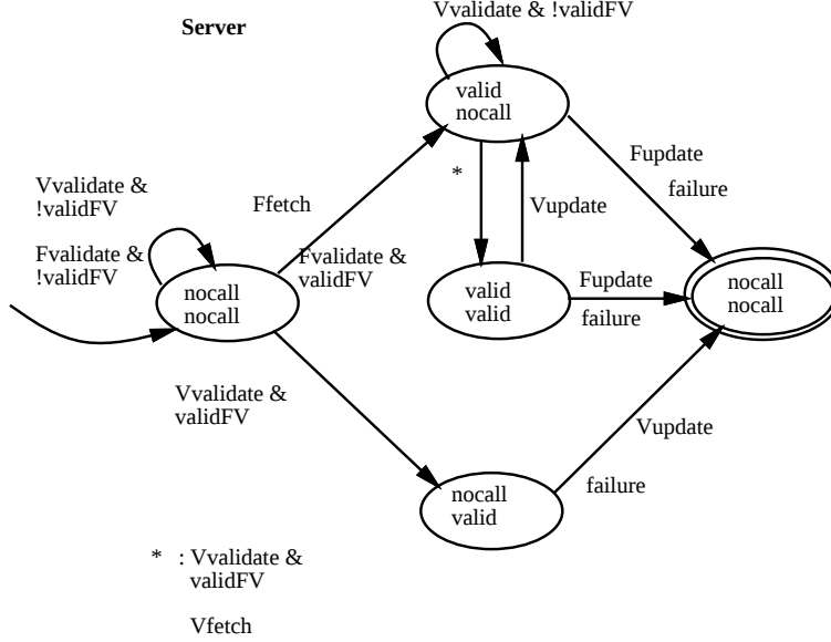
Figure 10: State Transition Diagram for Coda+ Server
