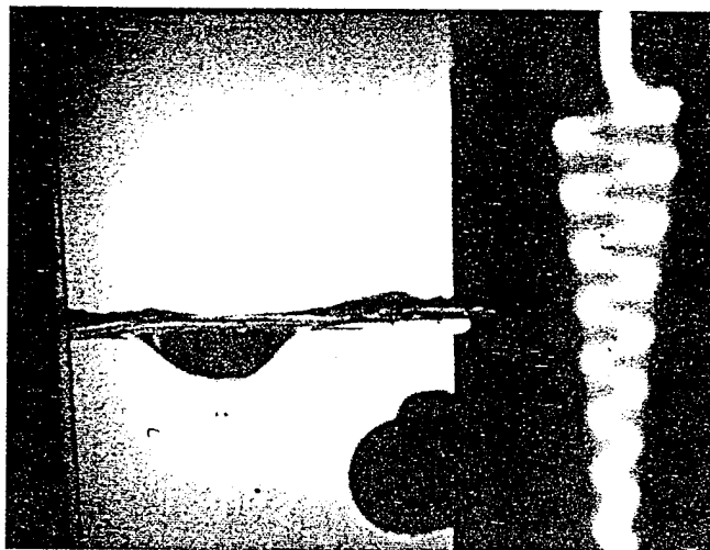
FIG. 1. A frame from a high-speed cinematographic sequence showing the entrapment of an air bubble when a drop hits a liquid surface (courtesy of H. C. Pumphrey and L. A. Crum). The left half of the frame shows the physical event. One can see the free surface indented by the crater caused by the impact and, directly under it, the bubble that has just detached. The shadow in the lower right is a hydrophone that drives an oscilloscope the trace of which is shown, vertically, in the right half of the frame. The right half of the picture shows therefore, in a sense, the "soundtrack" of the left half. The damped sinusoid of the oscilloscope trace is the acoustic signal produced by the volume oscillations of the bubble. A study of the angular distribution of the signal reveals the expected dipole pattern. See Refs. 3-5 for further details.
