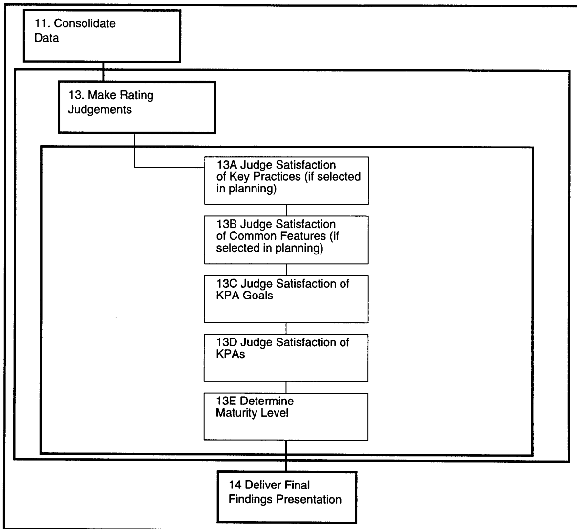
Figure 3-14: Make Rating Judgments Activity Diagram
