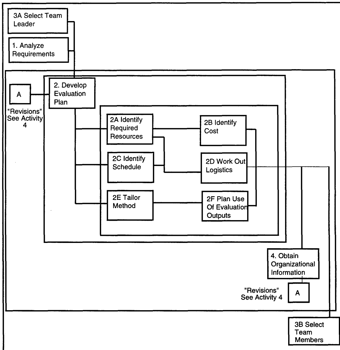
Figure 3-3: Develop Evaluation Plan Activity Diagram
