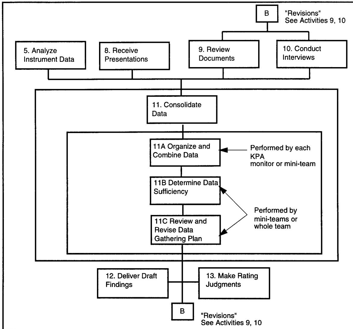
Figure 3-12: Consolidate Data Activity Diagram
