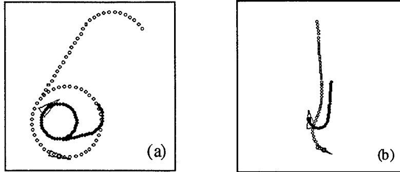
Figure 2 (a) Demonstration of the ability of the plane to survive indefinitely by flying in continuous circles within the missile's turn radius. (b) Demonstration of the learned behavior of the plane to turn toward the missile to increase the distance between the two in the long term.
