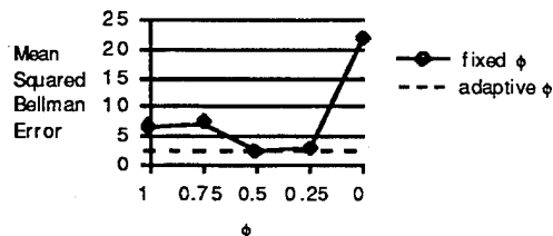
Figure 4: The use of an adaptive \phi reduced the mean squared Bellman residual further than any of the tested fixed \phi 's.
