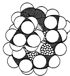
( S,S )-6a
