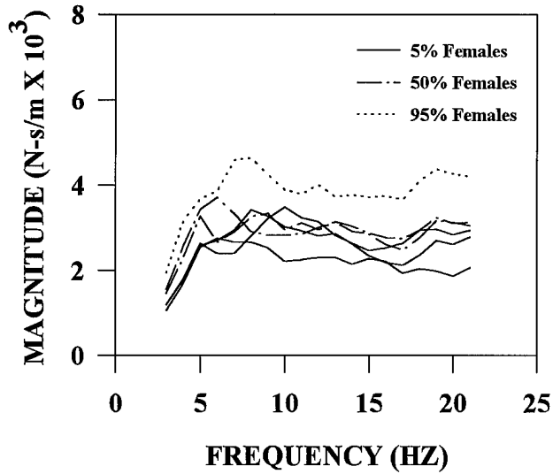
IMPEDANCE VS FREQUENCY Females, Rigid Seat, 0.59 \text{ m/s}^2 \text{ rms}
