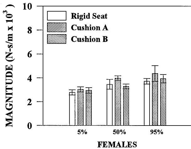
Figure 8 Primary Peak Impedance Magnitude Means +/- One Standard Deviation - Seat Configuration Effects
