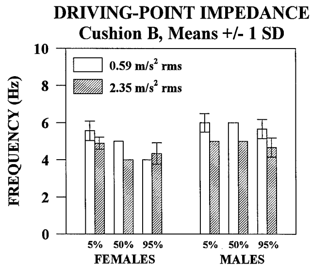
Figure 4 Primary Impedance Resonance Frequency Means +/- One Standard Deviation
