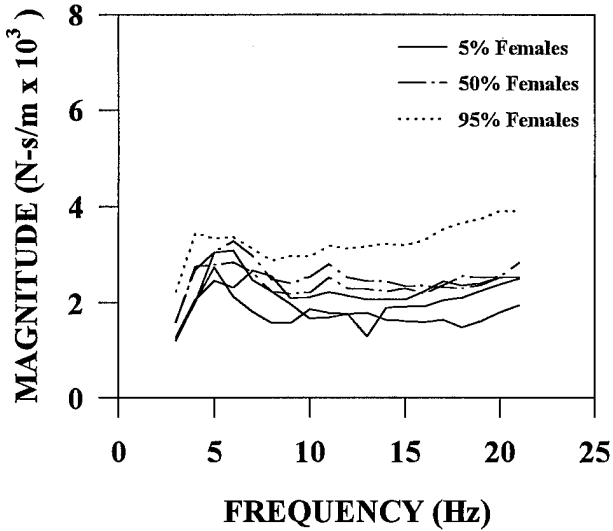
IMPEDANCE VS FREQUENCY Females, Rigid Seat, 2.35 \text{ m/s}^2 \text{ rms}
