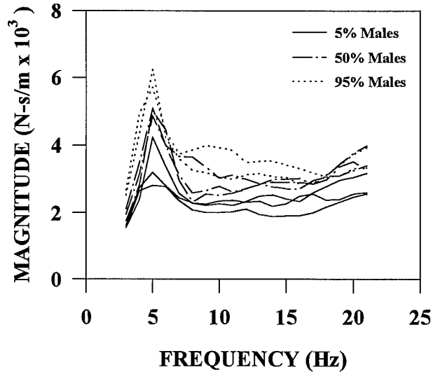
IMPEDANCE VS FREQUENCY Males, Rigid Seat, 2.35 \text{ m/s}^2 \text{ rms}
