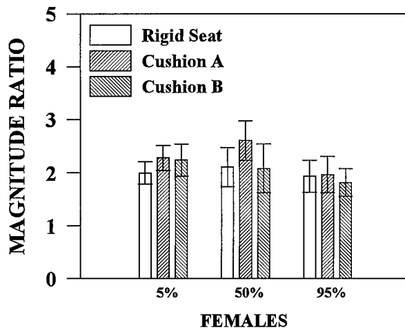
Figure 21 Primary Peak Vertical (Z) Head Transmissibility Means \pm One Standard Deviation - Seat Configuration Effects
