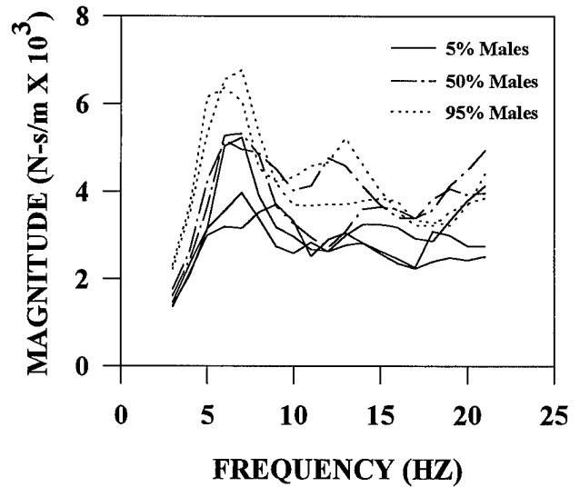
IMPEDANCE VS FREQUENCY Males, Rigid Seat, 0.59 \text{ m/s}^2 \text{ rms}
