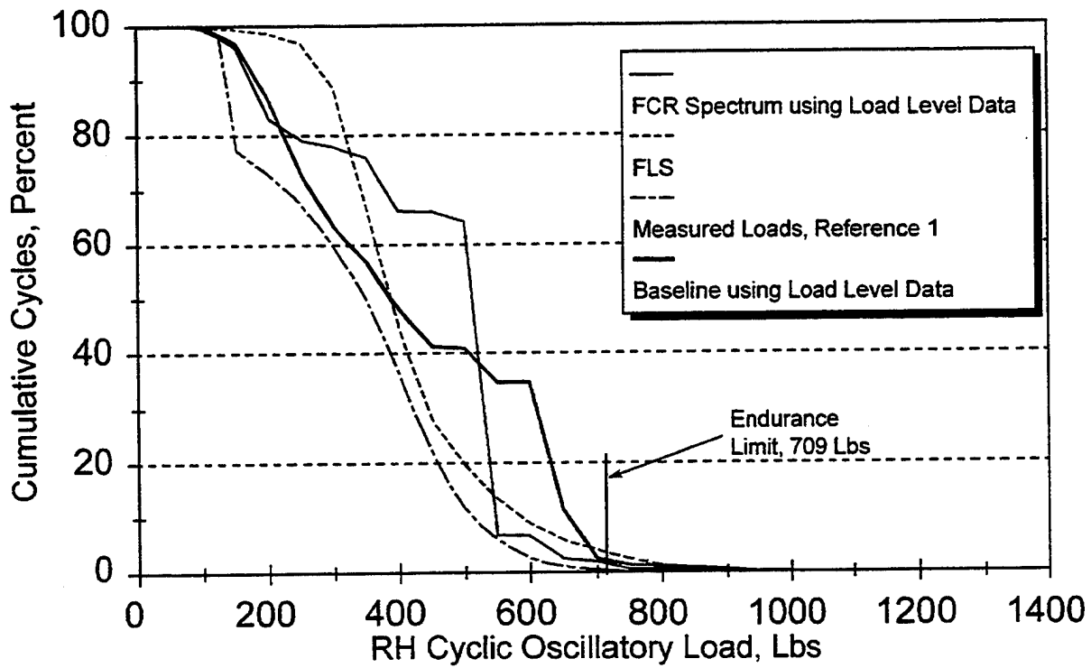
SD470 Figure 27. Cumulative Cycles vs Oscillatory Load - Swashplate Inner Ring
