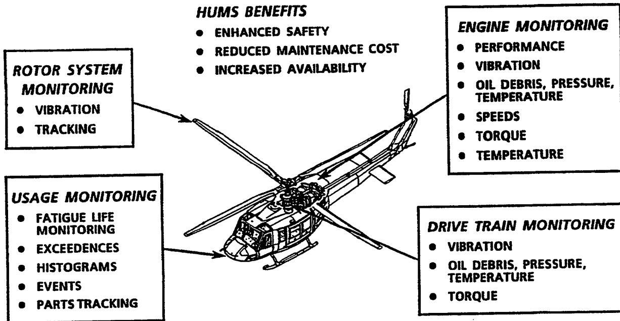
Figure 2. HUMS Functions
