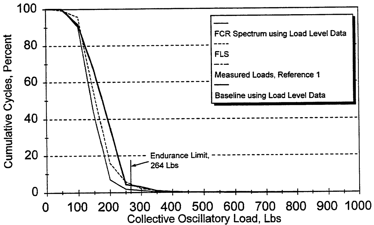
SD471 Figure 28. Cumulative Cycles vs Oscillatory Load - Collective Lever
