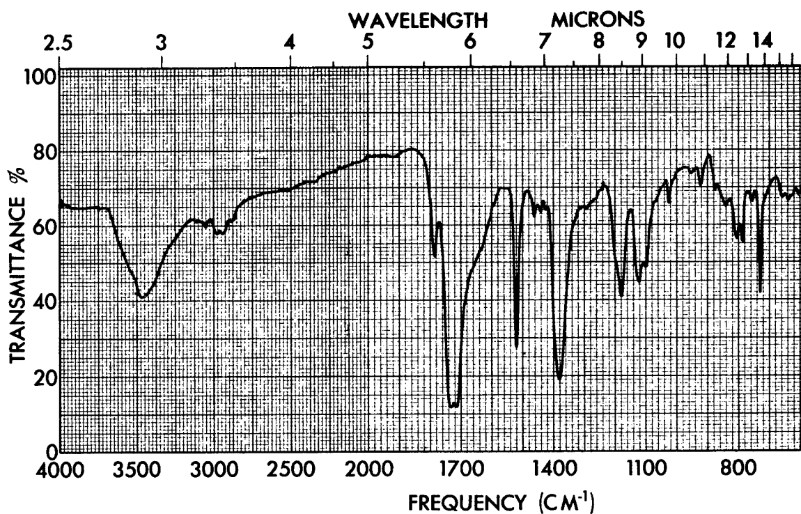
Figure C.1. Infrared Spectrum of 1150 FMW MN/MDA/PMDA Imidized Prepolymer Powder (KBr) Concentration: 3.3 mg/g KBr
