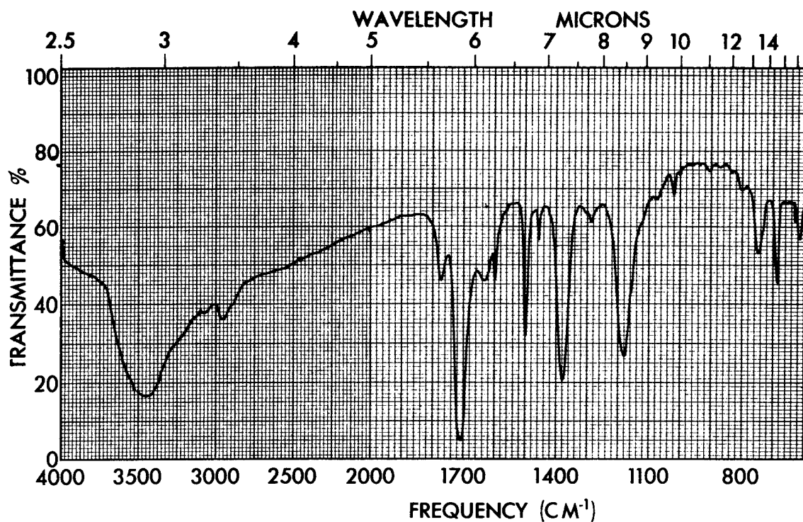
Figure B.1. Infrared Spectrum of Pyrolysis Residue I-589-1-V (KBr) Concentration: 3.3 mg/g KBr
