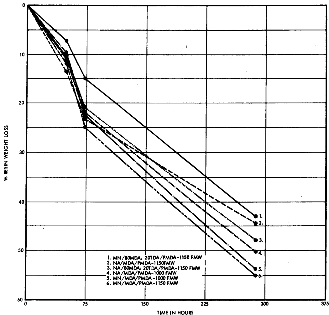
Figure 19. Plot of Resin Weight Loss as a Function of Isothermal Aging at 616°K in Air (100 cm 3 /min. flow).
