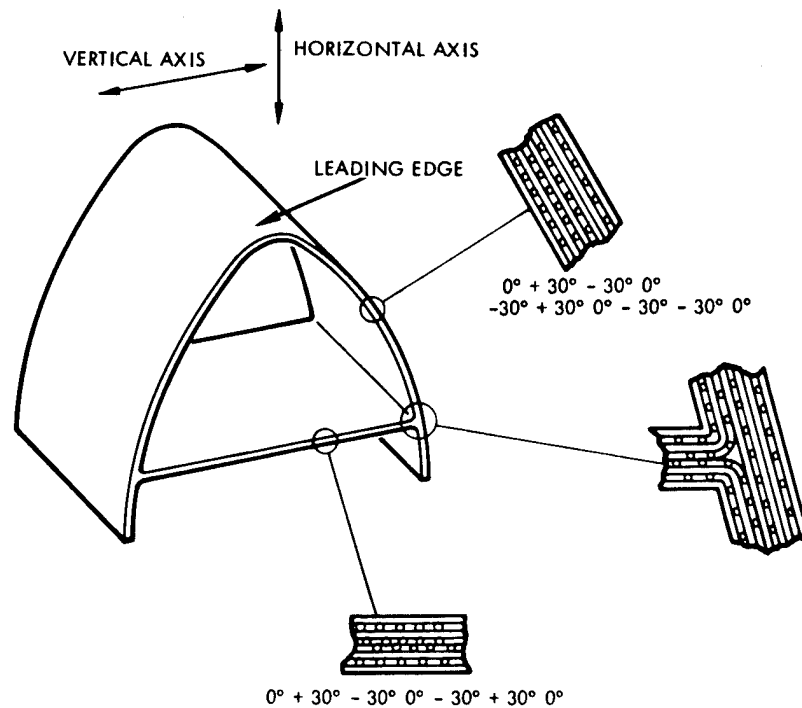
Figure 31. Demonstration Component
