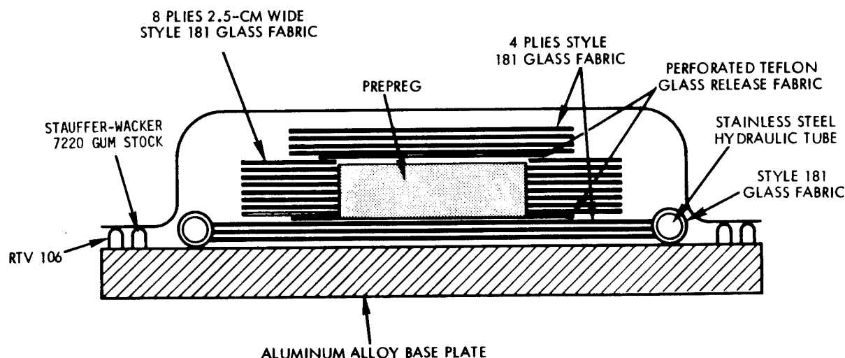
Figure 29. Schematic of Bagging System
