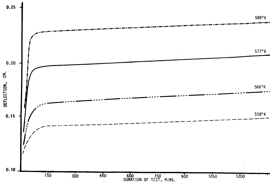
Figure 17. Flexural Creep vs Time at 50% Stress Level
