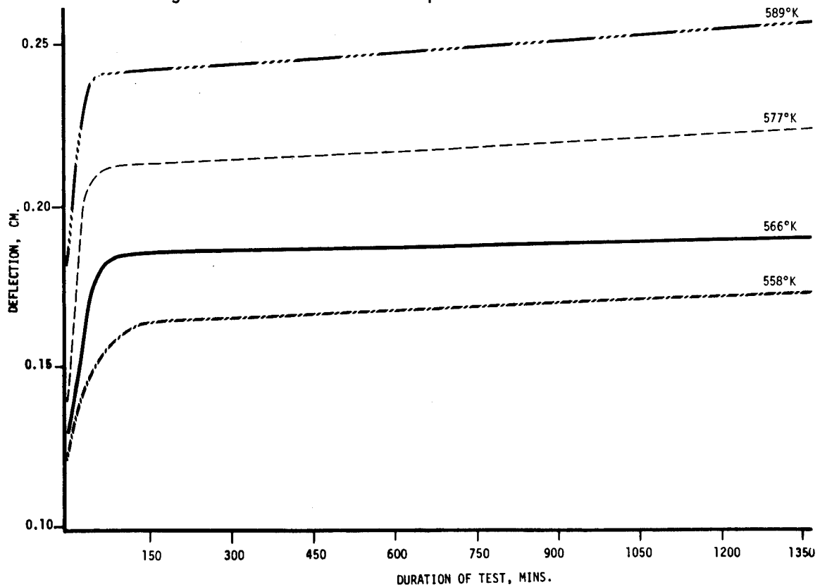
Figure 18. Flexural Creep vs Time at 75% Stress Level
