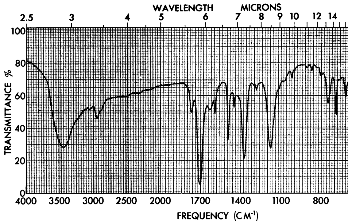
Figure B.4. Infrared Spectrum of Pyrolysis Residue I/II-589-2-P (KBr) Concentration: 3.3 mg/g KBr
