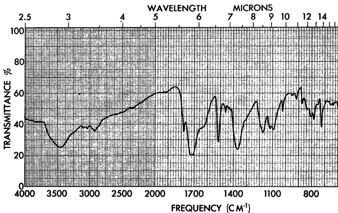
Figure C.2. Infrared Spectrum of 1150 FMW MN/MDA/PMDA Cured Polymer (KBr) Concentration: 6.6 mg/g KBr
