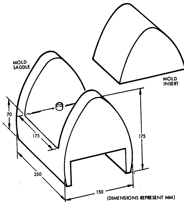
Figure 32. Lay-up Mold Design
