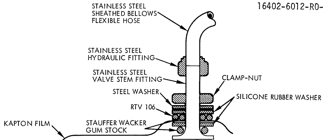
Figure 35. Schematic of Valve Stem Vacuum Hose Connector
