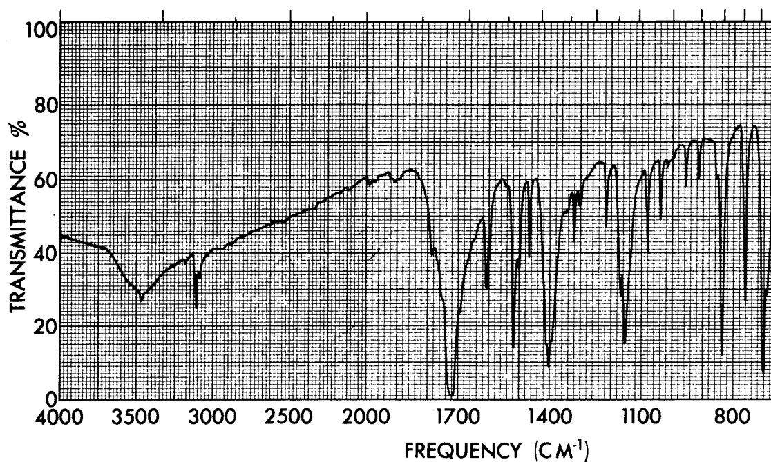
Figure A.2. Infrared Spectrum of N-Phenyl Maleimide (KBr) Concentration: 3.7 mg/g KBr
