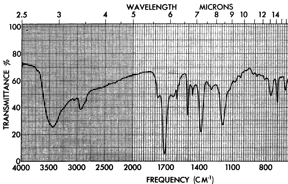
Figure B.2. Infrared Spectrum of Pyrolysis Residue I-589-2-P (KBr) Concentration: 3.3 mg/g KBr
