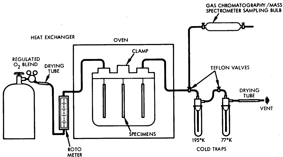
Figure 11. Aging Apparatus For Unstressed Specimens
