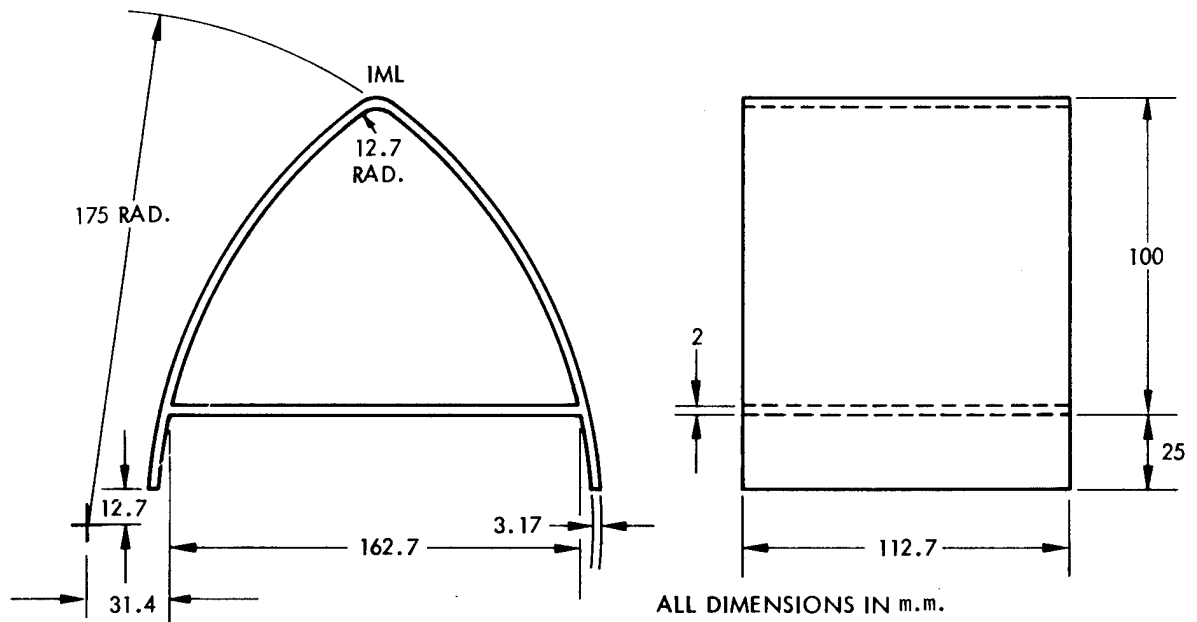
Figure 30. Graphite Composite, Autoclave Molded, Demonstration Component
