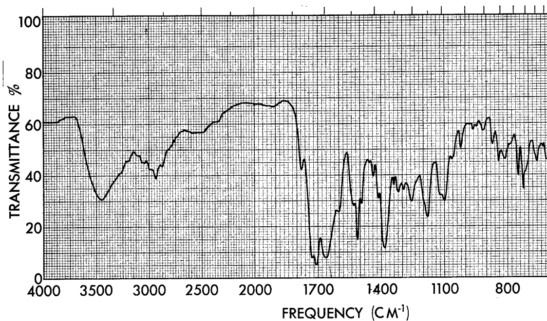
Figure 25. Infrared Spectrum of 1000 FMW NA/80MDA:20TDA/PMDA Resin Removed from Opaque Glass Prepreg Heated to <311^{\circ}\text{K} (KBr) Concentration: 3.9 mg/g KBr
