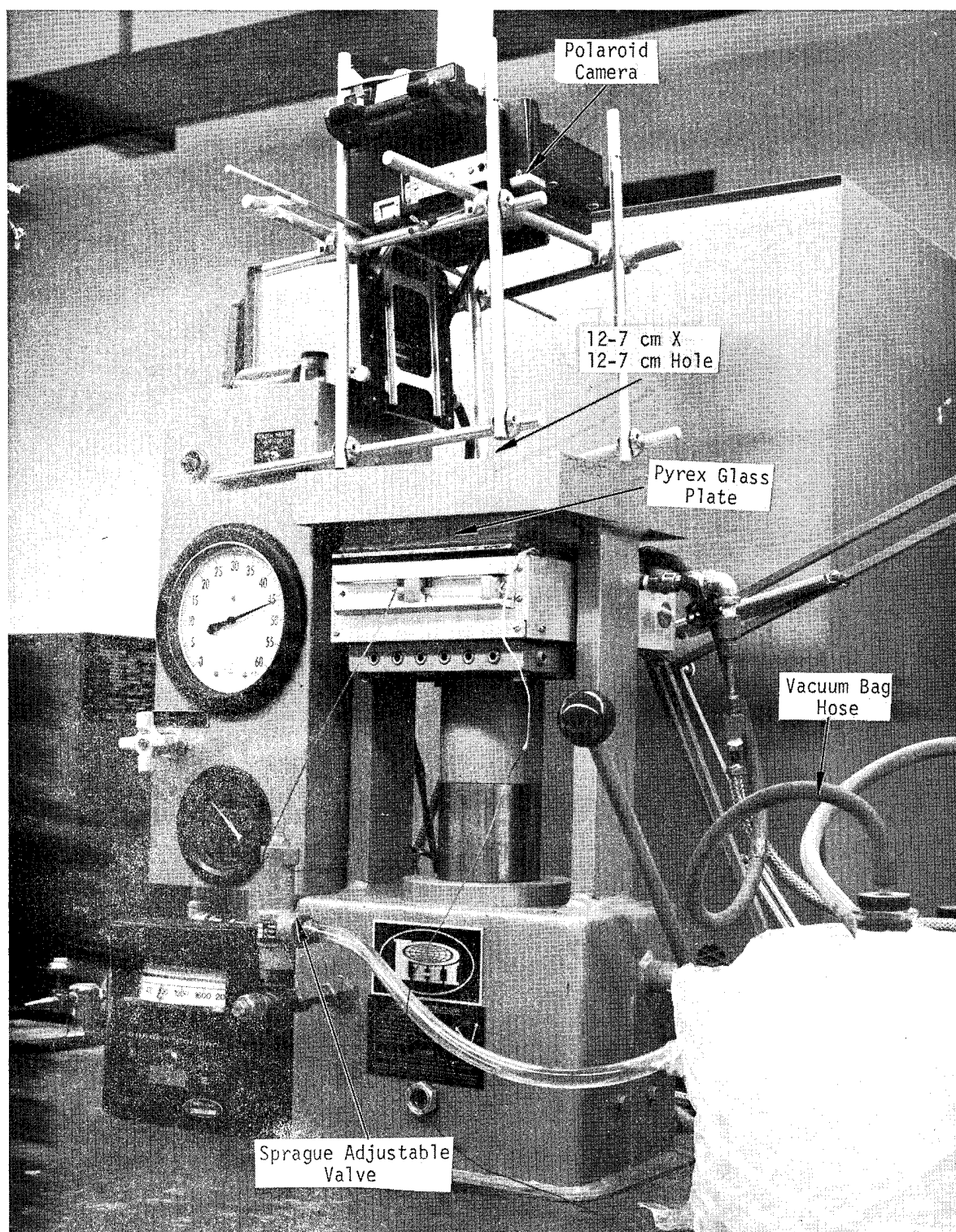
Figure 21. Resin Flow Screening Apparatus
