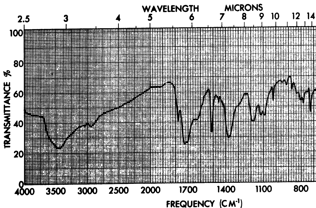
Figure C.3. Infrared Spectrum of P10P Cured in the Absence of \text{SnCl}_4 for 1.0 Hour (KBr) Concentration: 3.3 mg/g KBr
