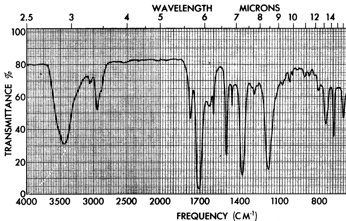
Figure B.3. Infrared Spectrum of Pyrolysis Residue I-561-2-P-C (KBr) Concentration: 3.3 mg/g KBr
