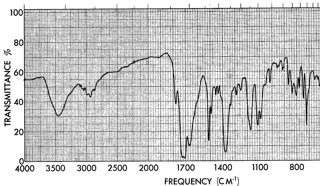
Figure 26. Infrared Spectrum of 1000 FMW NA/80MDA:20TDA/PMDA Resin Removed from One Quarter Clear Glass Prepreg Heated to 366^{\circ}\text{K} (KBr) Concentration: 4.1 mg/g KBr
