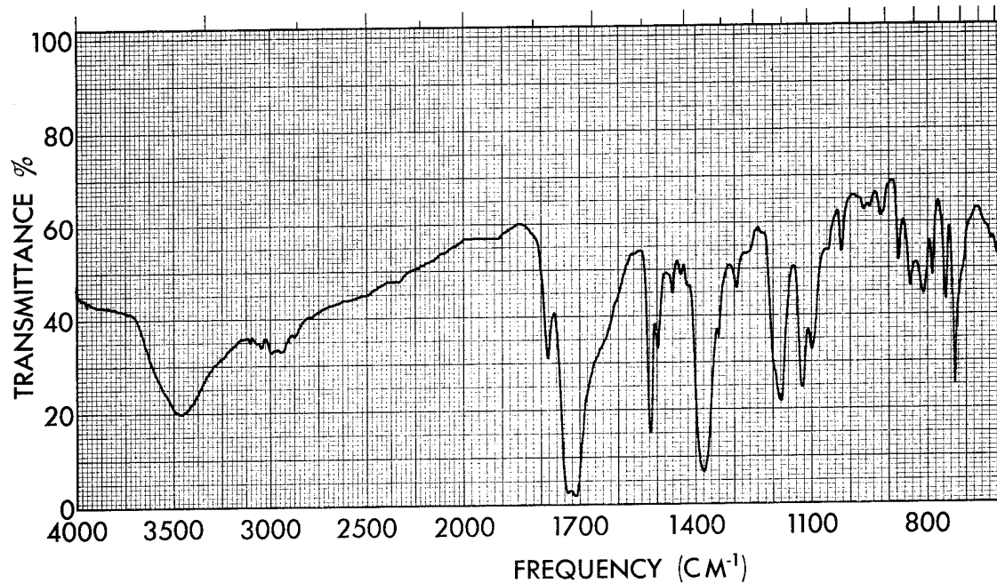
Figure 28. Infrared Spectrum of 1000 FMW NA/80MDA:20TDA/PMDA Resin Removed from Totally Clear Glass Prepreg Heated to 478°K (KBr) Concentration: 3.3 mg/g KBr
