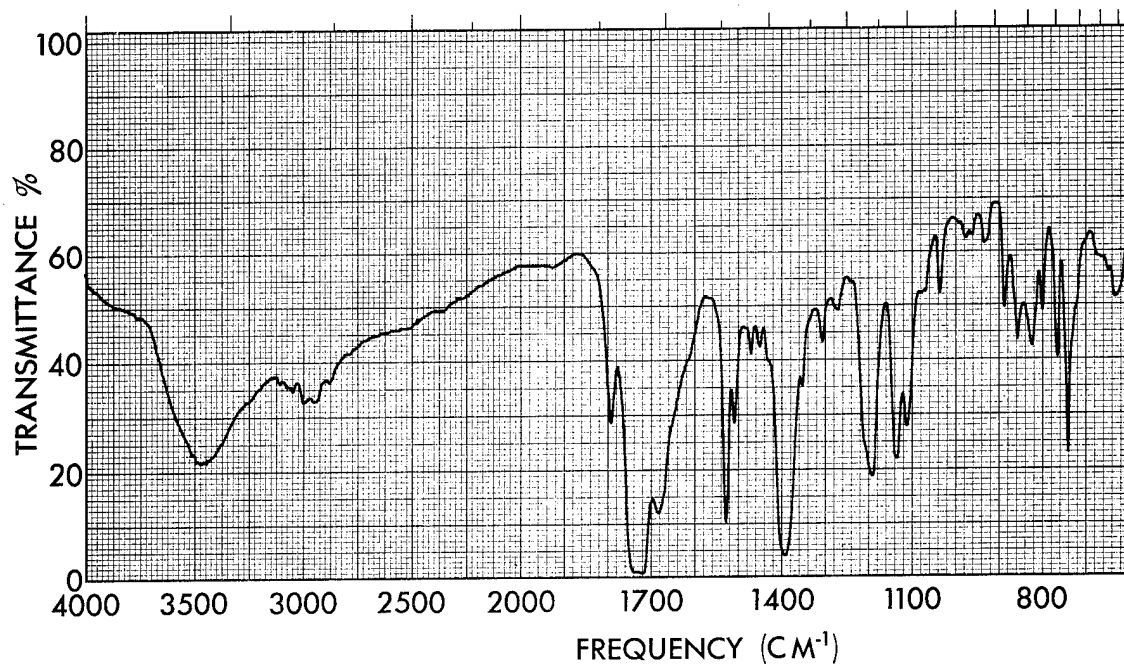
Figure 27. Infrared Spectrum of 1000 FMW NA/80MDA:20TDA/PMDA Resin Removed from One-Half Clear Glass Prepreg Heated to 422°K (KBr) Concentration: 3.3 mg/g KBr
