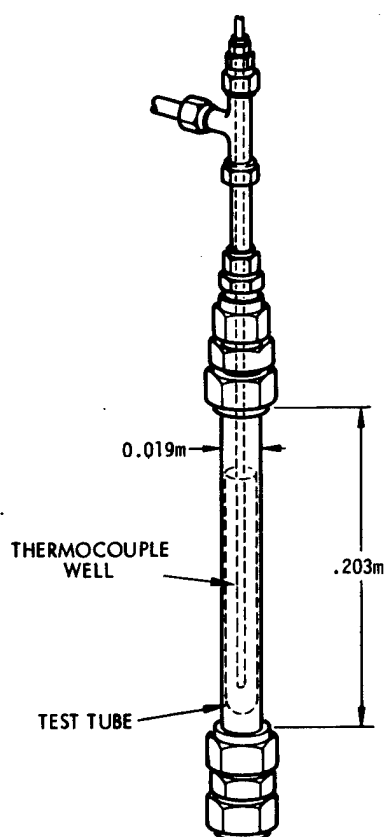
Figure 2. Pressure Chamber Used for Pyrolysis Experimentation
