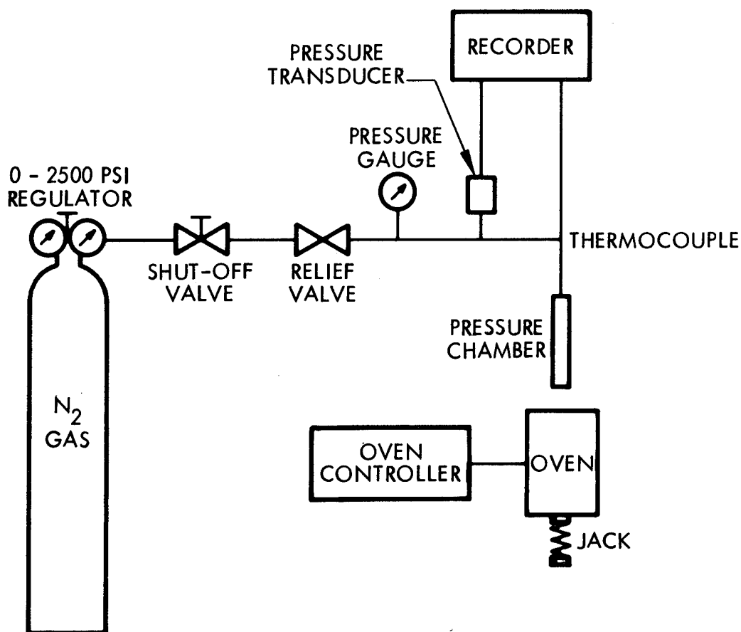
Figure 3. Schematic Pressure Pyrolysis Experimentation Set-up
