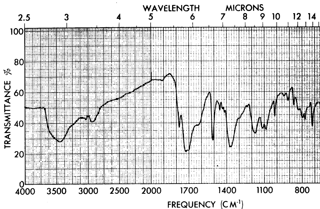
Figure C.5. Infrared Spectrum of P10P Cured in the Presence of 2.5% w/w SnCl 4 for 1.0 Hour (KBr) Concentration: 3.3 mg/g KBr
