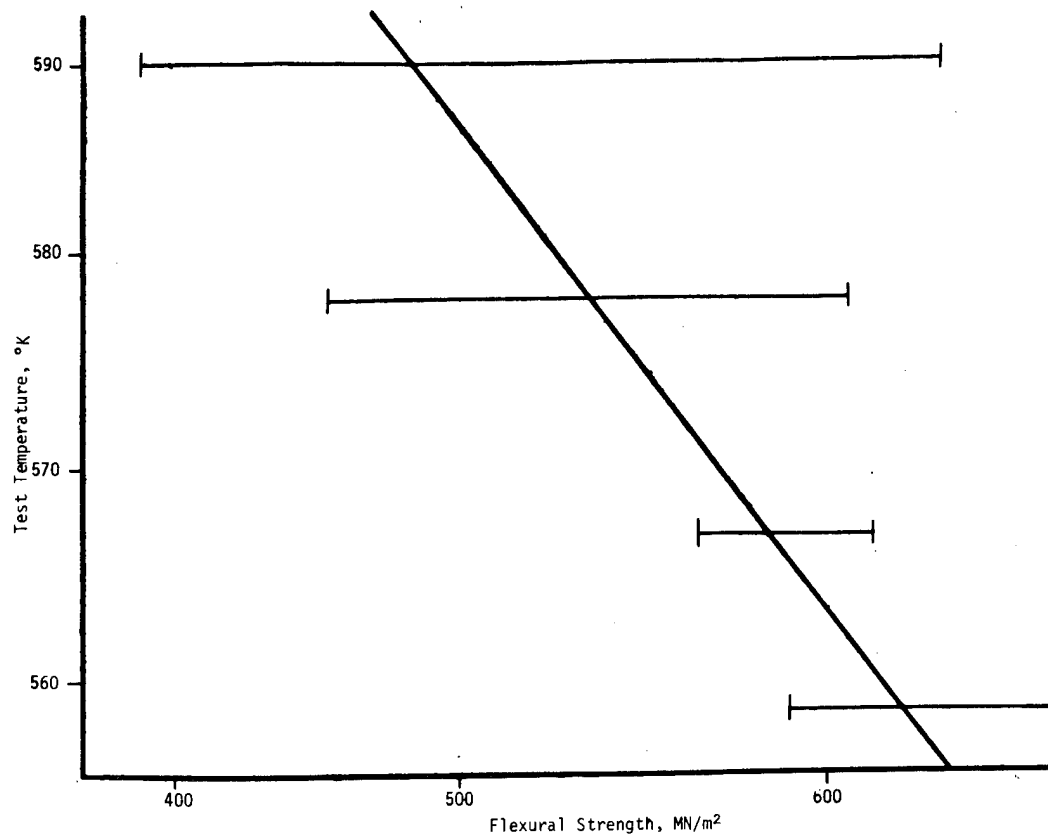
Figure 16. Flexural Strength at Elevated Temperature
