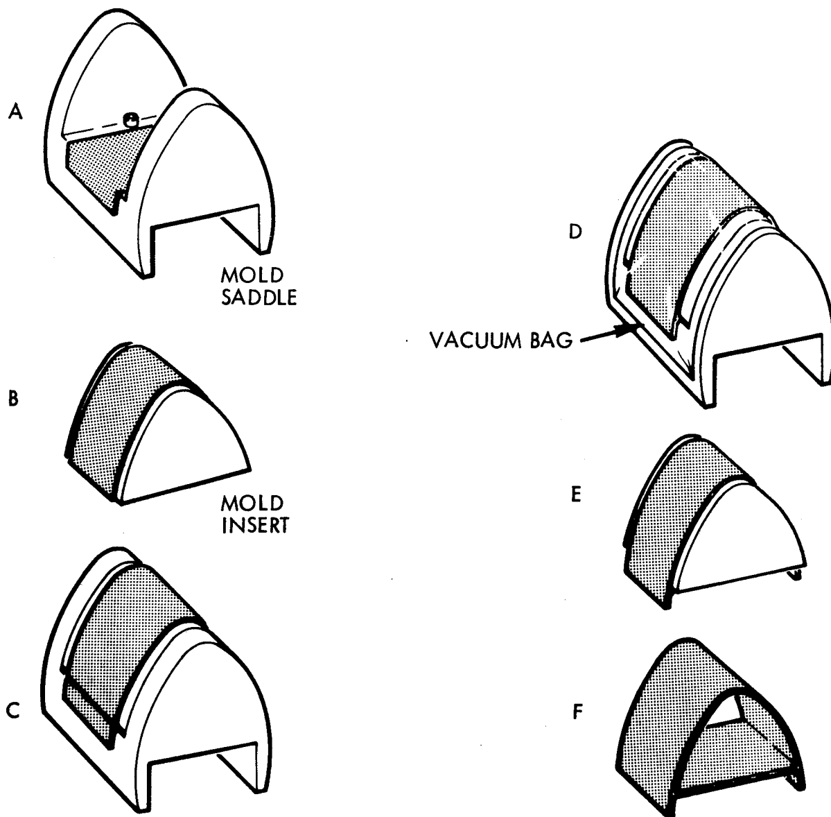
Figure 33. Fabrication Sequence
