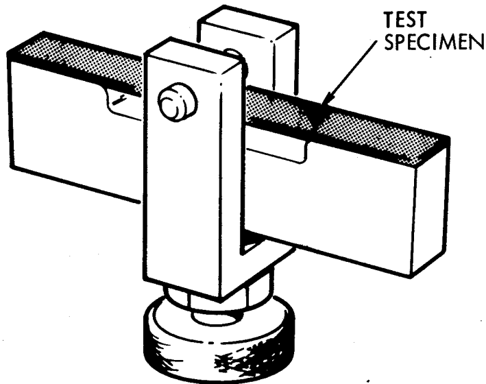
Figure 9. Restraining Jig
