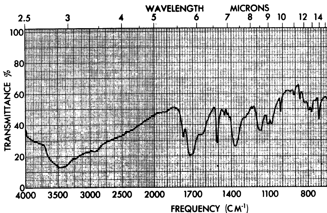
Figure C.5. Infrared Spectrum of P10P Cured in the Presence of 2.5% w/w SnCl 4 for 1.0 Hour (KBr) Concentration: 3.3 mg/g KBr
