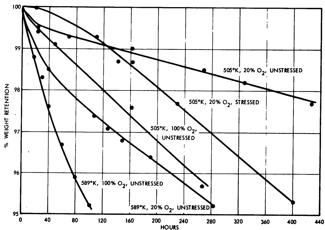
Figure 13. Weight Retention of Stressed And Unstressed Specimens
