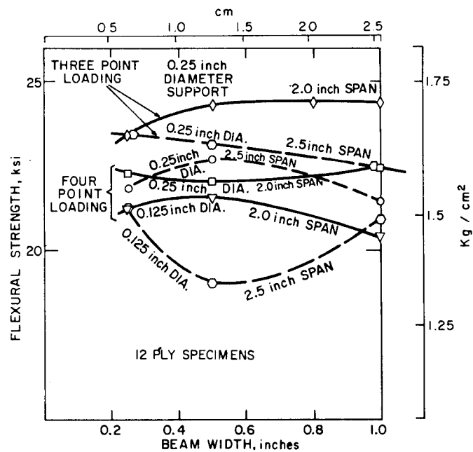
FIGURE 2-37. INFLUENCE OF BEAM WIDTH, LOAD SUPPORT DIAMETER, SPAN, AND LOADING MODE ON TRANSVERSE FLEXURAL STRENGTH OF UNIDIRECTIONAL BORON EPOXY (65)
