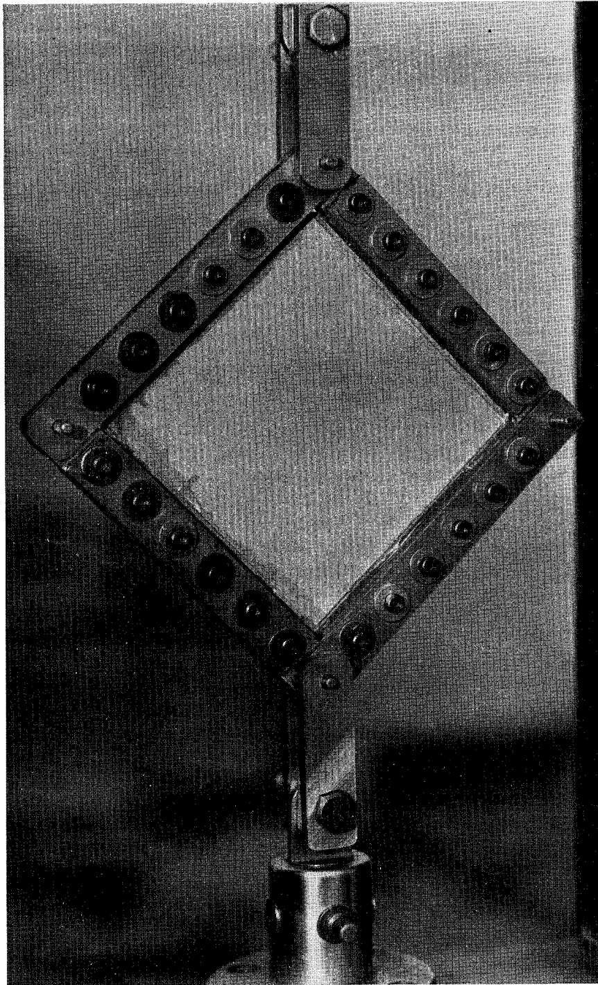
FIGURE 3-11. PICTURE FRAME FIXTURE WITH TEST ASSEMBLY
