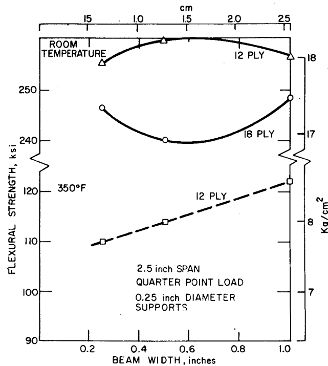
FIGURE 2-36. INFLUENCE OF BEAM WIDTH, NUMBER OF PLYS, AND TEST TEMPERATURE ON FLEXURAL STRENGTH (2.5-IN. SPAN) OF UNIDIRECTIONAL BORON EPOXY (65)
