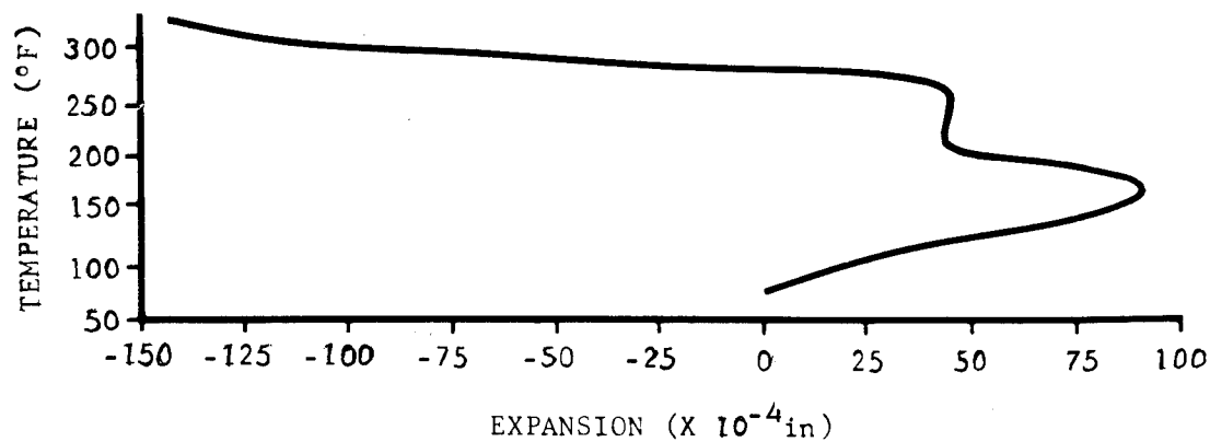
FIGURE 2-19. TYPICAL EXPANSION CURVE OF TRANSVERSE SPECIMEN OF THORNEL 50/E-798 EPOXY LAMINATE PRIOR TO POSTCURE (63)
