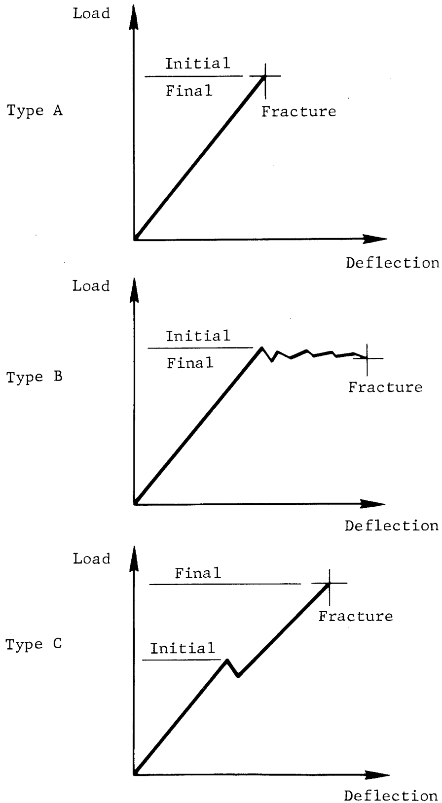
FIGURE 3-20. LOAD/DEFLECTION BEHAVIOR OF BORON/EPOXY BEARING SPECIMENS (103)
