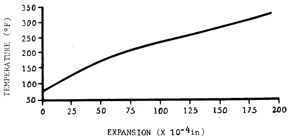
FIGURE 2-21. TYPICAL EXPANSION CURVE OF TRANSVERSE SPECIMEN OF THORNEL 50/E-798 EPOXY LAMINATE AFTER POSTCURE (63)
