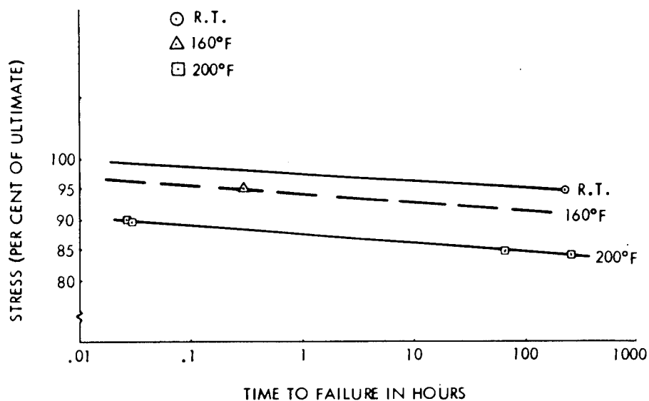
FIGURE 3-35. THE EFFECT OF STRESS LEVEL ON THE CREEP RUPTURE TIME FOR (30 DEG, -60 DEG) LAMINATES TESTED AT DIFFERENT TEMPERATURES
