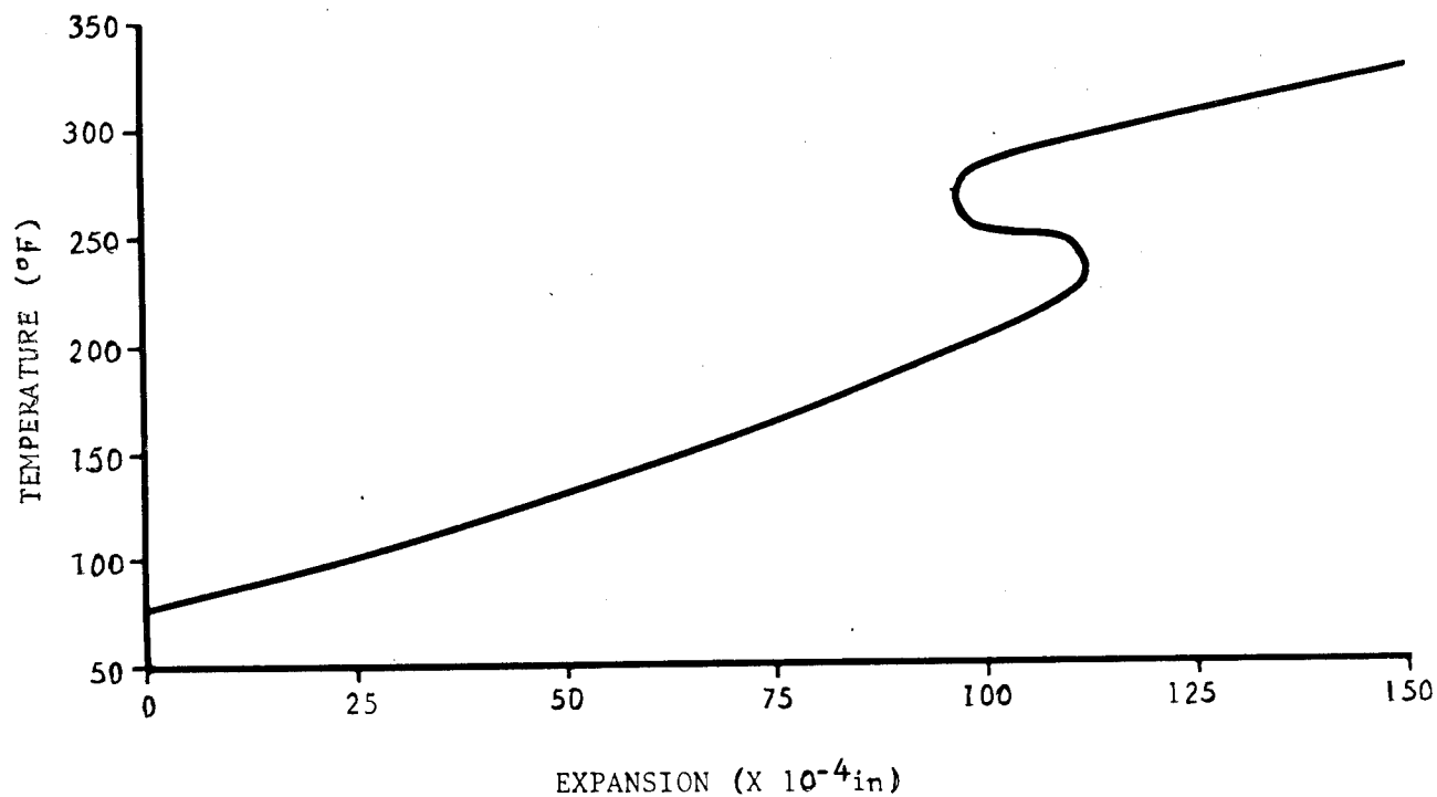
FIGURE 2-18. TYPICAL EXPANSION CURVE OF E-798 CAST RESIN PRIOR TO POSTCURE (63)
