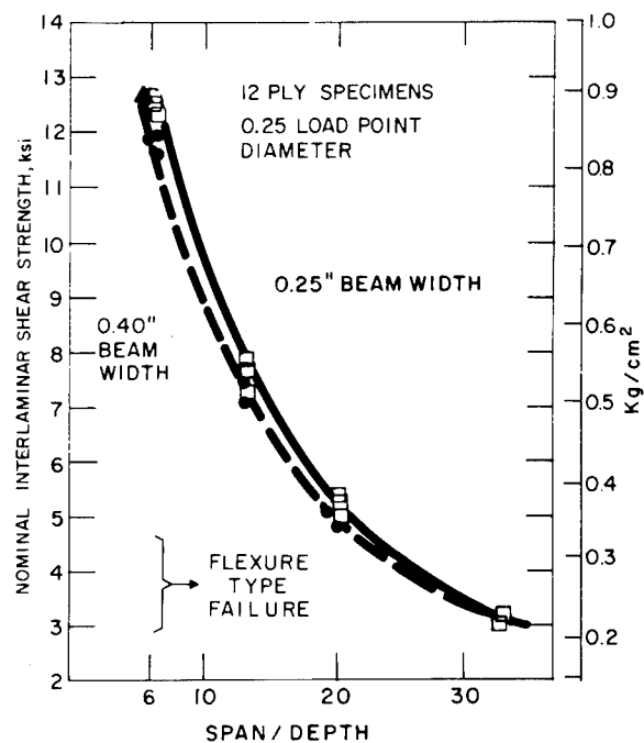
FIGURE 2-40. INFLUENCE OF SPAN TO DEPTH AND BEAM WIDTH ON NOMINAL INTERLAMINAR SHEAR STRENGTH OF UNIDIRECTIONAL BORON EPOXY (65)
