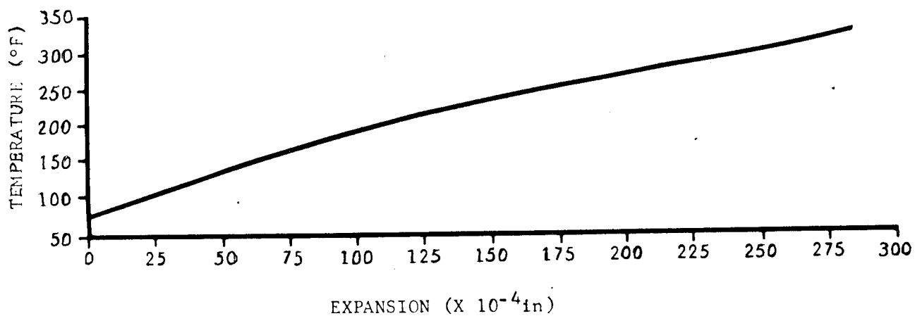
FIGURE 2-20. TYPICAL EXPANSION CURVE OF E-798 CAST RESIN AFTER POSTCURE (63)
