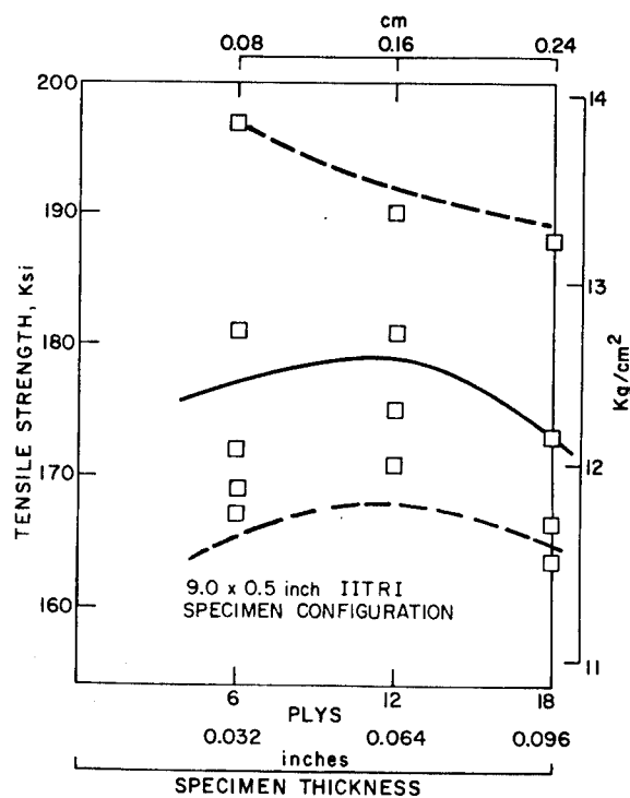
FIGURE 2-31. INFLUENCE OF PLY THICKNESS ON TENSILE STRENGTH OF UNIDIRECTIONAL BORON EPOXY (65)
