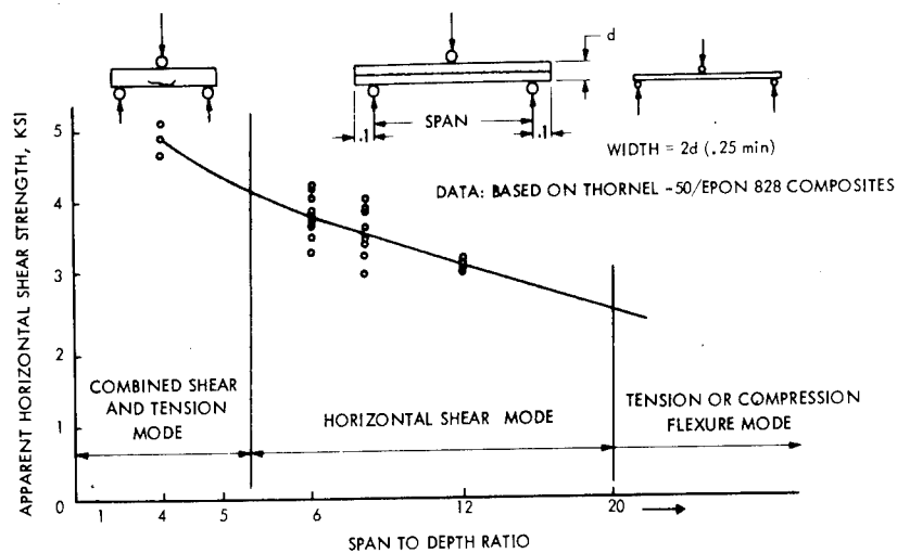
FIGURE 2-39. GENERAL CHARACTERISTICS OF INTERLAMINAR TEST FOR GRAPHITE/EPOXY COMPOSITES (66)
