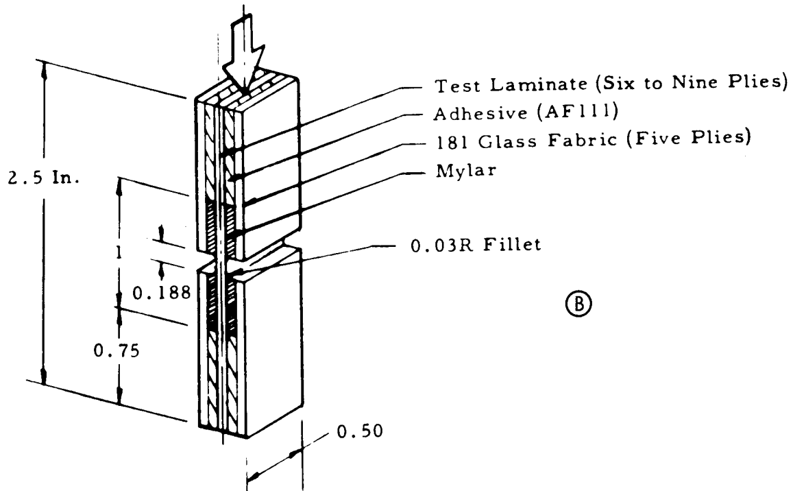
FIGURE 3-8. COMPRESSION TEST SPECIMEN TYPES (71,86)
