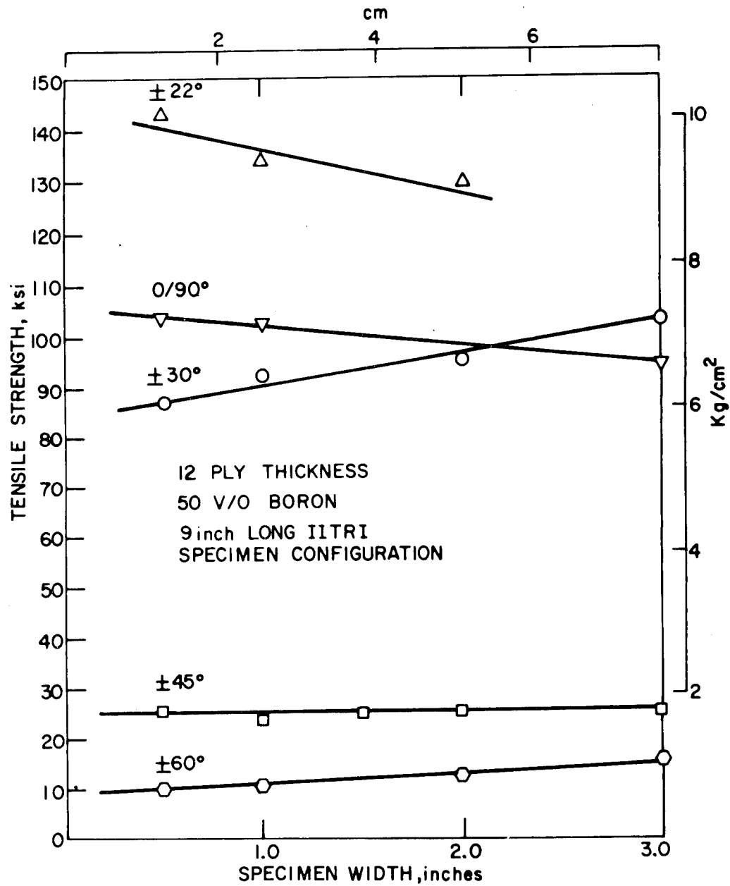
FIGURE 2-32. INFLUENCE OF SPECIMEN WIDTH ON TENSILE STRENGTH OF CROSS-PLY AND ANGLE-PLY BORON EPOXY (65)
