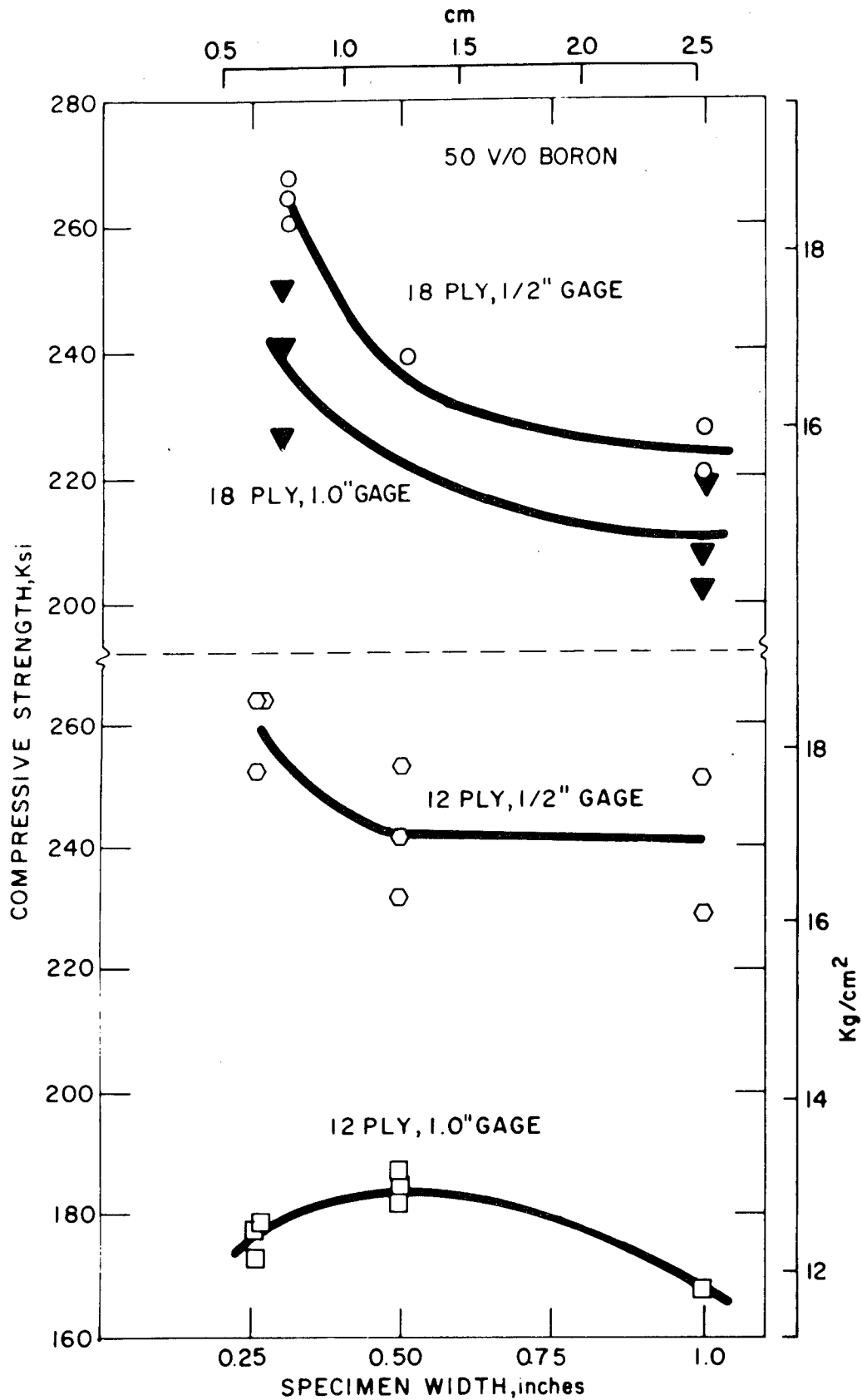
FIGURE 2-34. INFLUENCE OF SPECIMEN WIDTH, LENGTH, AND NUMBER OF PLYS ON COMPRESSIVE STRENGTH OF UNIDIRECTIONAL BORON EPOXY (65)
