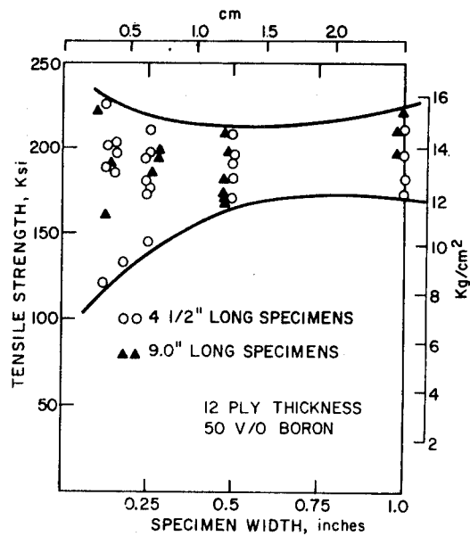
FIGURE 2-30. INFLUENCE OF SPECIMEN WIDTH AND LENGTH ON TENSILE STRENGTH OF UNIDIRECTIONAL BORON EPOXY (65)
