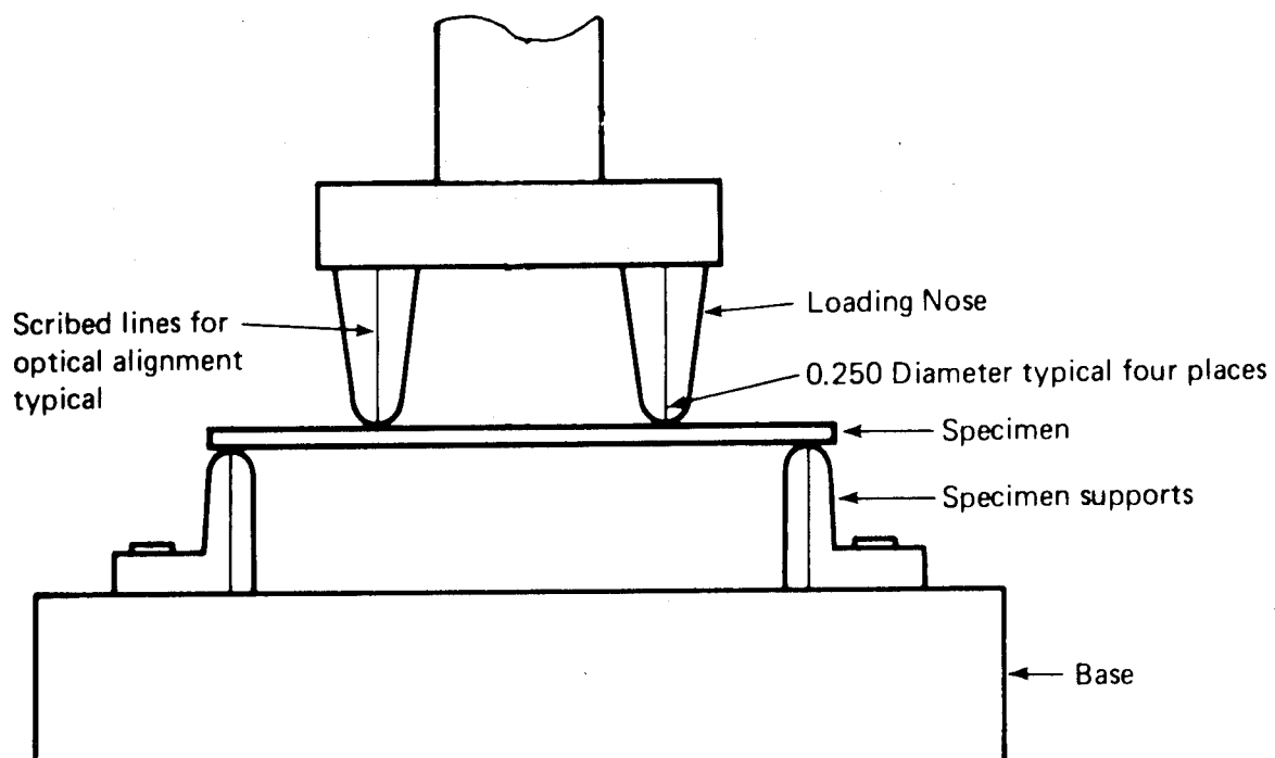
FIGURE 2-15. FLEXURE TEST FIXTURE (46)
