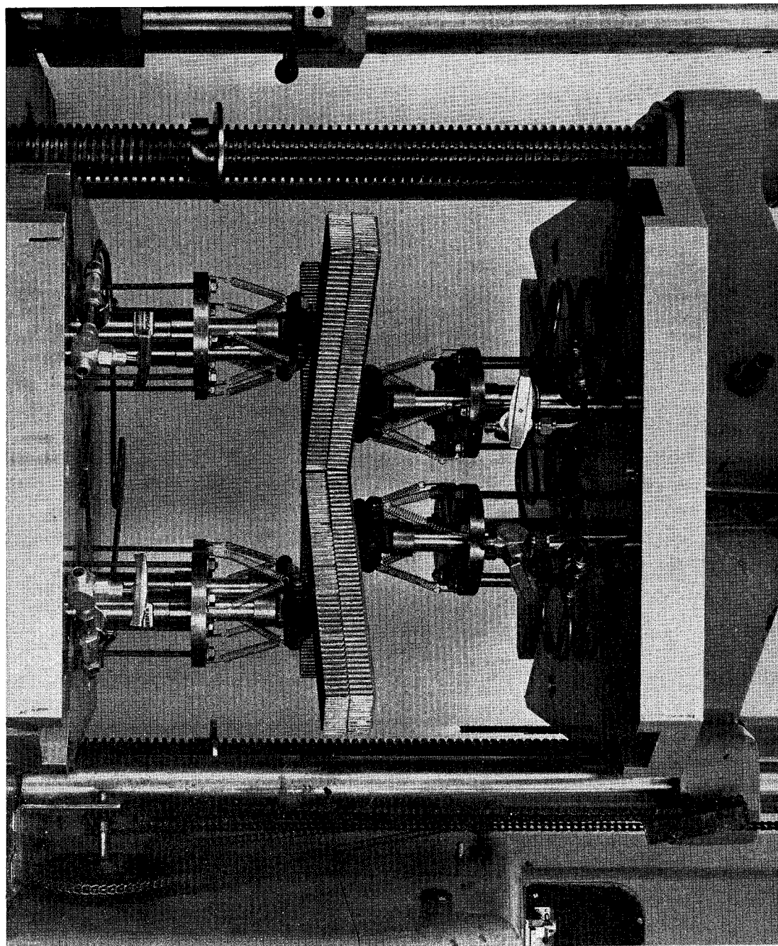
FIGURE 3-6. HYDRAULIC CUSHIONED BIAXIAL CROSSBEAM STRESS FIXTURE (64)
