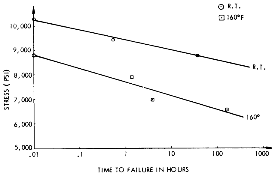
FIGURE 3-36. THE EFFECT OF STRESS LEVEL ON THE CREEP RUPTURE TIME FOR (45 DEG, -45 DEG) LAMINATES TESTED AT DIFFERENT TEMPERATURES
