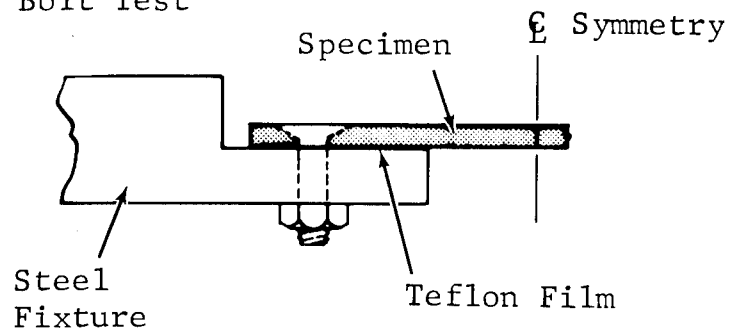
Countersunk Bolt Test
