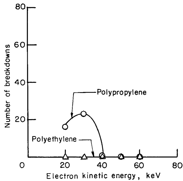
Figure 11.- Dependence of breakdown frequency on kinetic energy for polyethylene and polypropylene. Electron fluence for each data point = 2 \times 10^{13} \text{ e/cm}^2 . T = 298°.
