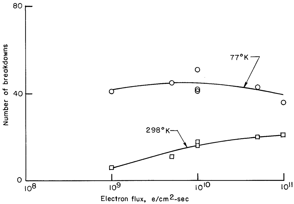
Figure 15.- Dependence of breakdown frequency on flux for Pyrrone. Electron fluence for each data point = 1 \times 10^{13} e/cm 2 ; E_k = 30 keV.
