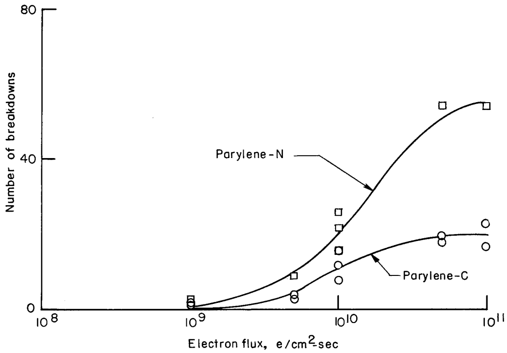
Figure 14.- Dependence of breakdown frequency on flux for parylene-C and parylene-N. Electron fluence for each data point = 1 \times 10^{13} e/cm 2 ; E_k = 30 keV; T = 298^\circ K.
