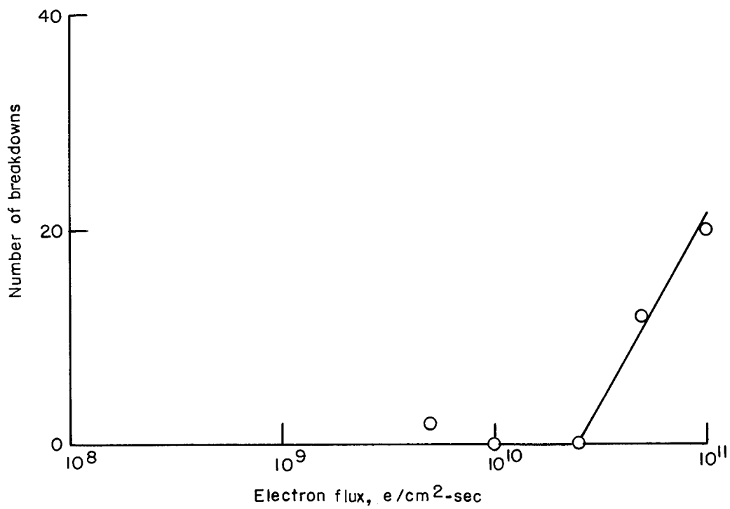
Figure 17.- Dependence of breakdown frequency on flux for polyethylene. Electron fluence for each data point = 2 \times 10^{13} e/cm 2 ; E_k = 30 keV; T = 2980 K.
