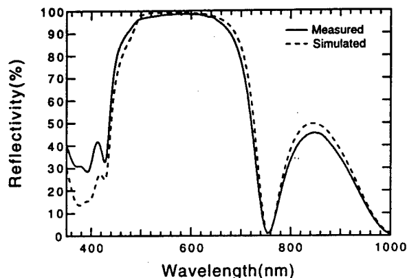
Fig. 2. Reflectance spectra for the 4.5-pair \text{Al}_{0.5}\text{In}_{0.5}\text{P} -oxide DBR.
