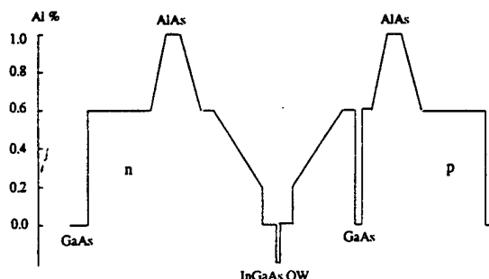
Fig. 1. The schematic of the conduction band of laser structure with AlAs layers above and below the waveguide region for oxidation.
